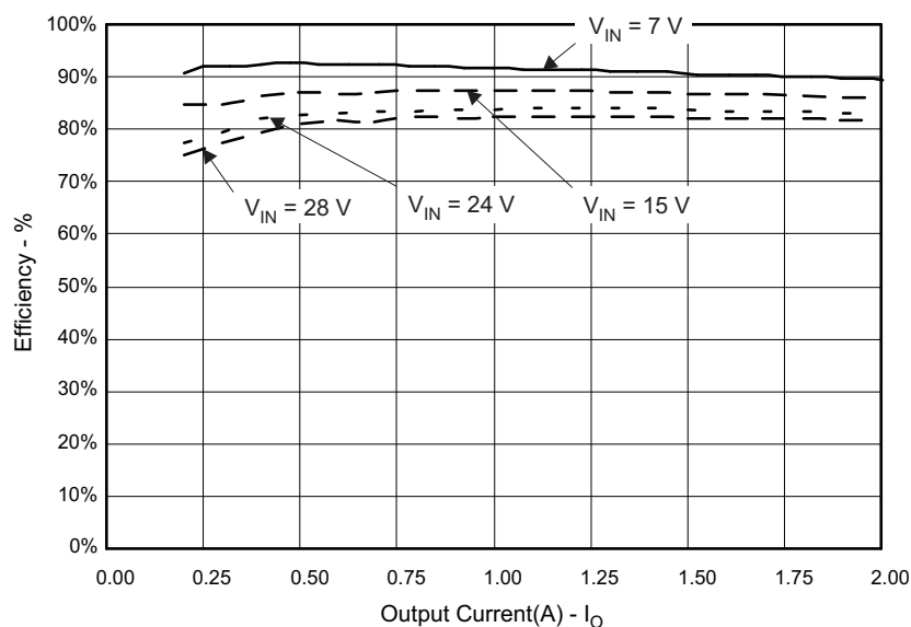
Figure 1. TPS54231EVM-372 Efficiency
