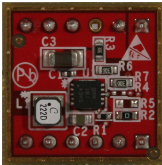
Figure 1. SMP-TPS61200-MVK Submodule
