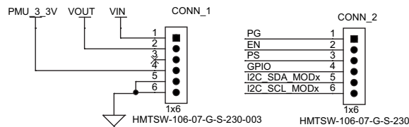
SUB-MODULE CONNECTORS
