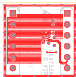
Figure 13. SMP-TPS7A1633-MVK Board Layer 4 – Bottom Side
