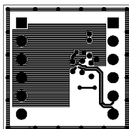
Figure 7. SMP-TPS7A1633-MVK Board Layer 4 – Bottom Side
