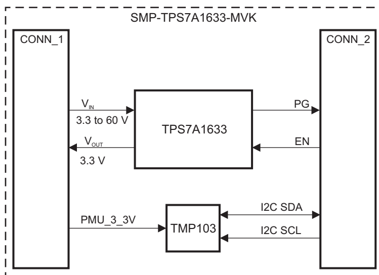
Figure 2. SMP-TPS7A1633-MVK Block Diagram
