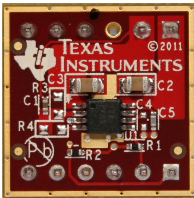
Figure 1. SMP-TPS7A1633-MVK MAVRK Submodule
