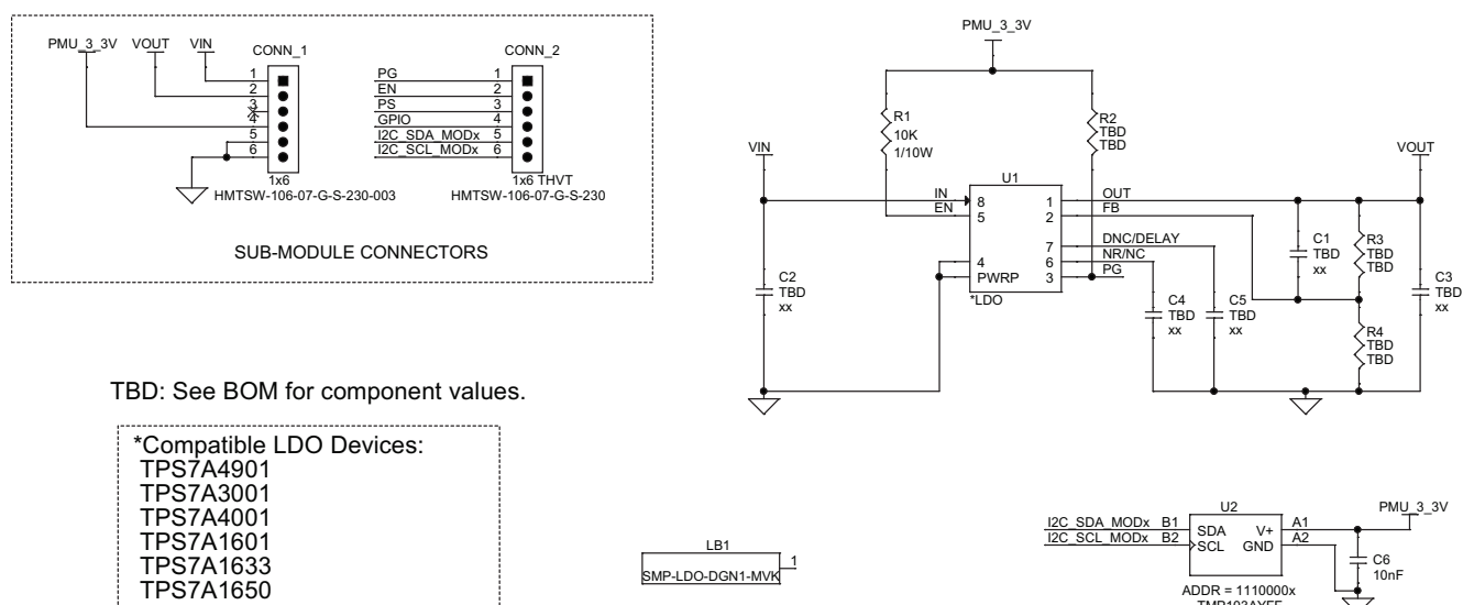
Figure 14. SMP-TPS7A1633-MVK Schematic
