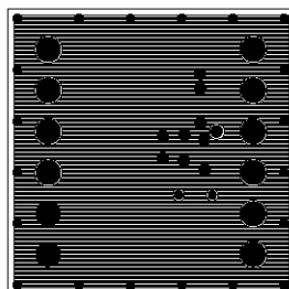
Figure 5. SMP-TPS7A1633-MVK Board Layer 2 – Ground Plane
