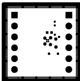
Figure 9. SMP-TPS7A1633-MVK Board Solder Mask – Bottom Side
