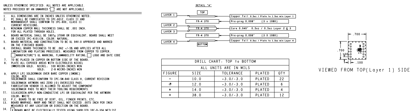
Figure 15. SMP-TPS7A1633-MVK Fabrication Drawing
