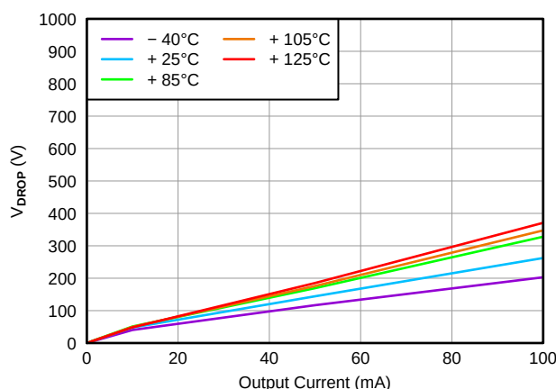
Figure 3. TPS7A1633 Dropout Voltage Versus Output Current
