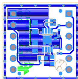
Figure 12. SMP-TPS7A1633-MVK Board Layer 1 – Top Side
