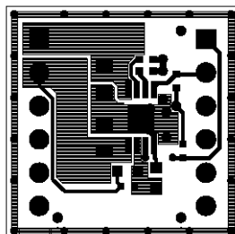
Figure 4. SMP-TPS7A1633-MVK Board Layer 1 – Top Side
