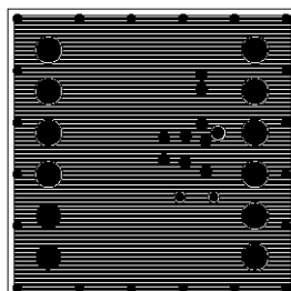
Figure 6. SMP-TPS7A1633-MVK Board Layer 3 – Ground Plane
