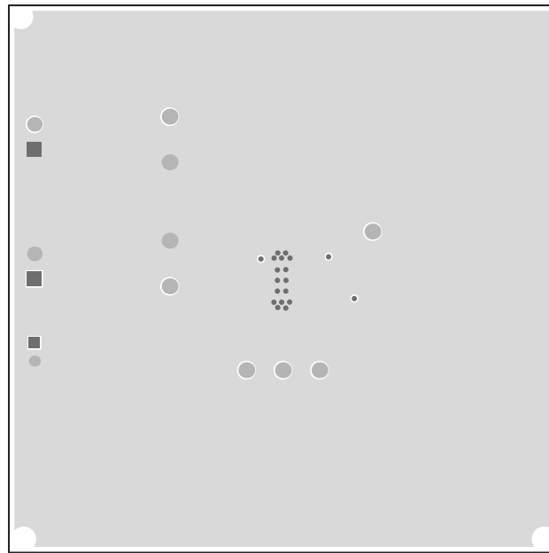
Figure 18. Internal Layer 2
