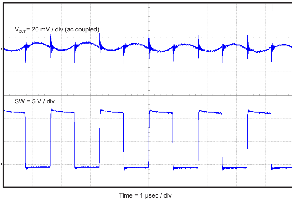
Figure 7. TPS54531EVM-530 Output Voltage Ripple ( I_{OUT} = 5 \text{ A} )
