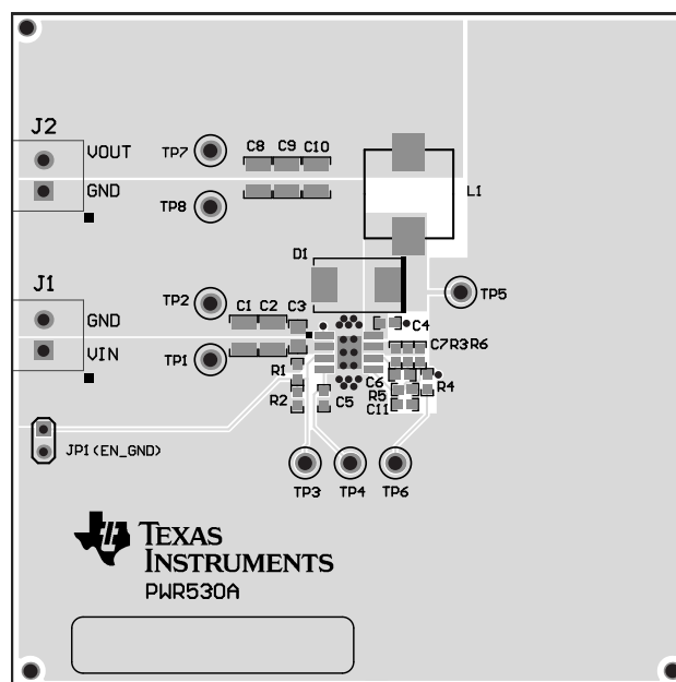
Figure 15. Top Assembly
