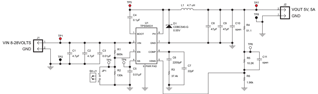
Figure 20. TPS54531EVM-530 Schematic Diagram
