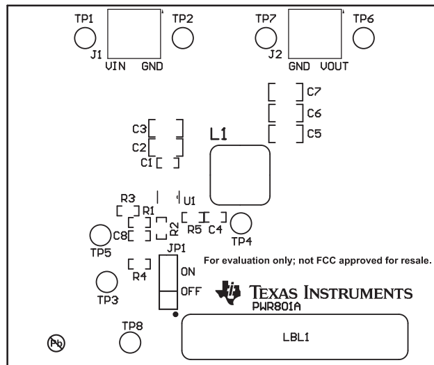
Figure 14. Top Assembly
