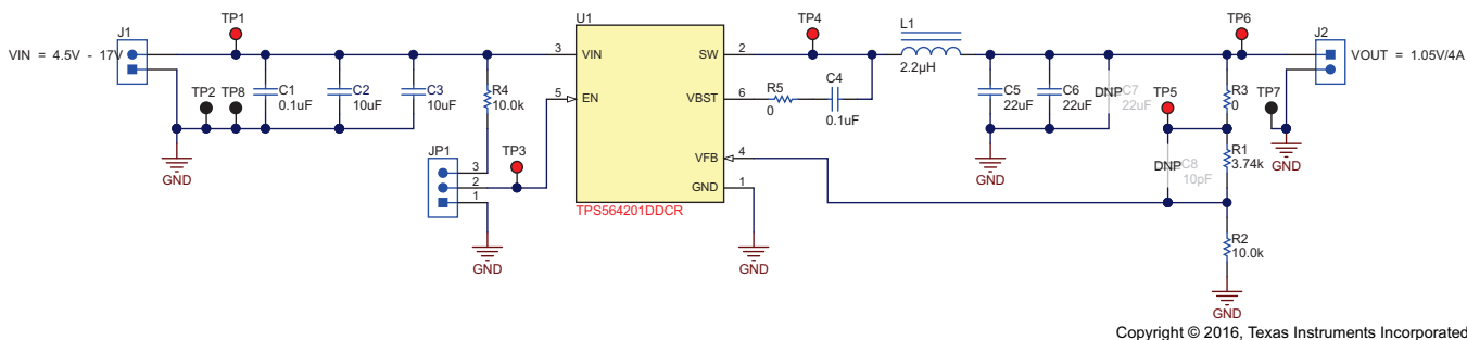
Figure 17. TPS564201EVM-801 Schematic Diagram
