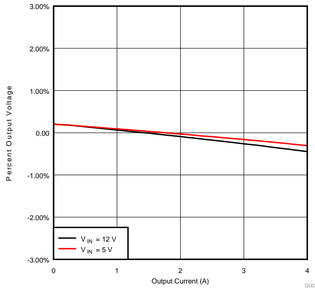
Figure 3. Load Regulation
