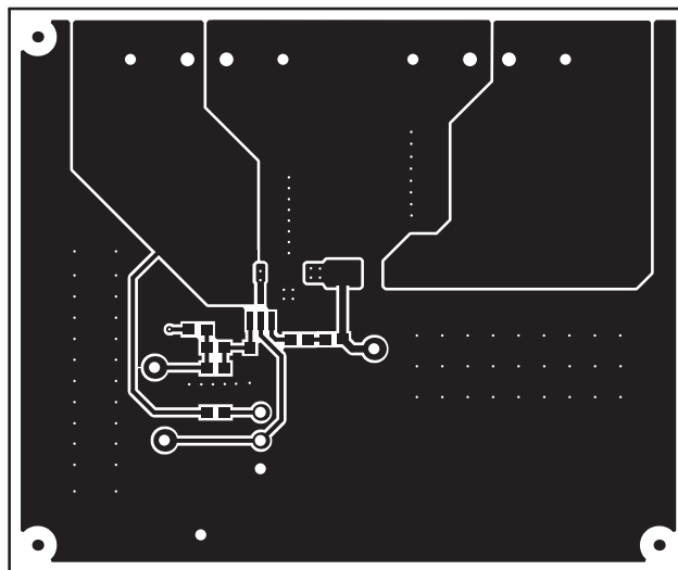
Figure 15. Top Layer
