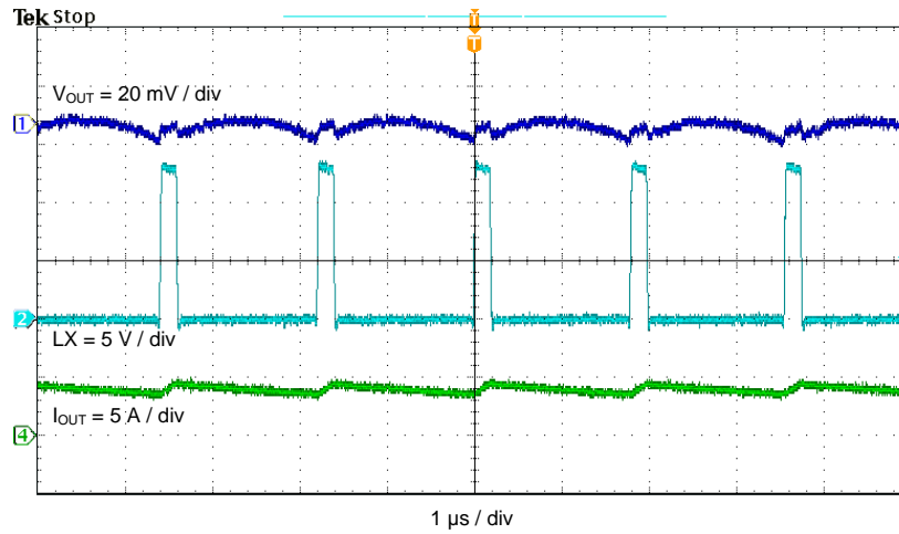
Figure 6. Output Voltage Ripple, I_{OUT} = 4 \text{ A}
