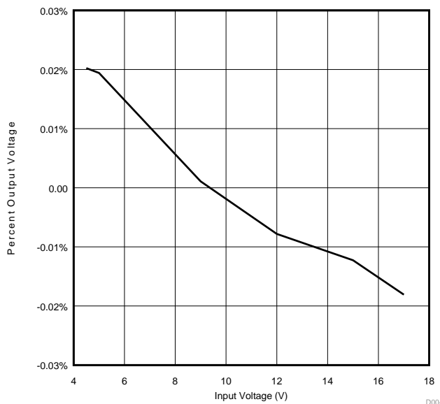
Figure 4. Line Regulation
