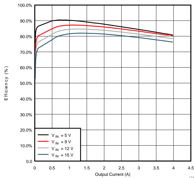
Figure 1. Efficiency
