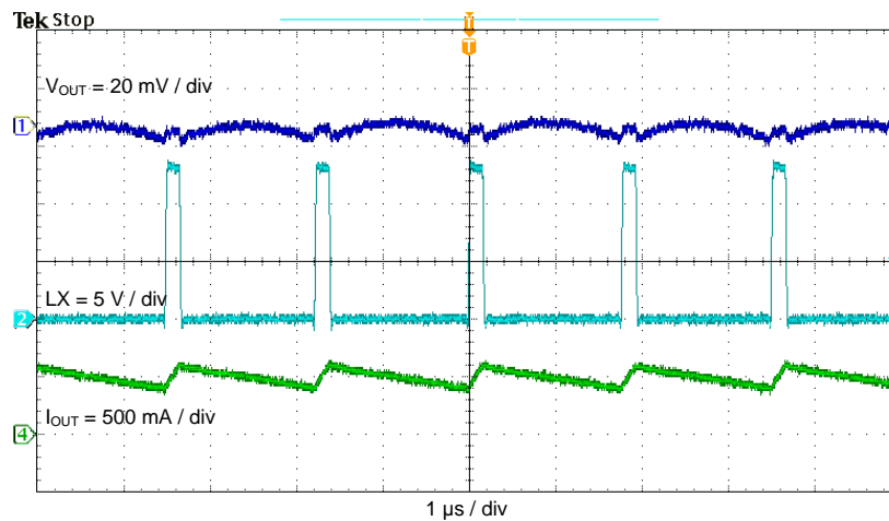
Figure 7. Output Voltage Ripple, I_{OUT} = 2 \text{ A}
