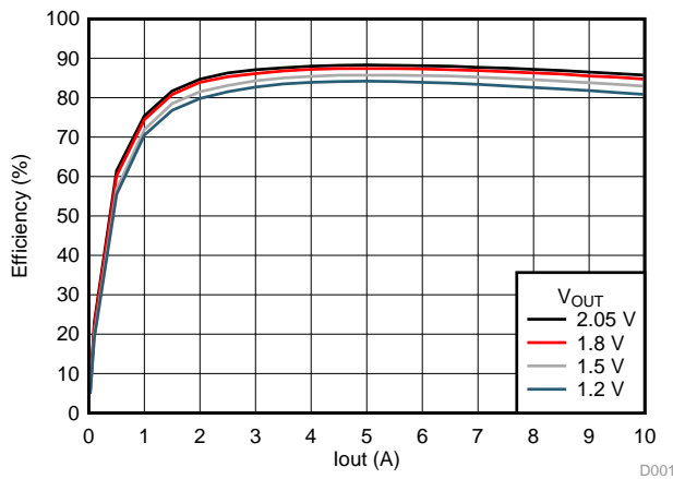
Figure 2. TPSM84A22EVM Efficiency (VG = OPEN)
