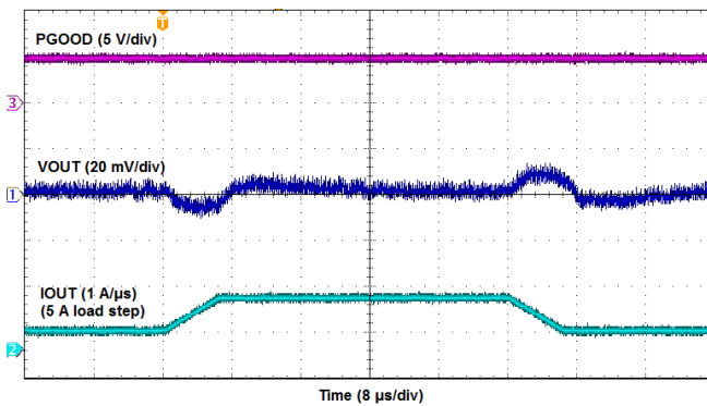
Figure 6. Output Current Transient Waveforms
