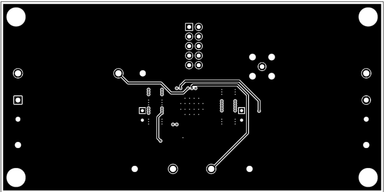
Figure 12. Layer 2 Copper
