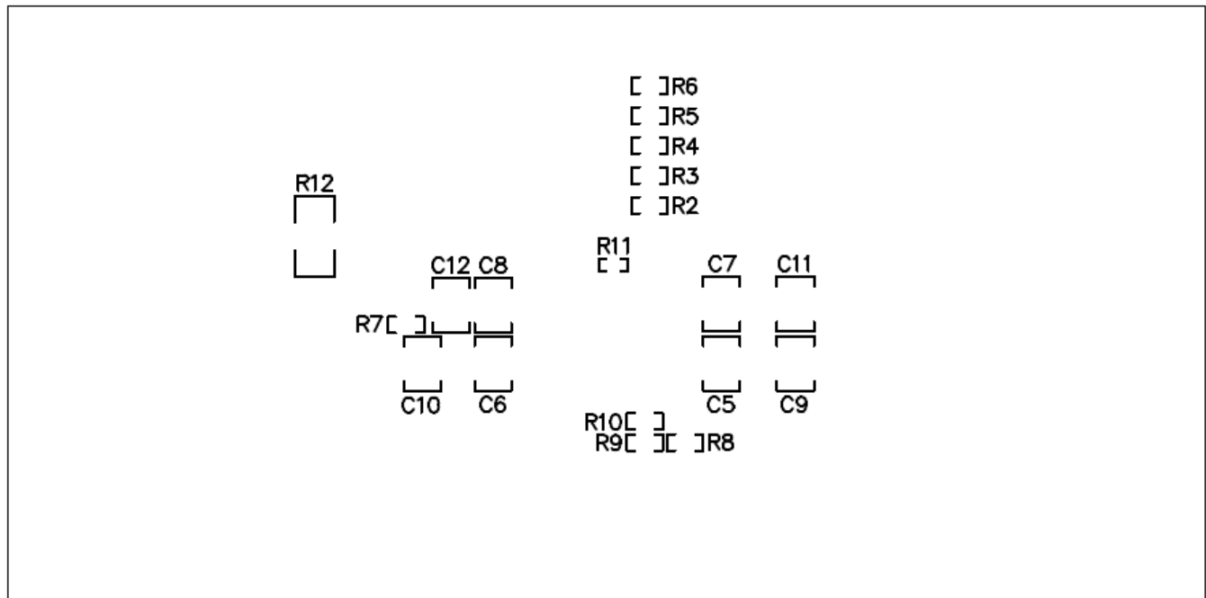
Figure 10. Bottom-Side Component Layout
