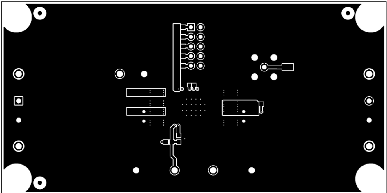
Figure 14. Bottom Copper
