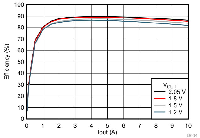
Figure 3. TPSM84A22EVM Efficiency (VG = 5V)
