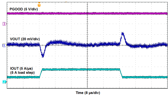
Figure 7. Output Current Transient Waveforms
