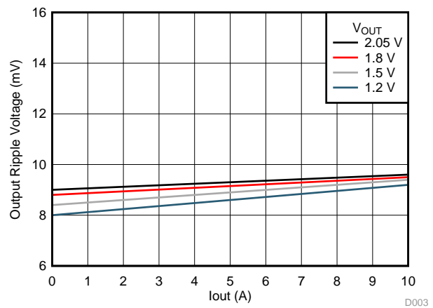
Figure 5. TPSM84A22EVM Output Voltage Ripple
