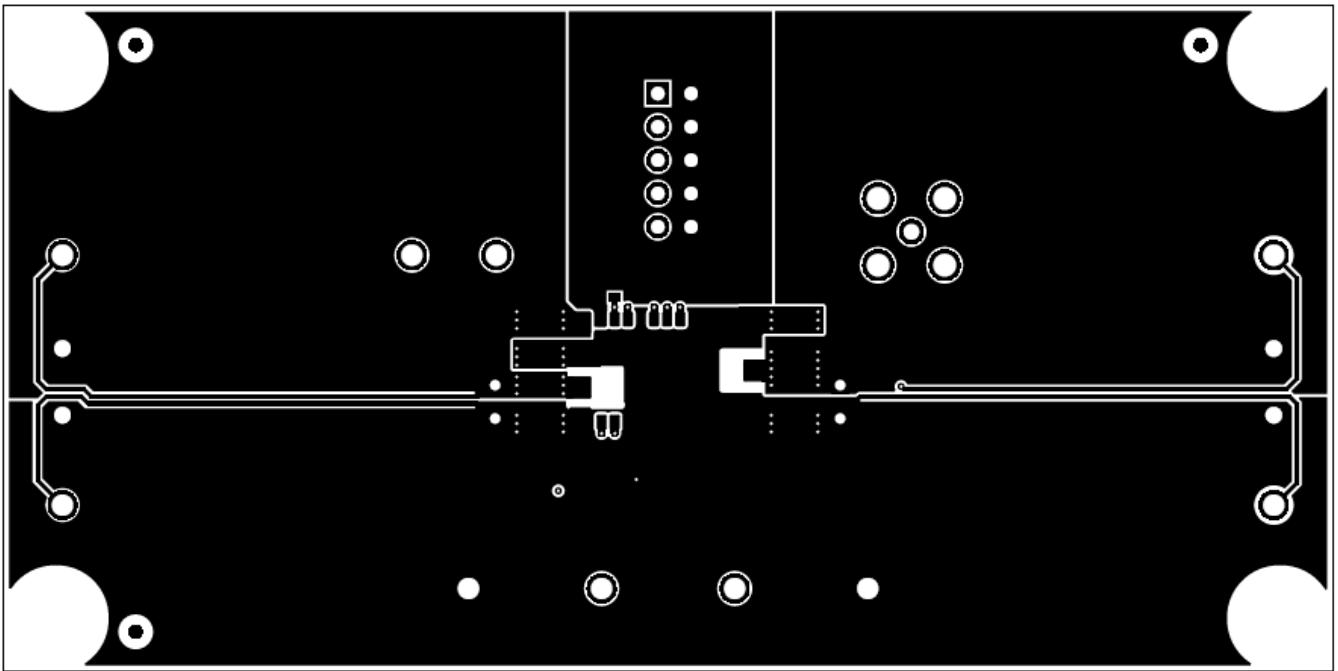
Figure 11. Top Copper
