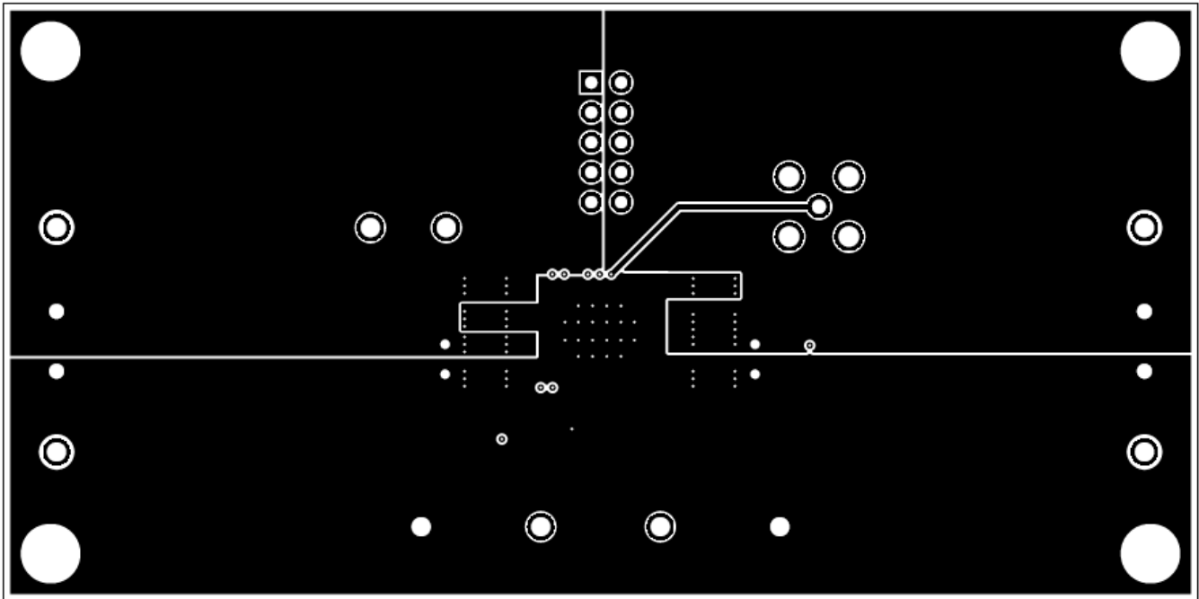
Figure 13. Layer 3 Copper
