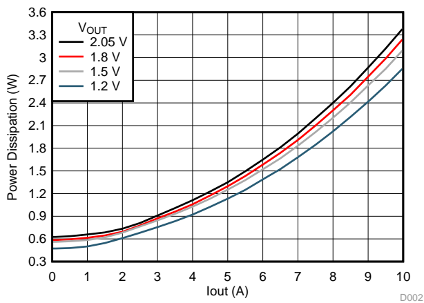
Figure 4. TPSM84A22EVM Power Dissipation
