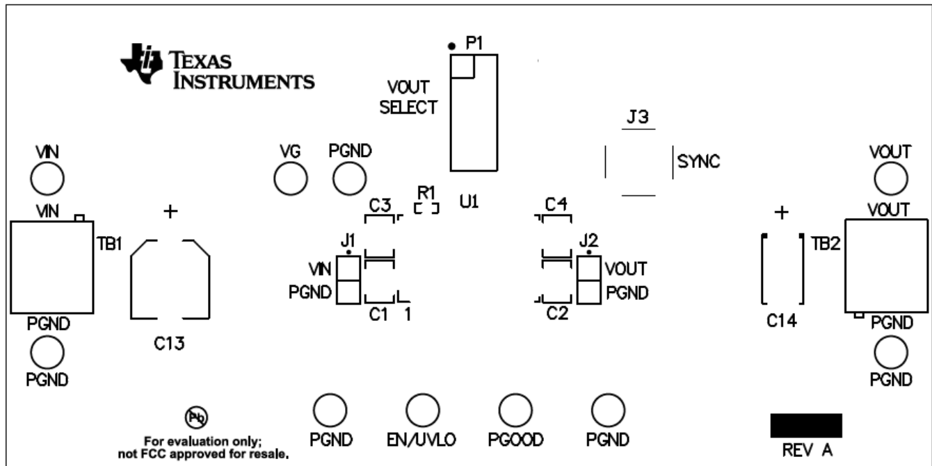
Figure 9. Topside Component Layout
