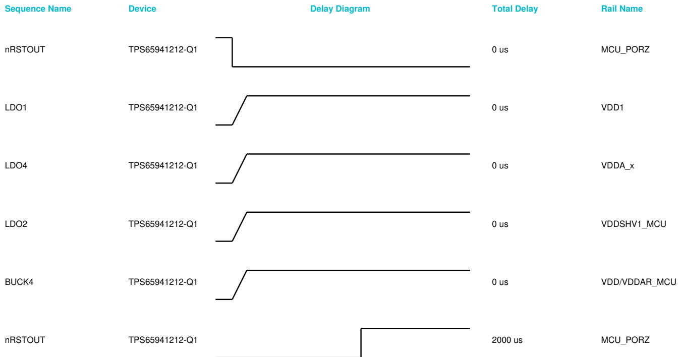
Figure 6-8. MCU_TO_WARM Sequence
