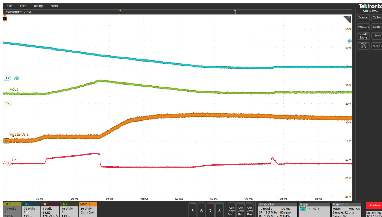
Figure 5-4. Overvoltage Response with 37-V OV-Cutoff Point
