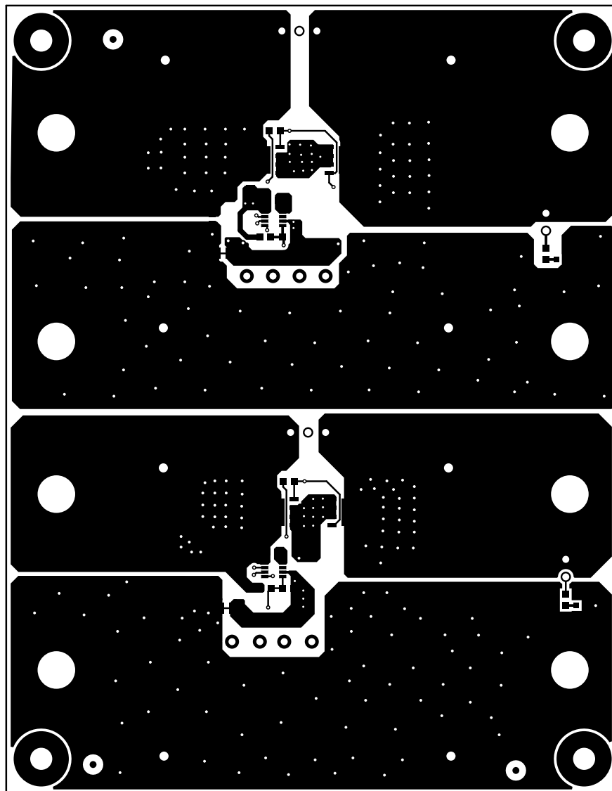
Figure 6-3. Top Layer Routing
