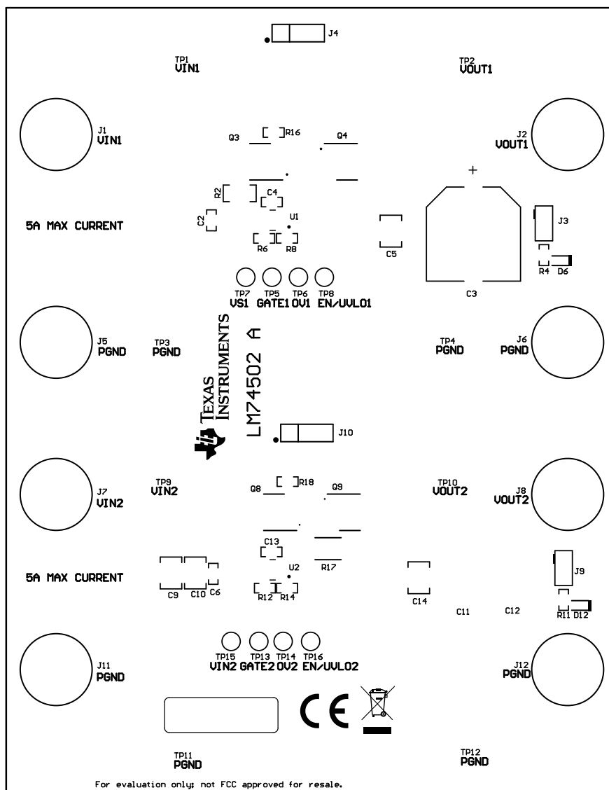
Figure 6-1. Top Layer Placement
