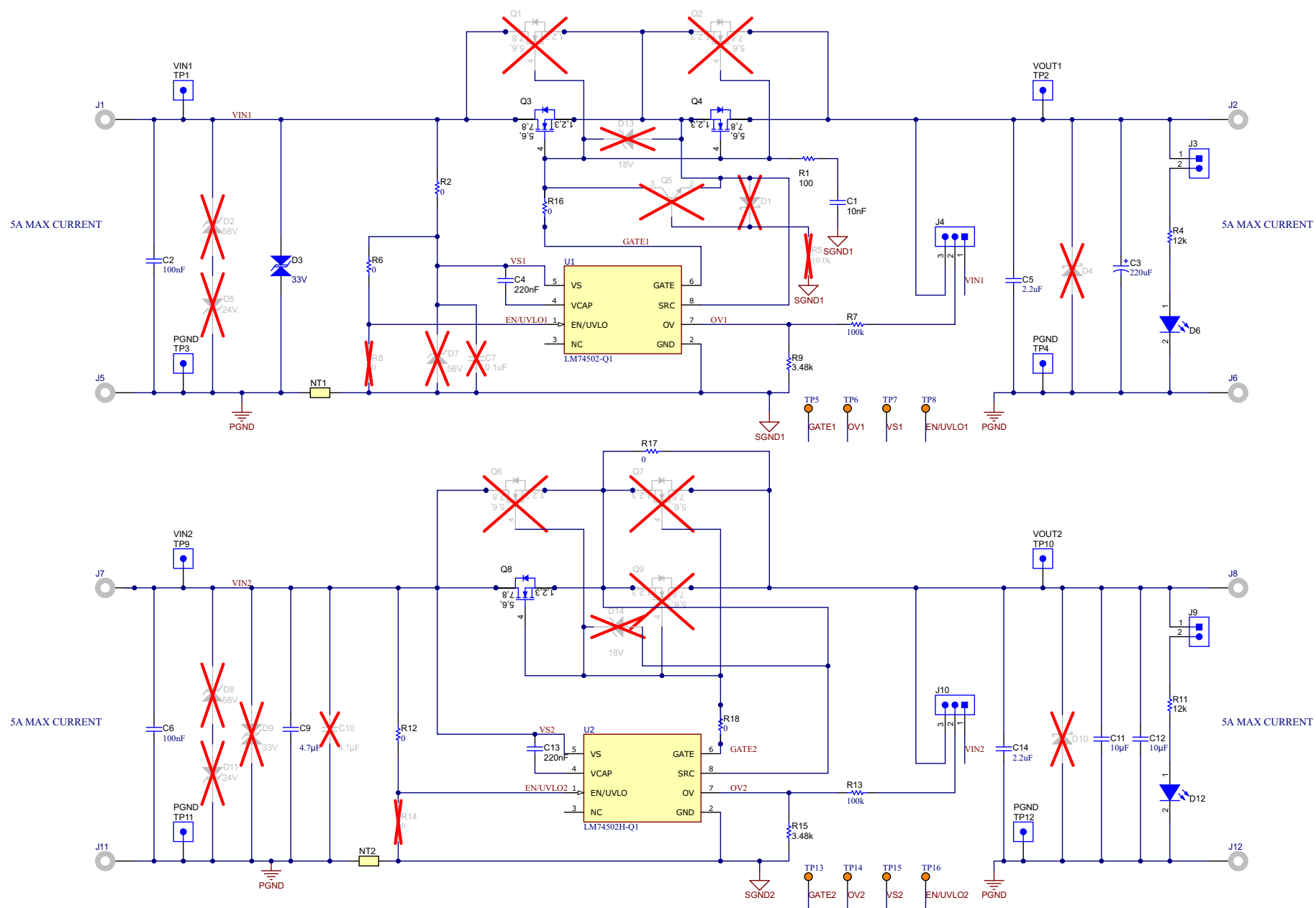
Figure 3-1. LM74502Q1EVM Schematic
