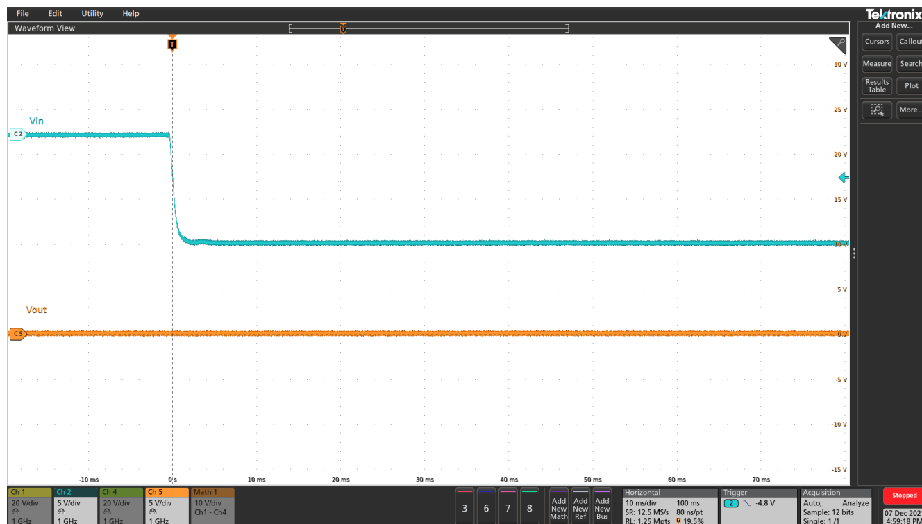
Figure 5-5. Reverse Input Response
