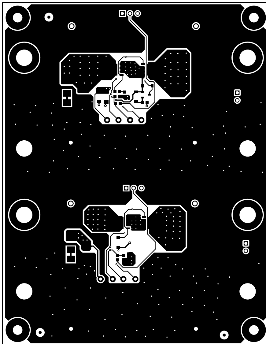
Figure 6-4. Bottom Layer Routing
