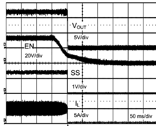
Figure 14. Shut Down at 48V IN
