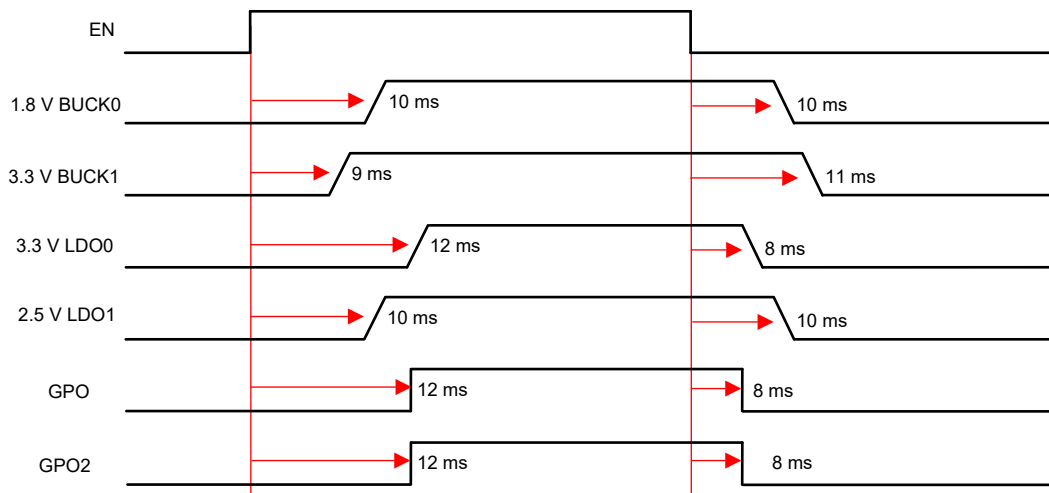
Figure 3-1. LP87334A-Q1 Power-up and Power Down Sequence
