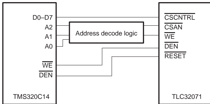
Figure 4–10. TMS320C14 to TLC32071 Interface
