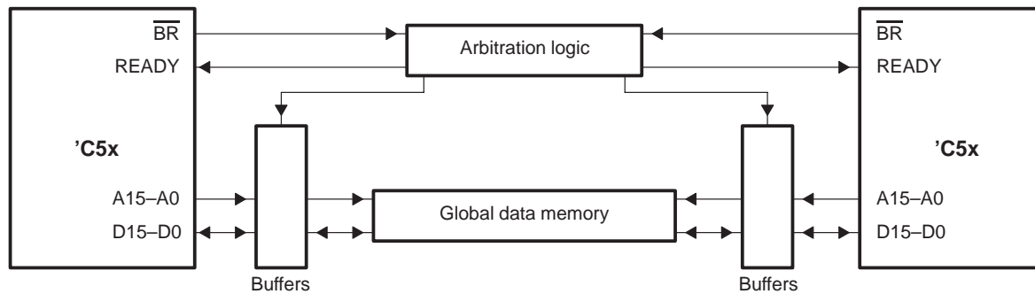
Figure 3–3. Global Memory Interface
