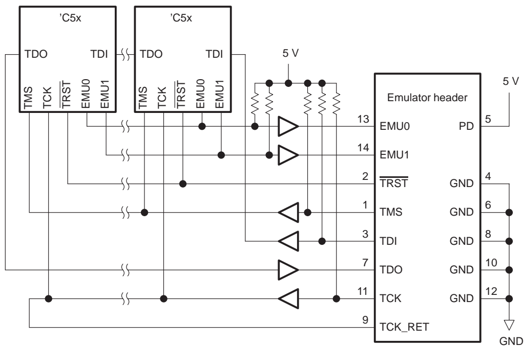
Figure A–5. Multiprocessor Connections
