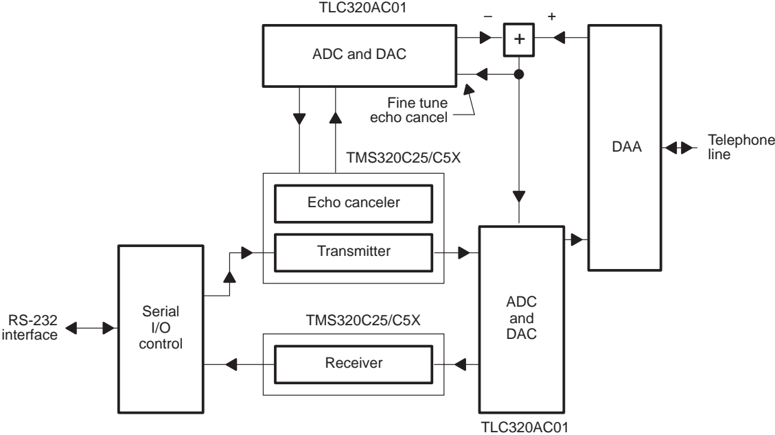
Figure 4-11. High-Speed V.32bis and Multistandard Modem With the TLC320AC01 AIC
