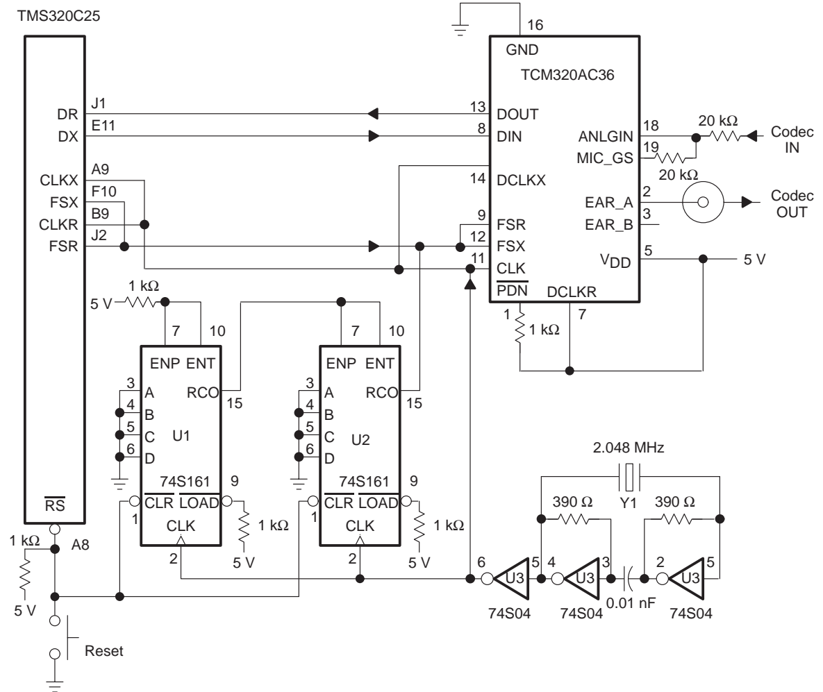
Figure 4–6. Typical DSP/Combo Interface
