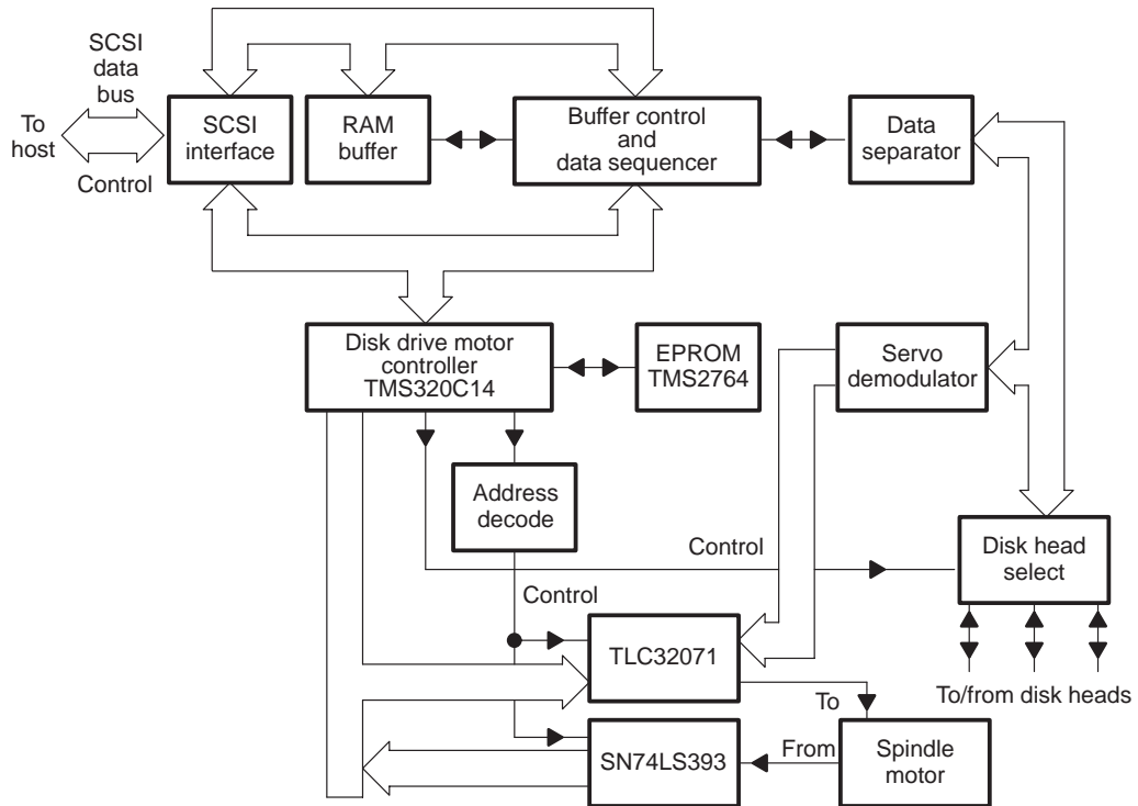
Figure 4–9. Disk Drive Control System Block Diagram
