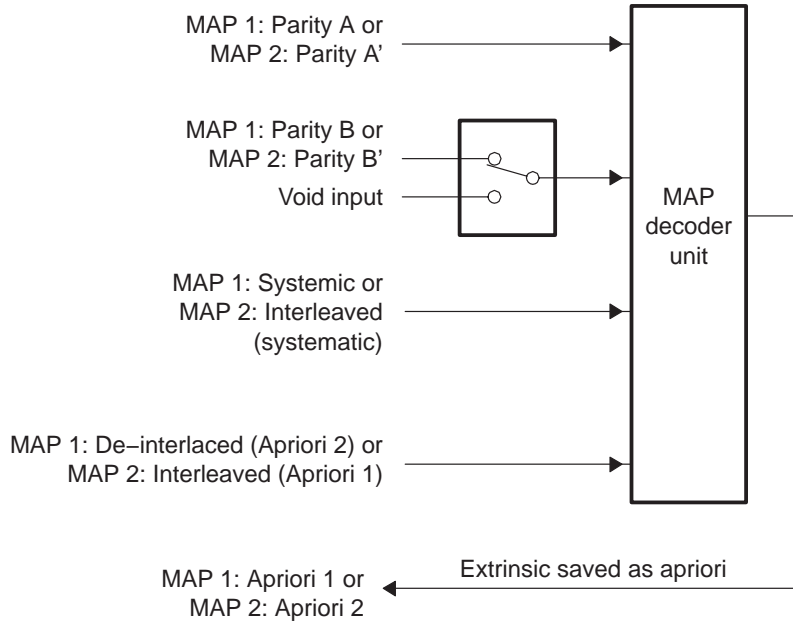
Figure 18. TCP2 Shared Processing Block Diagram
