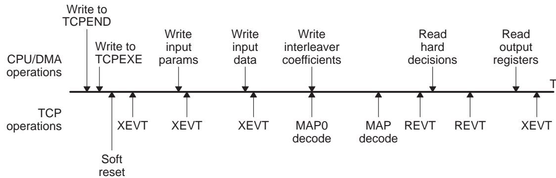
Figure 98. TCP2 Events Generation in Standalone (SA) Mode
