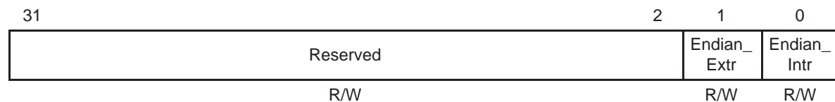
Figure 80. TCP_ENDIAN Register
