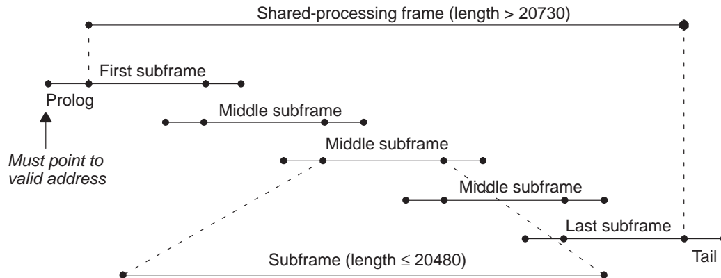
Figure 96. Shared Processing Subframe Segmentation (Example with 5 Subframes)
