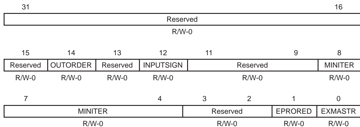
Figure 33. TCP2 Input Configuration Register 3 (TCPIC3)
