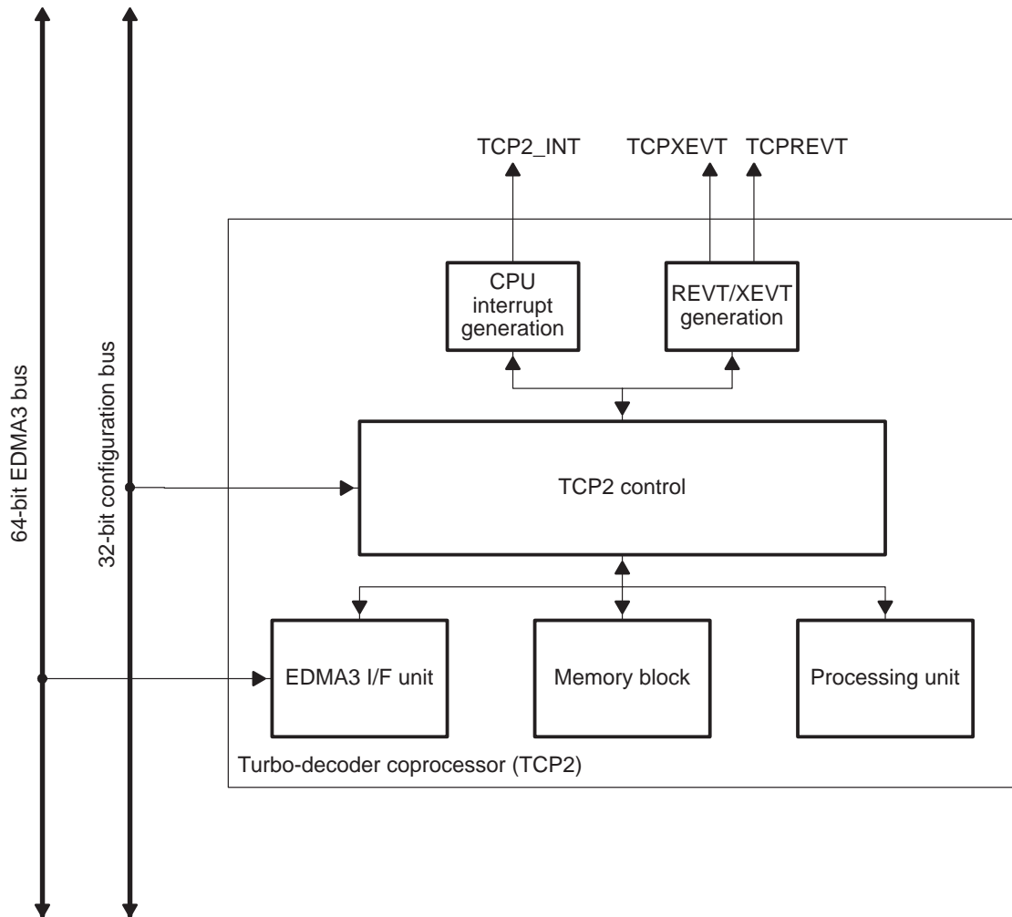
Figure 3. TCP2 Block Diagram
