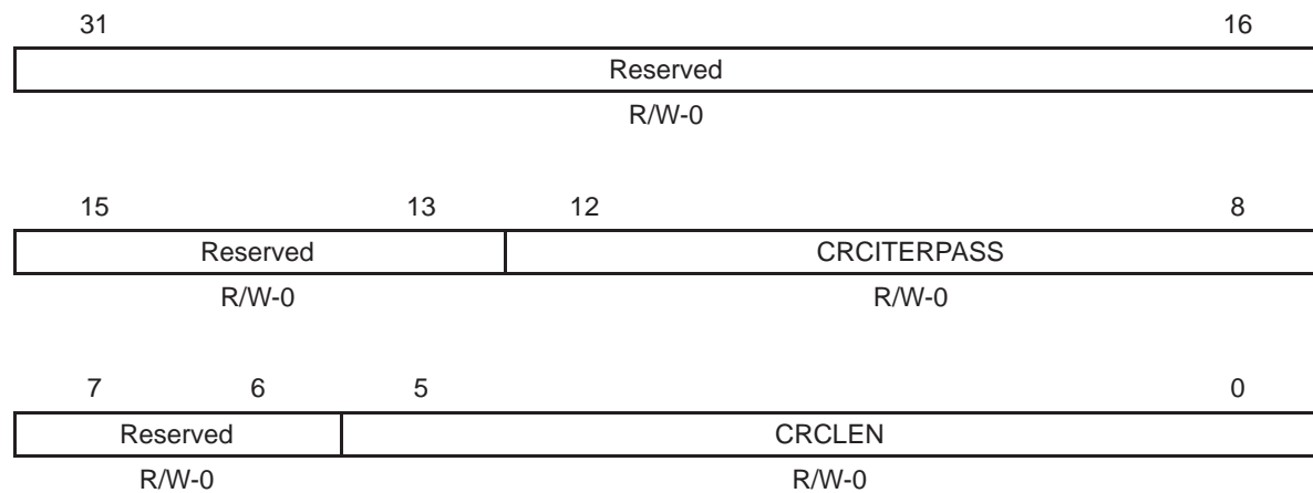
Figure 34. TCP2 Input Configuration Register 4 (TCPIC4)
