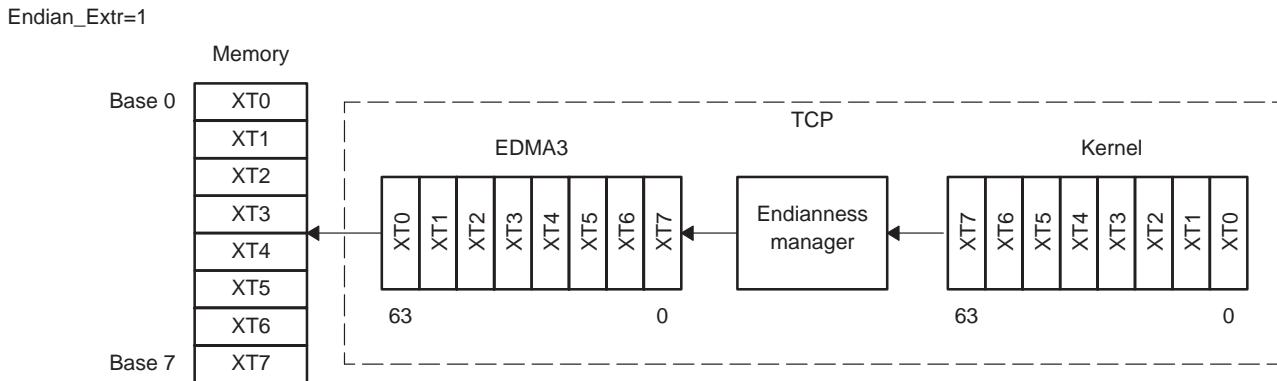
Figure 88. Extrinsic in DSP Memory (Endian_Extr = 1)
