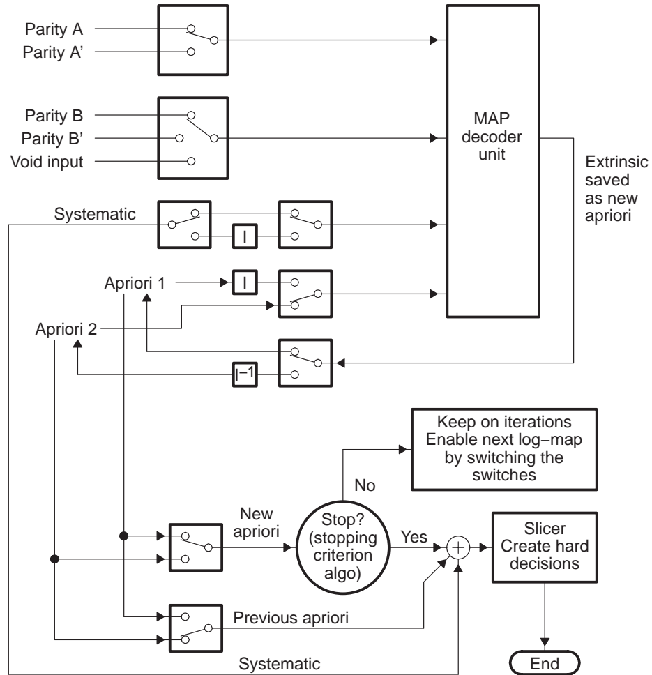
Figure 4. Standalone (SA) Mode Block Diagram
