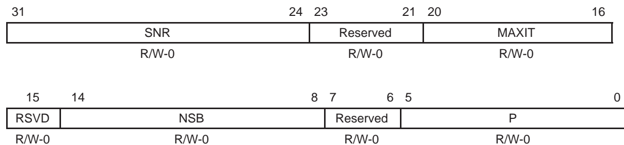
Figure 32. TCP2 Input Configuration Register 2 (TCPIC2)
