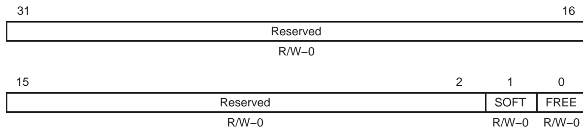
Figure 54. TCP2 Emulation Register (TCPEMU)
