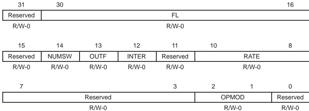
Figure 30. TCP2 Input Configuration Register 0 (TCPIC0)
