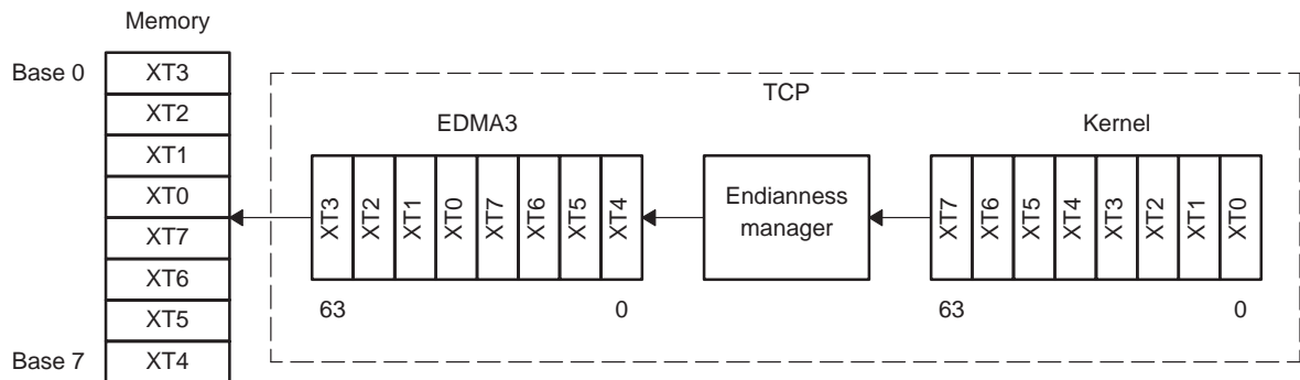
Figure 91. Extrinsic in DSP Memory (Endian_Extr = 0)
