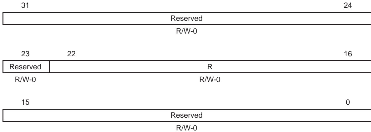
Figure 31. TCP2 Input Configuration Register 1 (TCPIC1)
