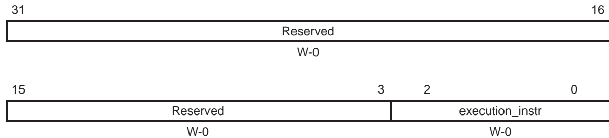
Figure 49. TCP2 Execution Register (TCPEXE)
