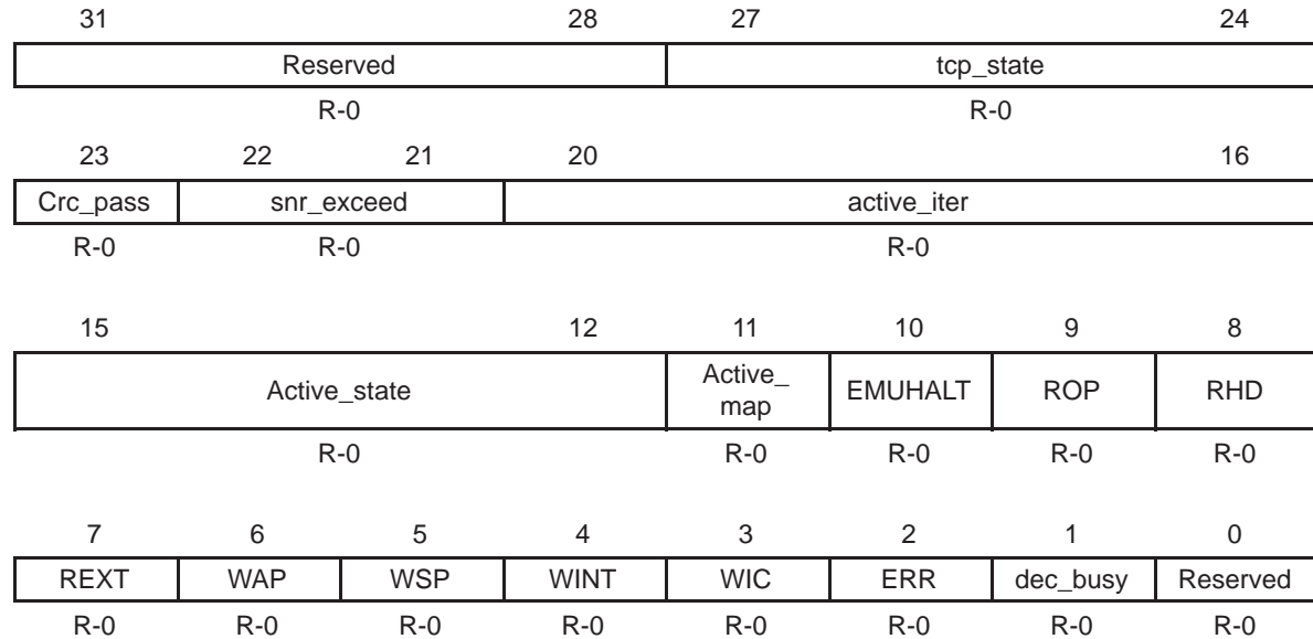
Figure 52. TCP2 Status Register (TCPSTAT)
