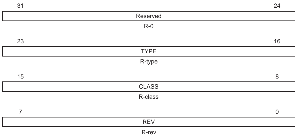
Figure 53. Peripheral Identification Register (PID)
