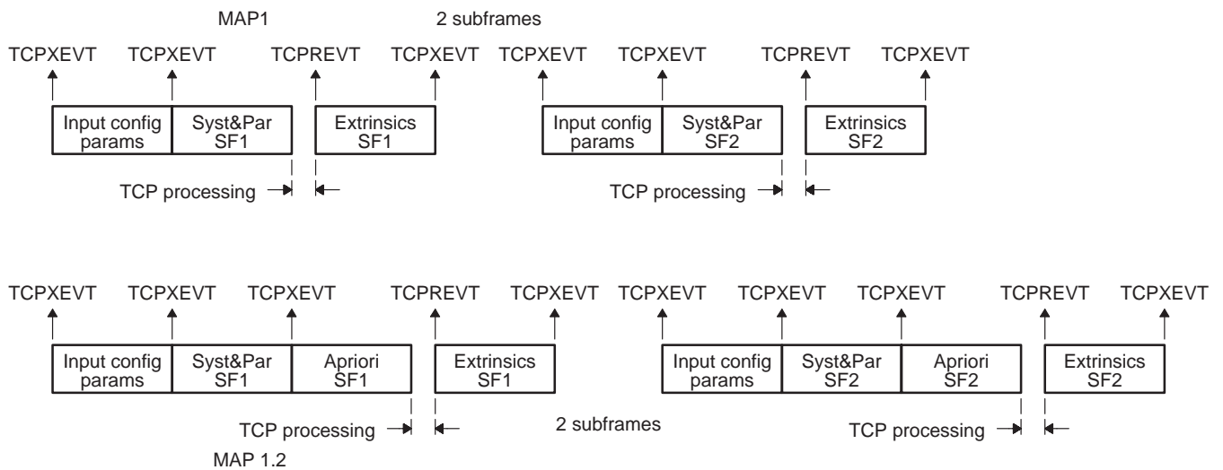
Figure 99. TCP2 Events Generation in Shared-Processing (SP) Mode
