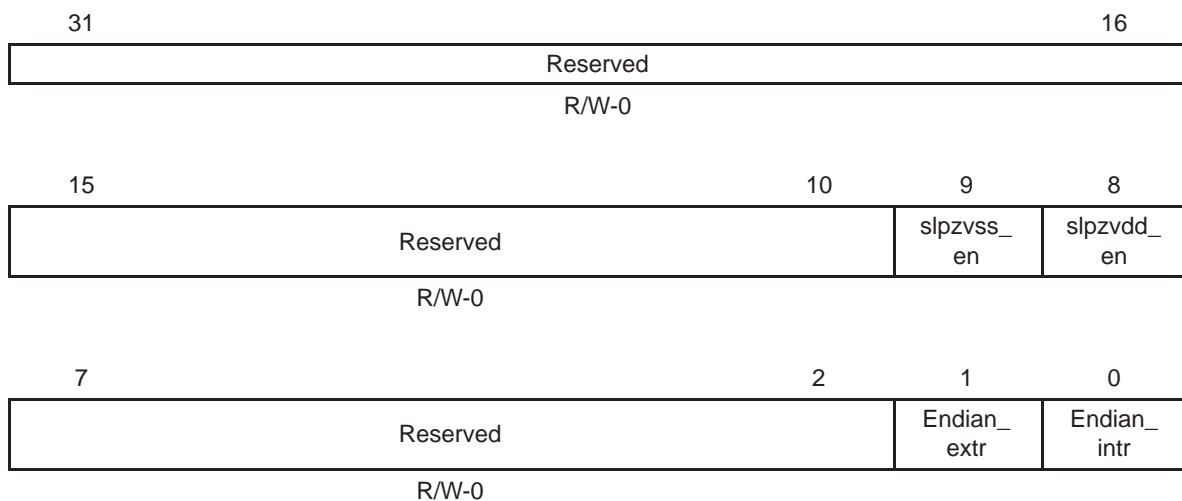
Figure 50. TCP2 Endian Register (TCPEND)
