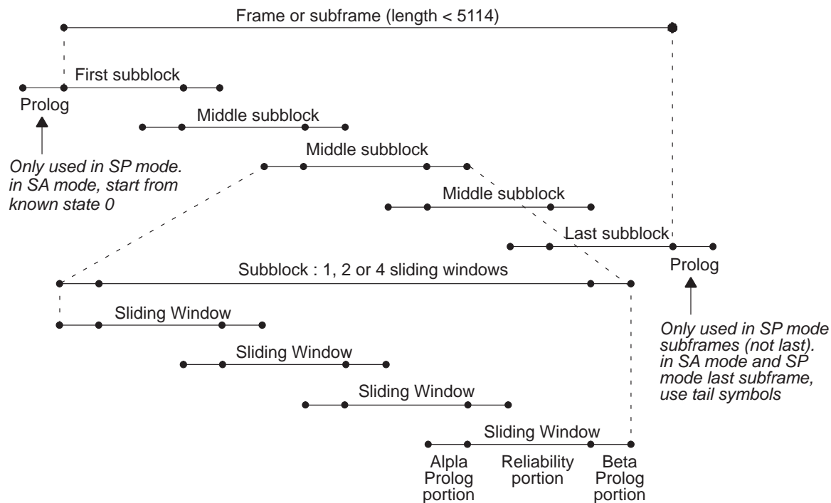
Figure 95. Sliding Windows and Subblocks Segmentation (Example with 5 Subblocks, frame length \leq 20730 )
