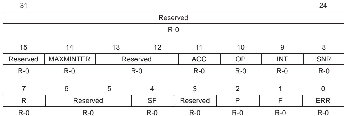
Figure 51. TCP2 Error Register (TCPERR)
