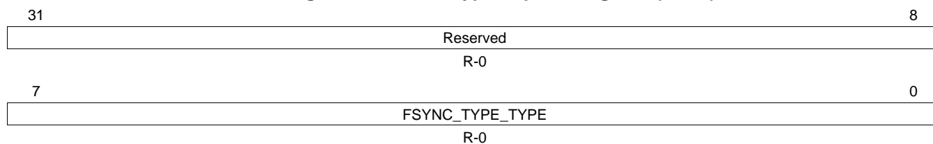
Figure 28. FSYNC Type Capture Register (TYPE)
