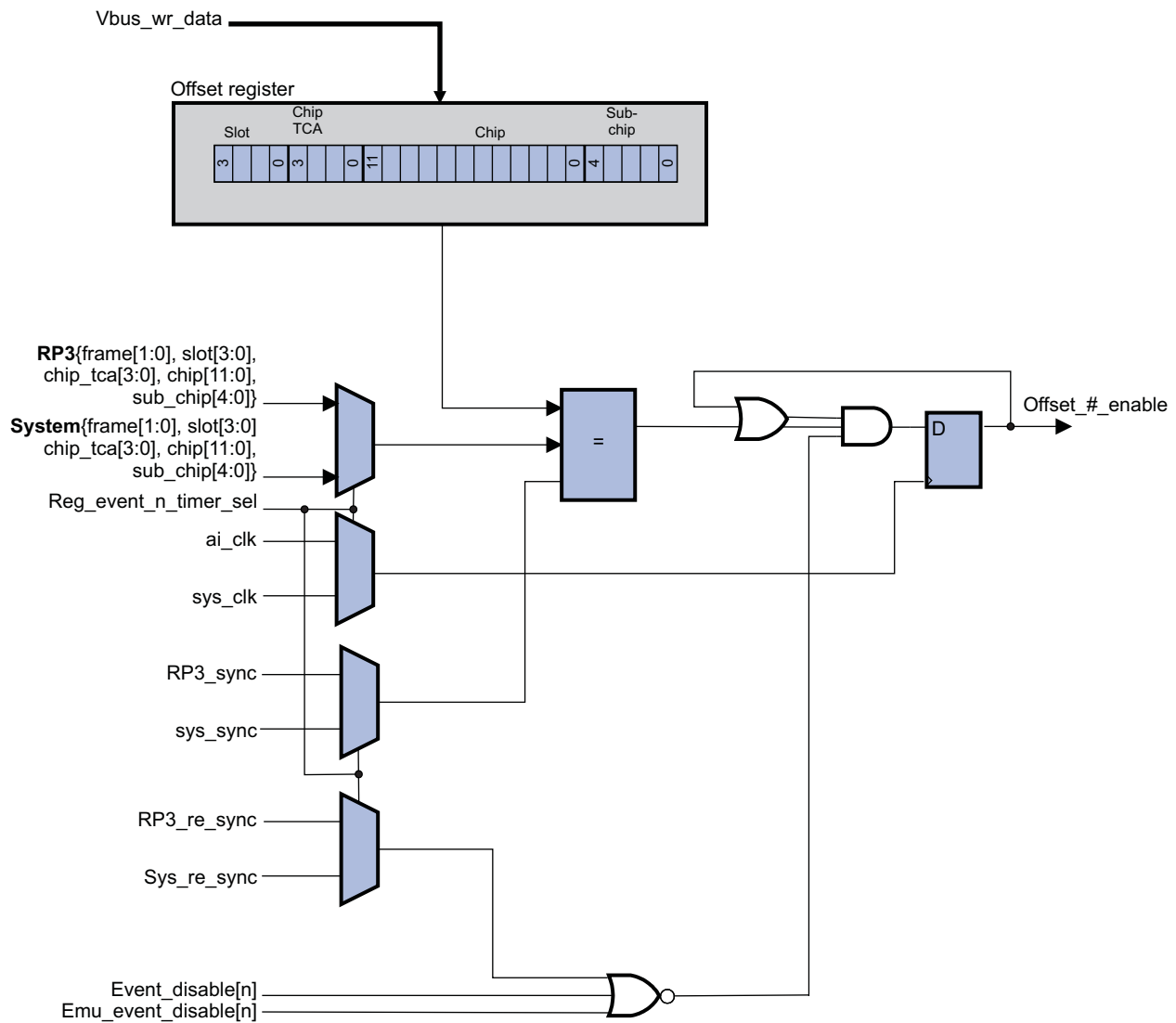
Figure 5. Event Generator Offset Condition
