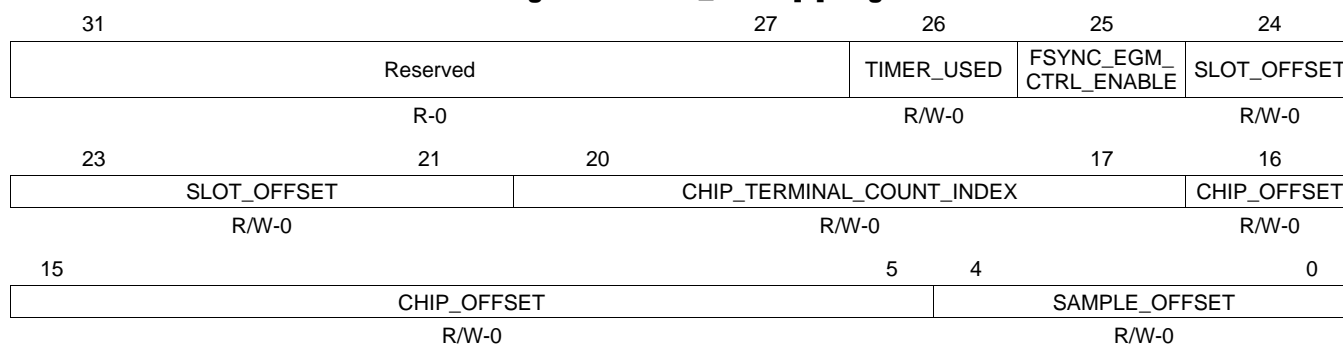
Figure 50. EGM_CTRL [0] Register
