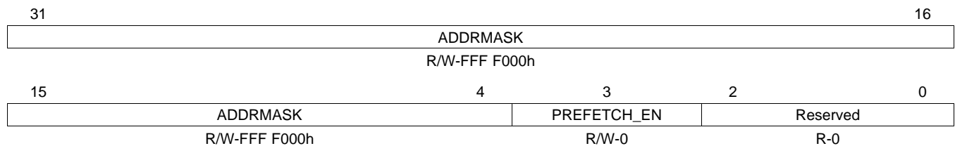
Figure 44. Base Address 1 Mask Register (PCIBAR1MSK)
