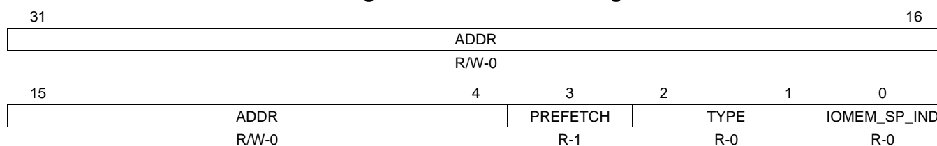
Figure 27. Base Address 4 Register
