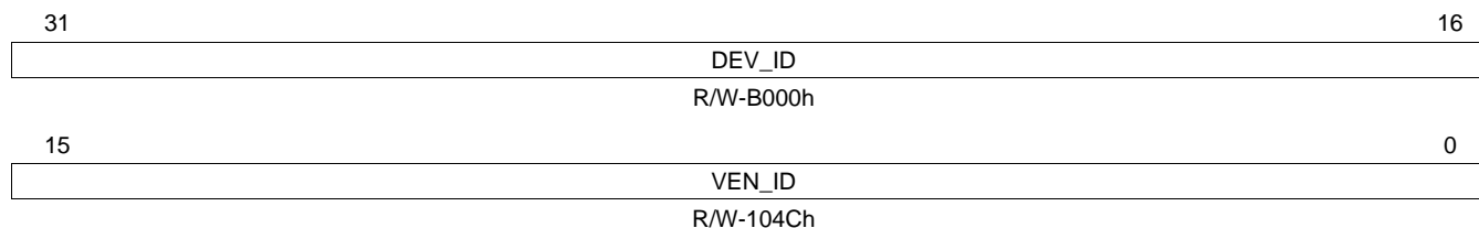
Figure 39. Vendor ID/Device ID Mirror Register (PCIVENDEVMIR)
