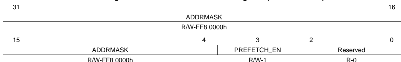
Figure 48. Base Address 5 Mask Register (PCIBAR5MSK)
