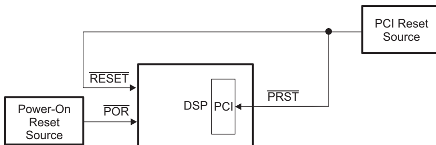
Figure 4. PCI Reset ( \overline{PRST} ) and Warm Reset ( \overline{RESET} ) Tied Together from Single External Source
