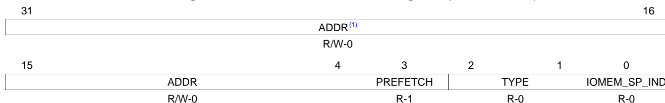
Figure 62. Base Address 3 Mirror Register (PCIBAR3MIR)
