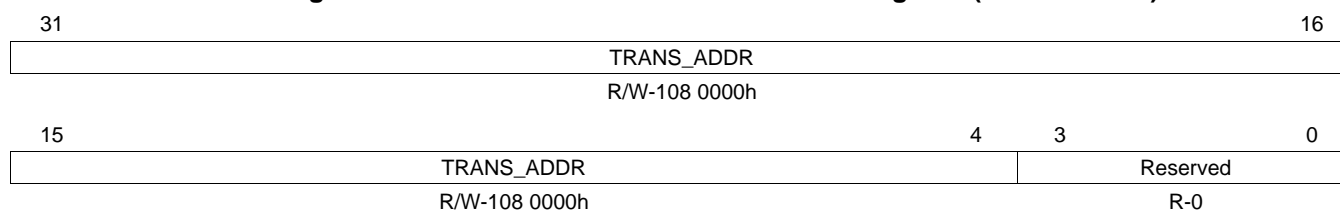
Figure 56. Slave Base Address 3 Translation Register (PCIBAR3TRL)
