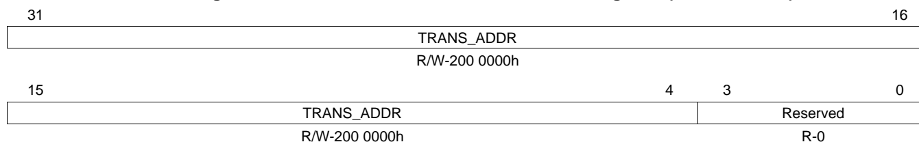
Figure 54. Slave Base Address 1 Translation Register (PCIBAR1TRL)
