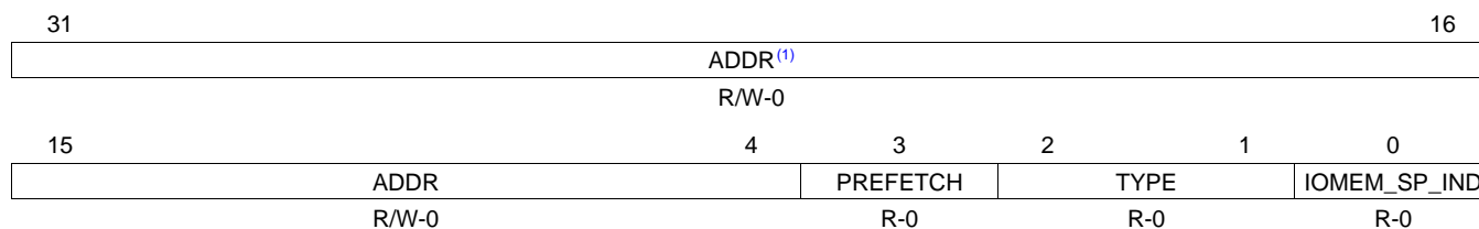
Figure 61. Base Address 2 Mirror Register (PCIBAR2MIR)
