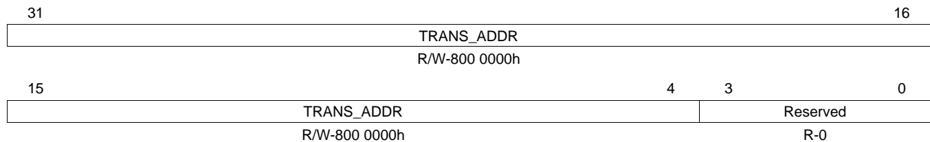
Figure 58. Slave Base Address 5 Translation Register (PCIBAR5TRL)
