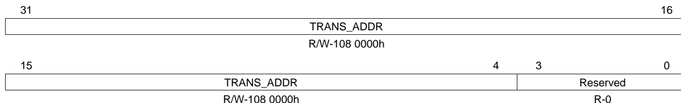
Figure 53. Slave Base Address 0 Translation Register (PCIBAR0TRL)
