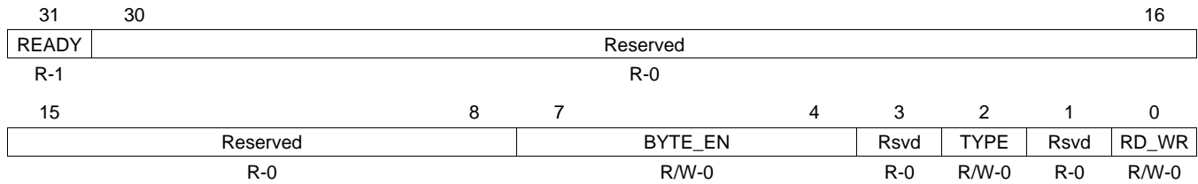
Figure 67. Master Configuration/IO Access Command Register (PCIMCFGCMD)
