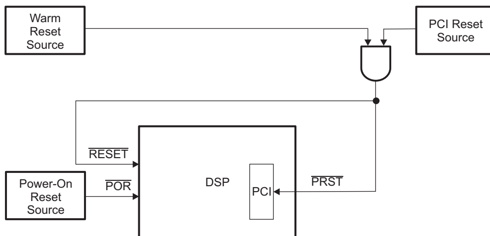
Figure 5. Independent External Power-On Reset ( \overline{POR} ), Warm Reset ( \overline{RESET} ), and PCI Reset ( \overline{PRST} ) Sources
