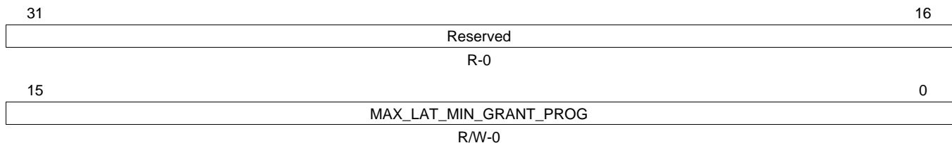
Figure 73. Maximum Latency and Minimum Grant Program Register (PCIMAXLGPRG)
