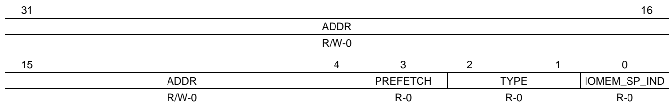
Figure 24. Base Address 1 Register
