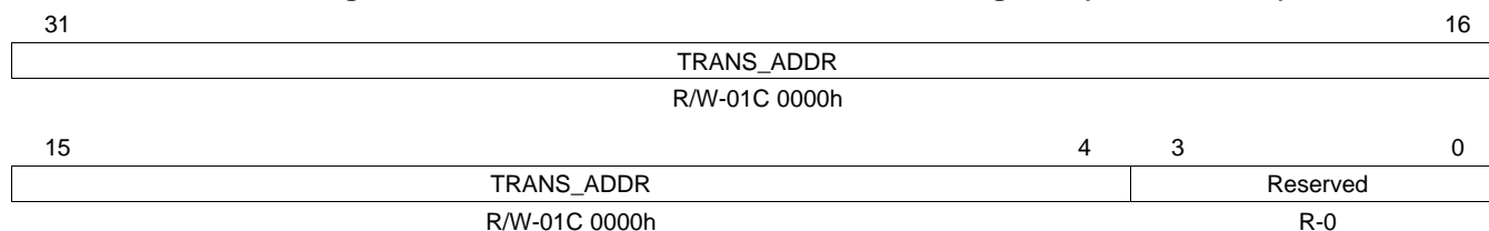
Figure 55. Slave Base Address 2 Translation Register (PCIBAR2TRL)
