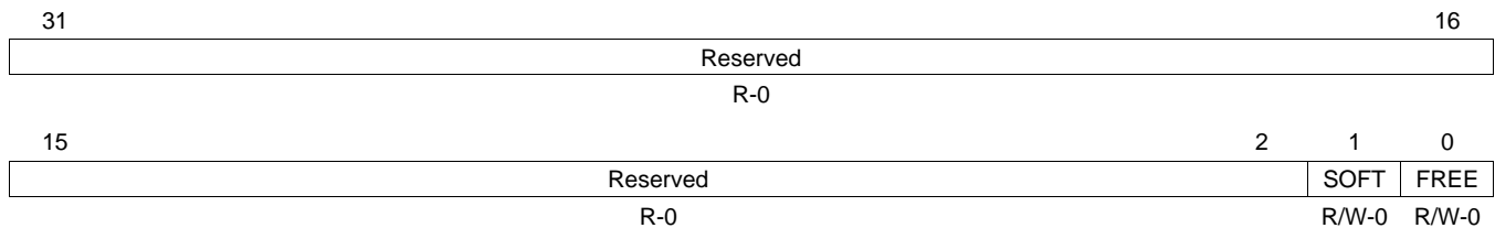
Figure 18. Power and Emulation Management Register (PWREMU_MGMT)
