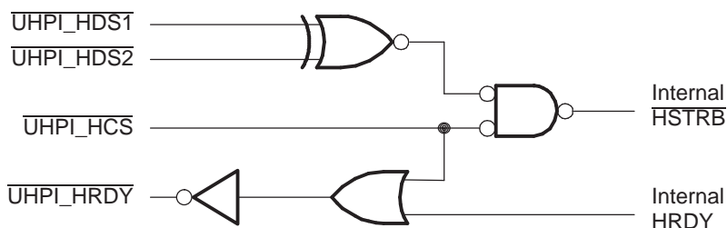
Figure 3. HPI Strobe and Select Logic
