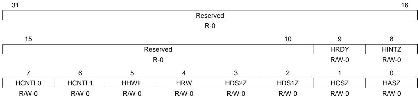
Figure 23. GPIO Data 2 Register (GPIO_DAT2)
