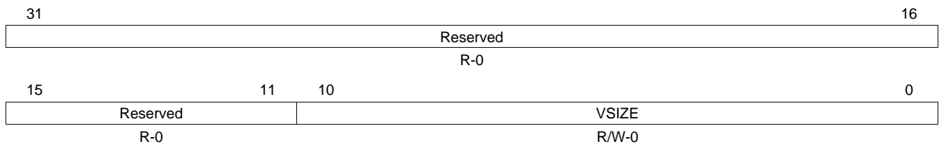
Figure 57. Channel n Vertical Image Size Register (C n VSIZE)
