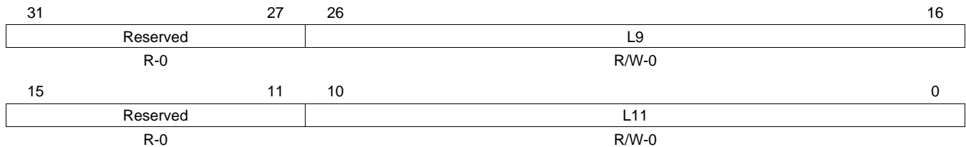
Figure 56. Channel n Vertical Size Configuration 2 Register (C n VCFG2)
