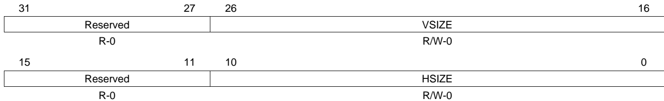
Figure 65. Channel n Bottom Field Vertical Ancillary Size Register (C n BVANCSIZE)
