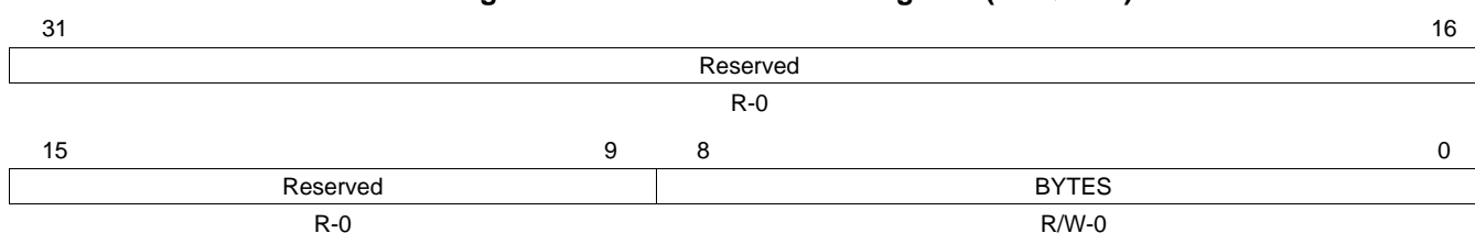
Figure 35. DMA Size Control Register (REQSIZE)
