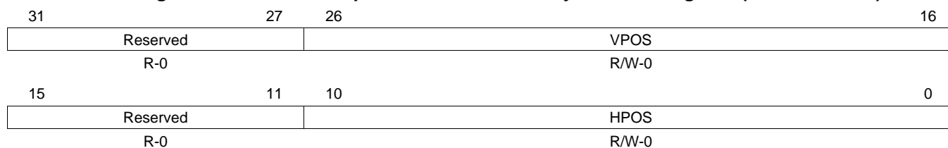
Figure 62. Channel n Top Field Vertical Ancillary Position Register (C n TVANCPOS)
