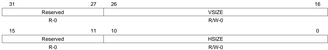
Figure 63. Channel n Top Field Vertical Ancillary Size Register (C n TVANCSIZE)
