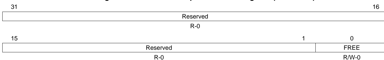
Figure 34. Emulation Suspend Control Register (EMUCTRL)
