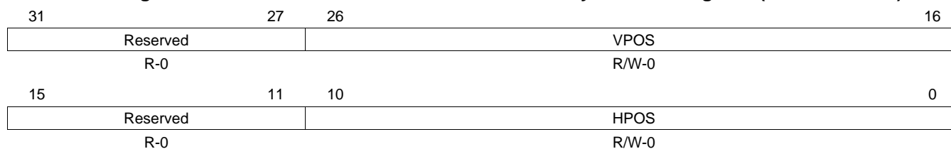
Figure 64. Channel n Bottom Field Vertical Ancillary Position Register (C n BVANCPOS)
