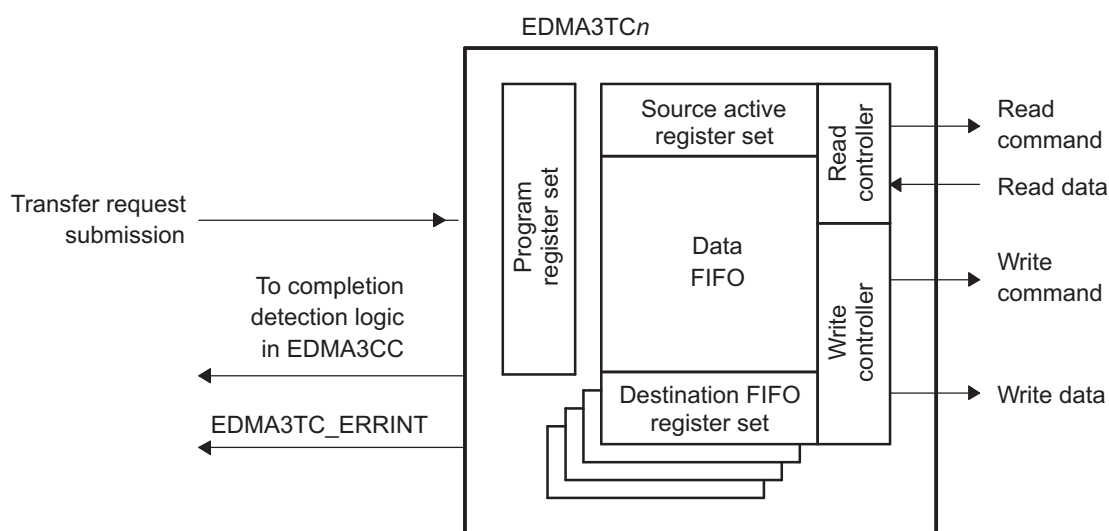
Figure 18-3. EDMA3 Transfer Controller (EDMA3TC) Block Diagram
