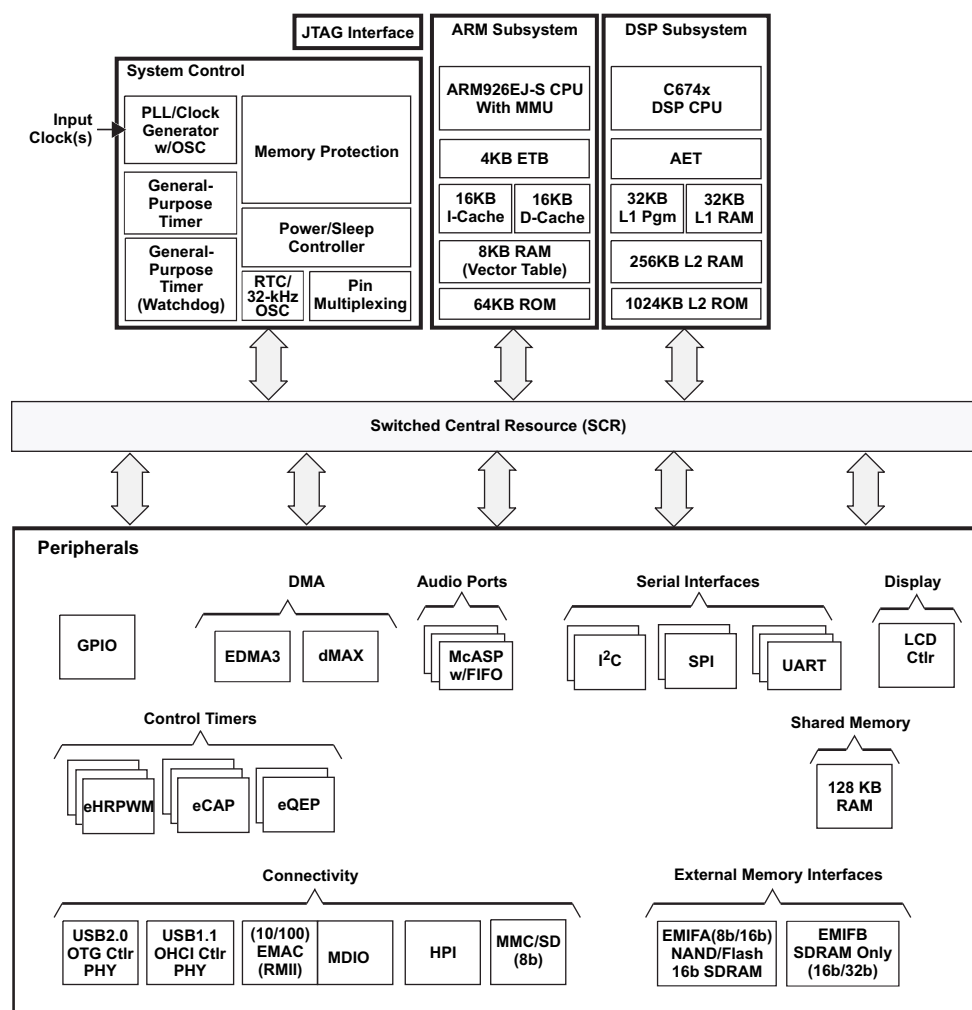
Figure 1-1. TMS320DA828/DA830 DSP Block Diagram
