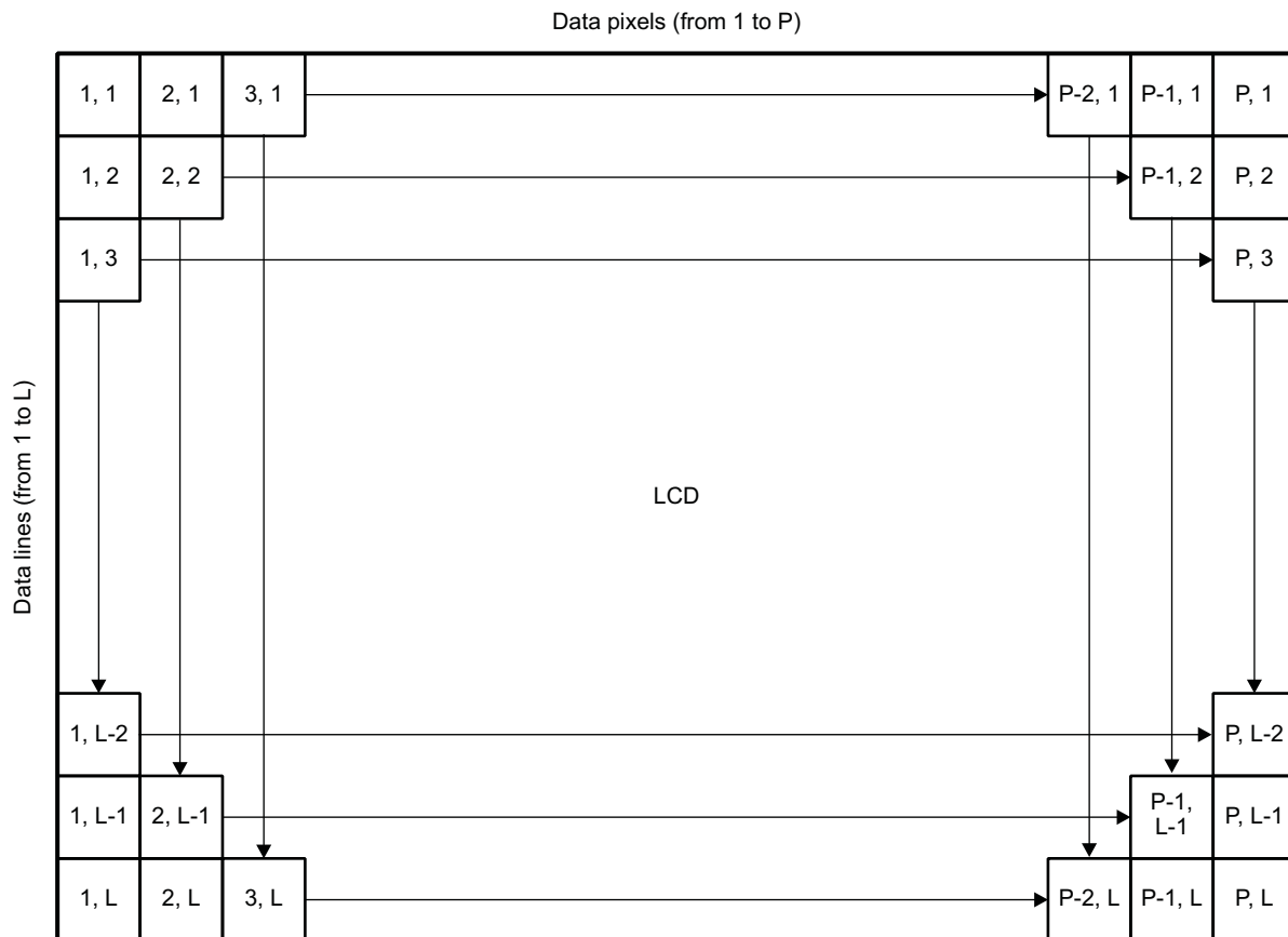
Figure 25-14. Raster Mode Display Format
