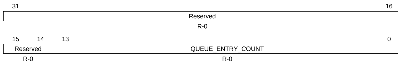
Figure 33-115. Queue Manager Queue N Status Register A (QSTATATA[ N ])
