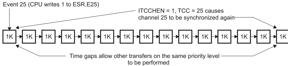
Figure 18-34. Smaller Packet Data Transfers Example
