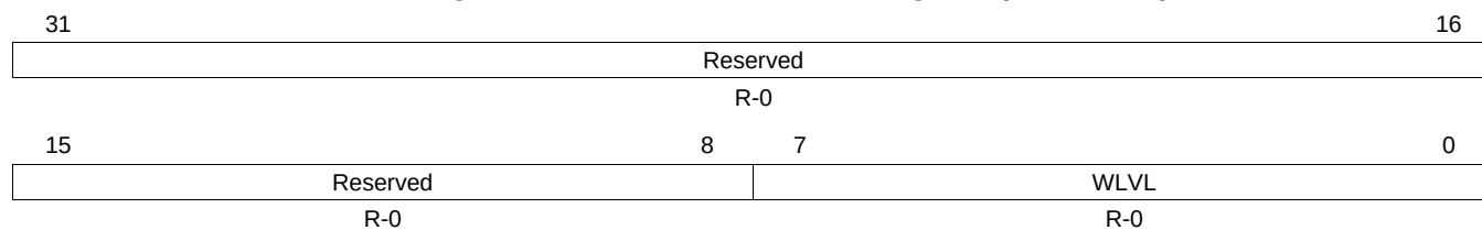
Figure 26-79. Write FIFO Status Register (WFIFOSTS)
