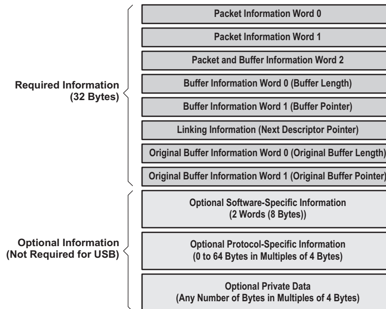
Figure 33-16. Host Packet Descriptor Layout
