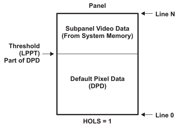
Figure 25-39. Subpanel Display: SPEN = 1, HOLDS = 1
