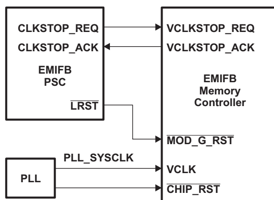
Figure 21-10. EMIFB Memory Controller Power and Sleep Controller Diagram
