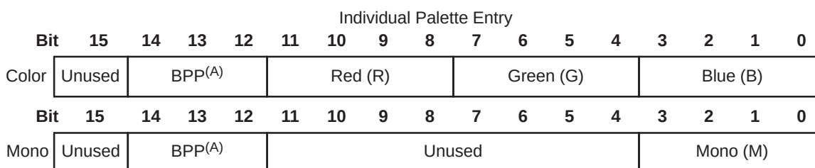
Figure 25-5. 16-Entry Palette/Buffer Format (1, 2, 4, 12, 16 BPP)
