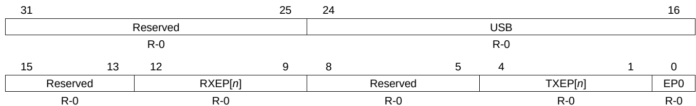
Figure 33-38. USB Interrupt Mask Register (INTMSKR)
