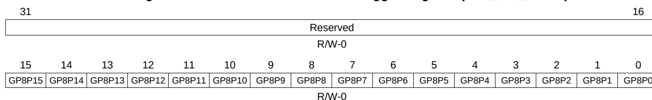
Figure 22-33. GPIO Bank 8 Set Rise Trigger Register (SET_RIS_TRIG8)
