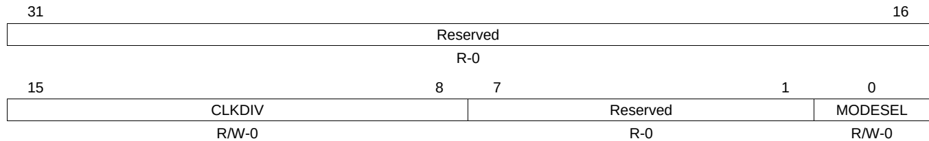
Figure 25-16. LCD Control Register (LCD_CTRL)
