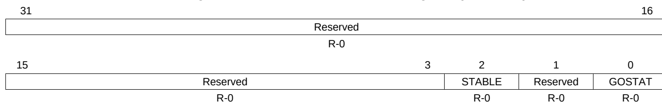
Figure 8-18. PLL Controller Status Register (PLLSTAT)
