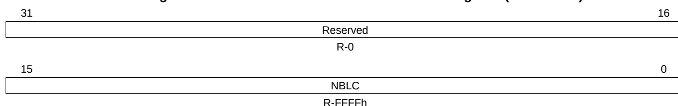
Figure 27-26. MMC Number of Blocks Counter Register (MMCNBLC)
