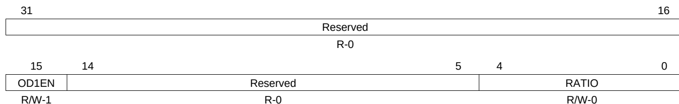
Figure 8-15. Oscillator Divider 1 Register (OSCDIV)
