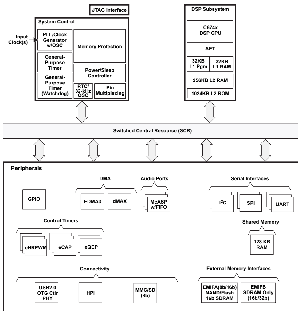
Figure 1-1. TMS320DA808/DA807/DA805/DA81x DSP Block Diagram
