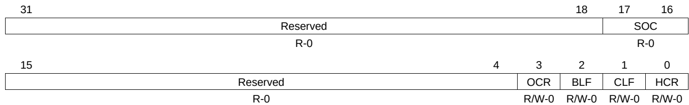
Figure 28-4. HC Command and Status Register (HCCOMMANDSTATUS)
