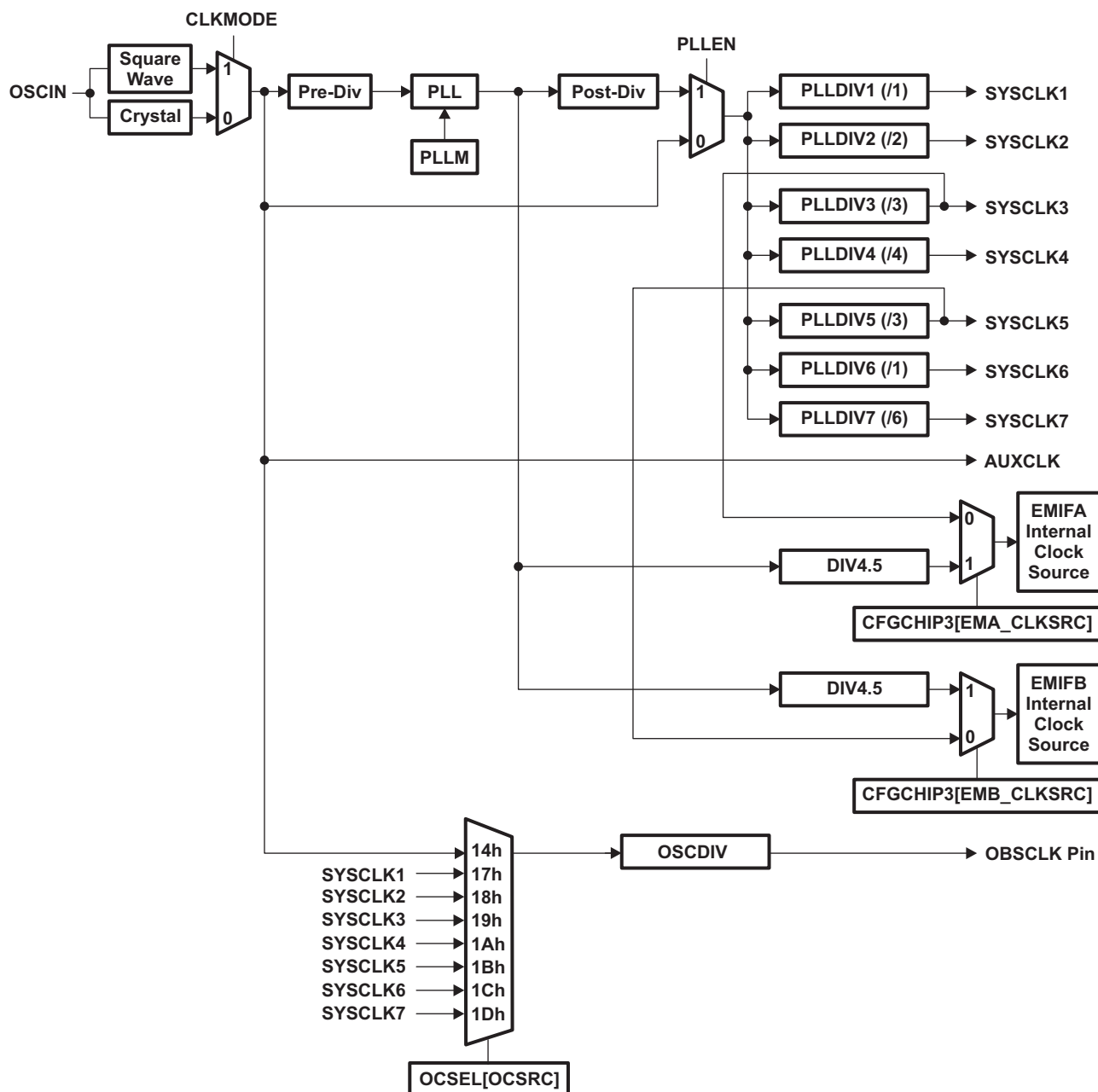
Figure 7-1. PLL0 Structure
