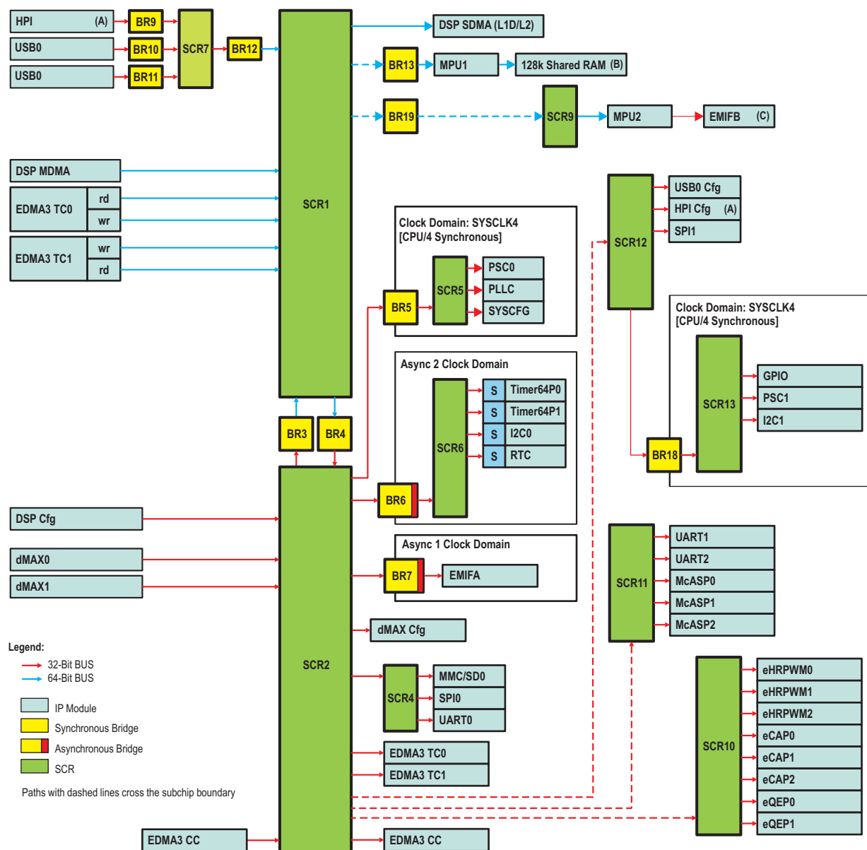
Figure 3-1. System Interconnect Block Diagram
