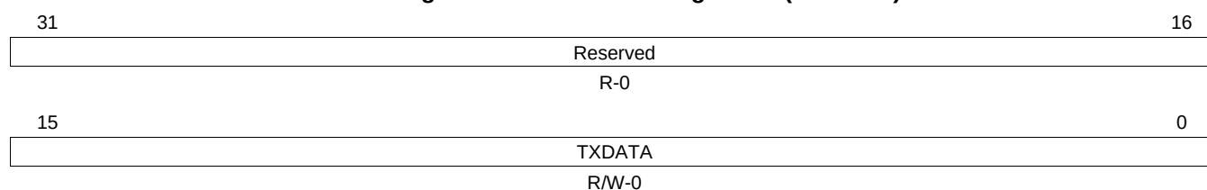
Figure 25-29. SPI Data Register 0 (SPIDAT0)
