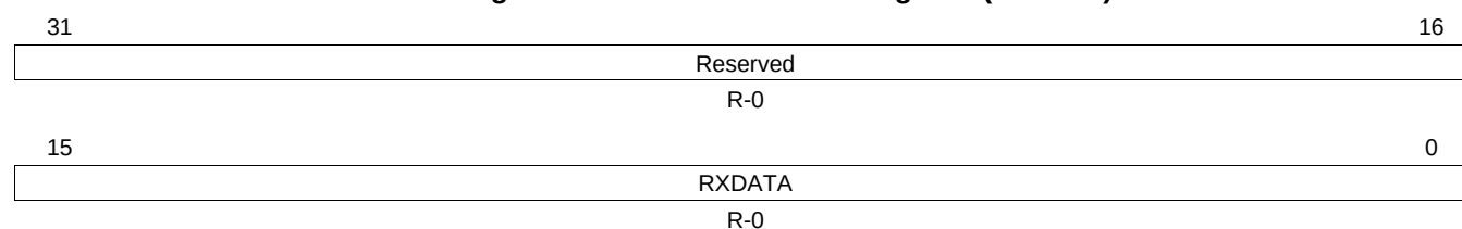
Figure 25-32. SPI Emulation Register (SPIEMU)
