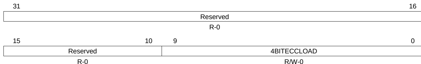
Figure 17-45. NAND Flash 4-Bit ECC LOAD Register (NAND4BITECCLOAD)
