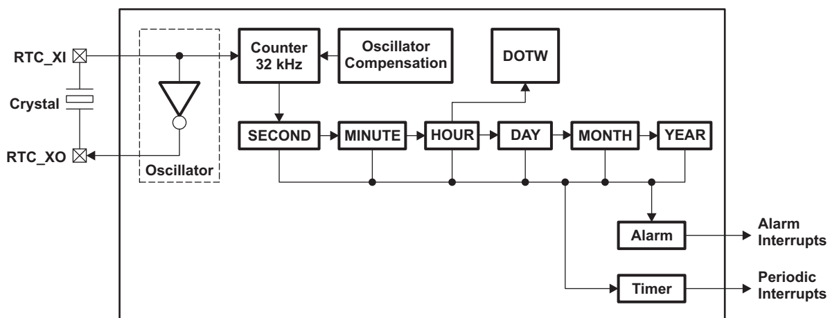
Figure 24-1. Real-Time Clock Block Diagram
