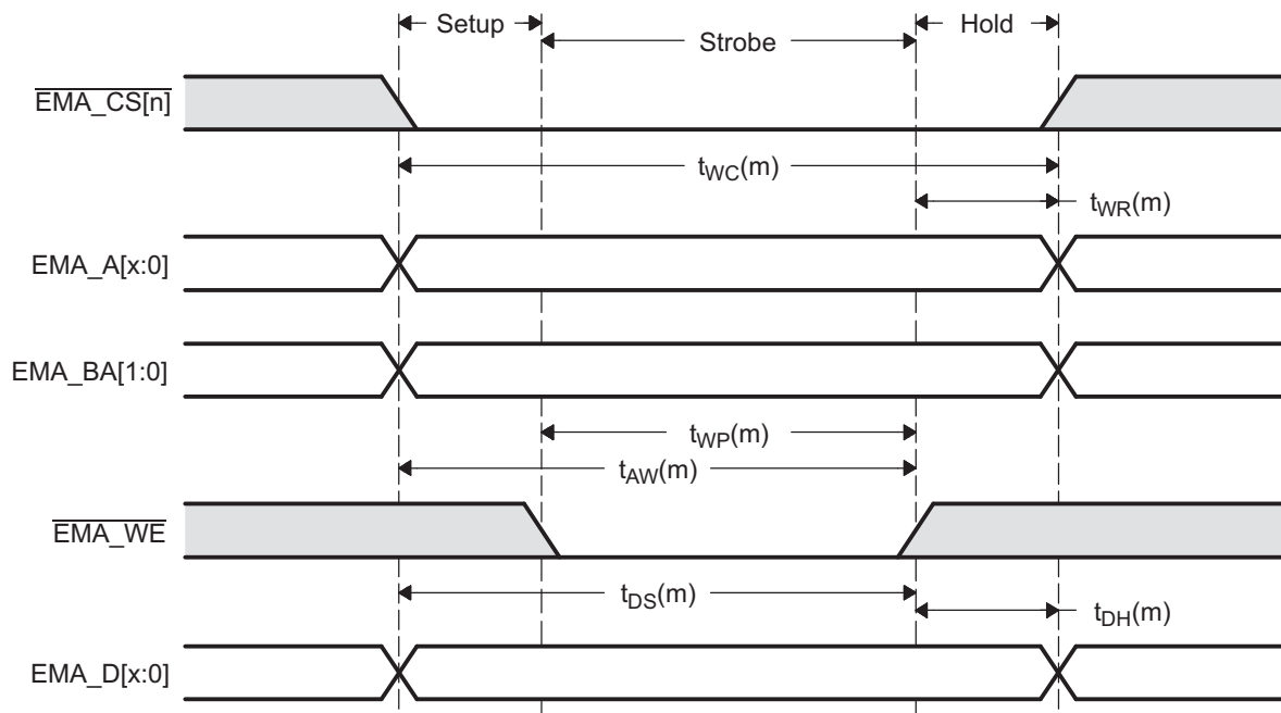
Figure 17-24. Timing Waveform of an ASRAM Write
