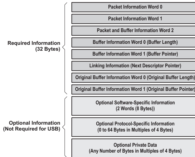
Figure 29-16. Host Packet Descriptor Layout
