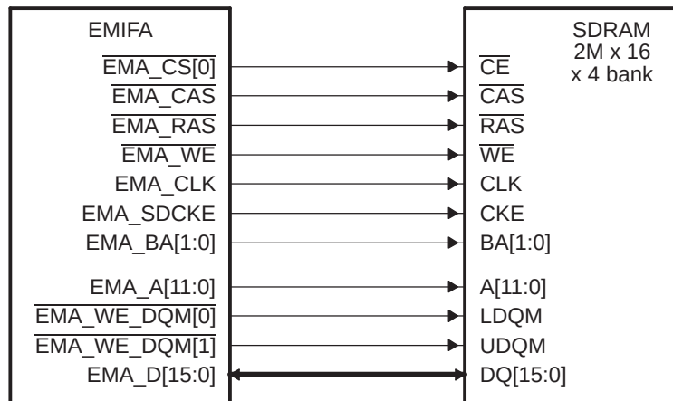
Figure 17-3. EMIFA to 2M × 16 × 4 bank SDRAM Interface
