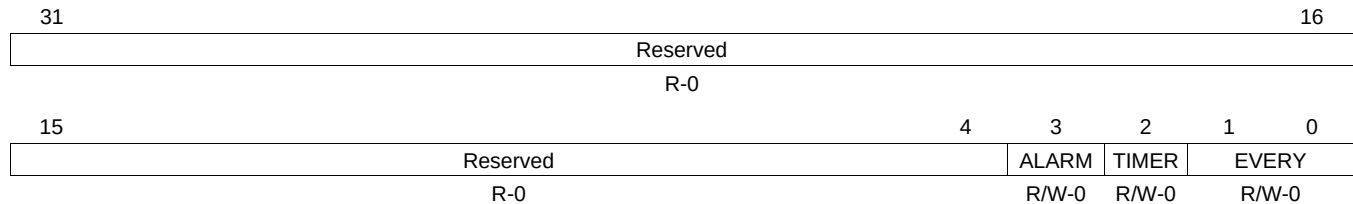
Figure 24-19. Interrupt Register (INTERRUPT)
