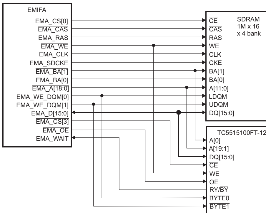
Figure 17-18. Example Configuration Interface
