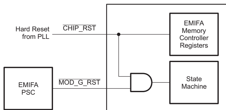
Figure 17-16. EMIFA Reset Block Diagram
