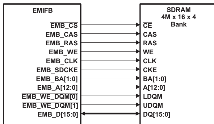
Figure 18-12. Connecting EMIFB Memory Controller for 16-bit Connection
