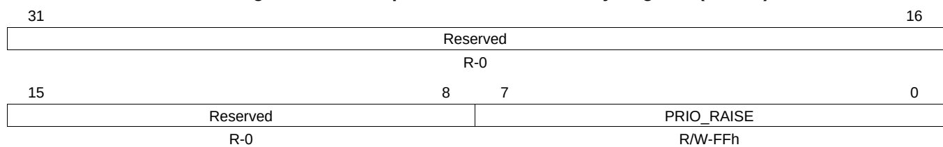
Figure 18-19. Peripheral Bus Burst Priority Register (BPRIO)
