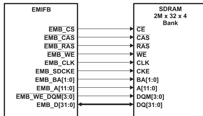
Figure 18-4. EMIFB to 2M × 32 × 4 bank SDRAM Interface
