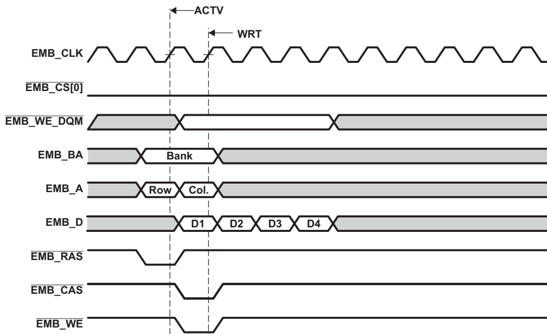
Figure 18-7. Timing Waveform for Basic SDRAM Write Operation
