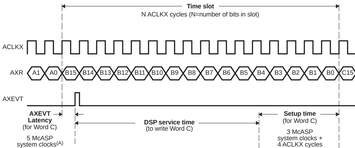
Figure 22-25. DSP Service Time Upon Transmit DMA Event (AXEVT)
