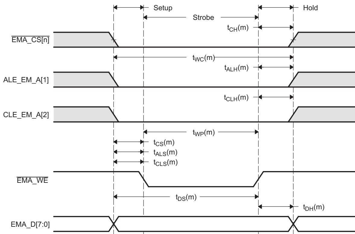
Figure 17-30. Timing Waveform of a NAND Flash Data Write
