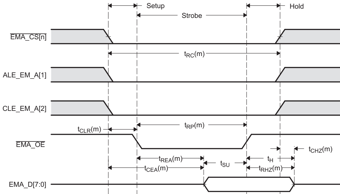
Figure 17-27. Timing Waveform of a NAND Flash Read
