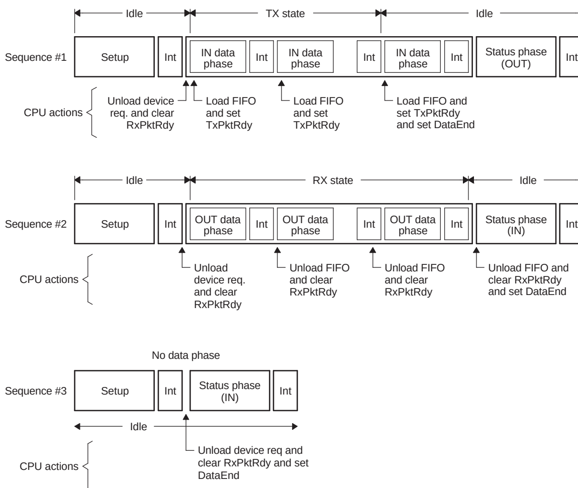
Figure 29-5. Sequence of Transfer
