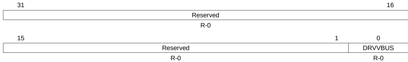
Figure 29-29. Status Register (STATR)
