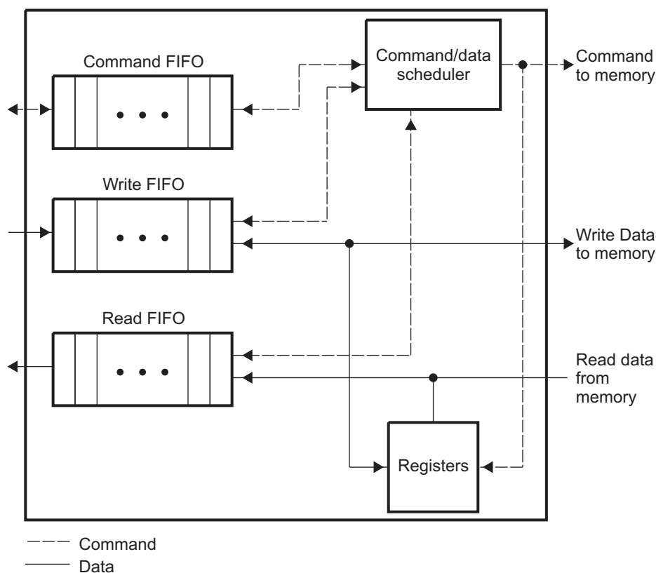
Figure 18-8. EMIFB Memory Controller FIFO Block Diagram
