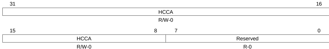
Figure 28-8. HC HCAA Address Register (HCHCCA)
