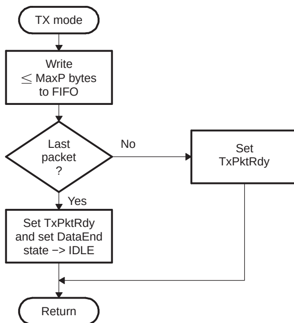
Figure 29-8. TX Mode Flow Chart
