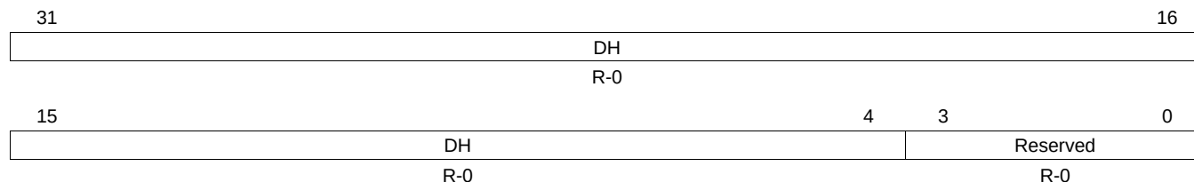
Figure 28-14. HC Head Done Register (HCDONEHEAD)
