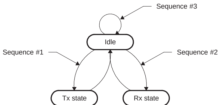
Figure 29-4. CPU Actions at Transfer Phases
