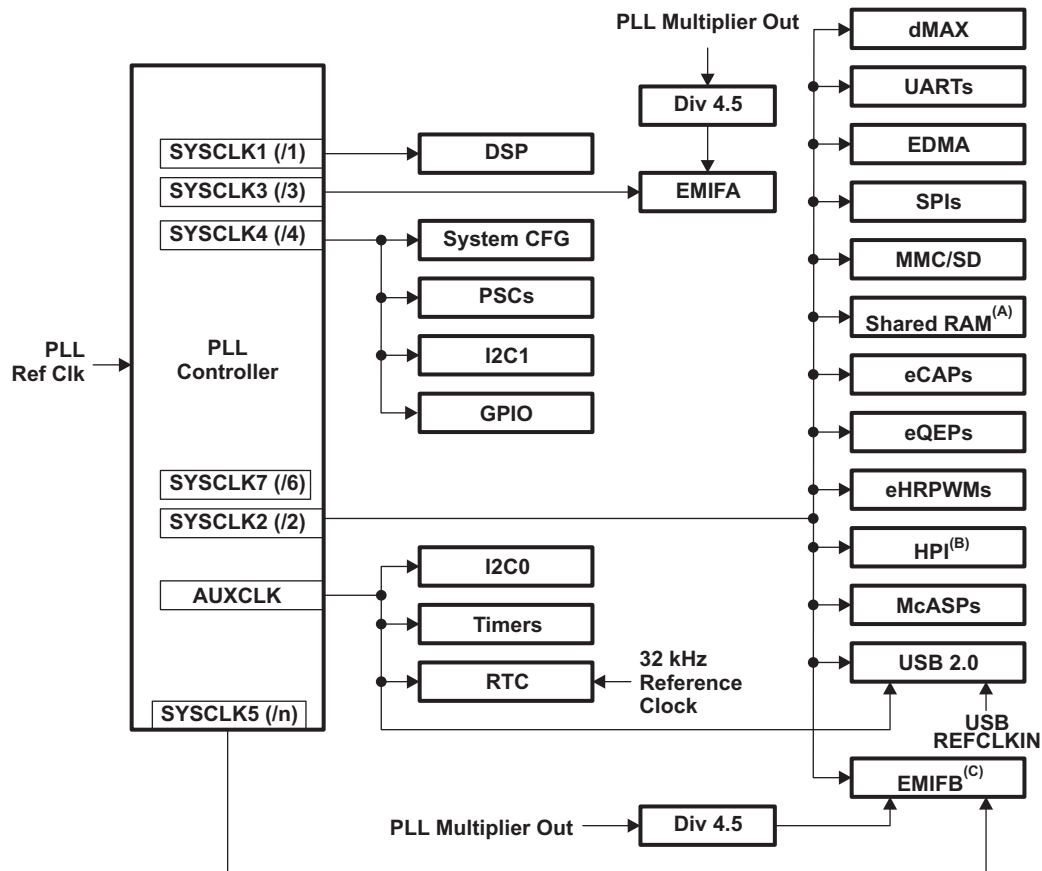
Figure 6-1. Overall Clocking Diagram
