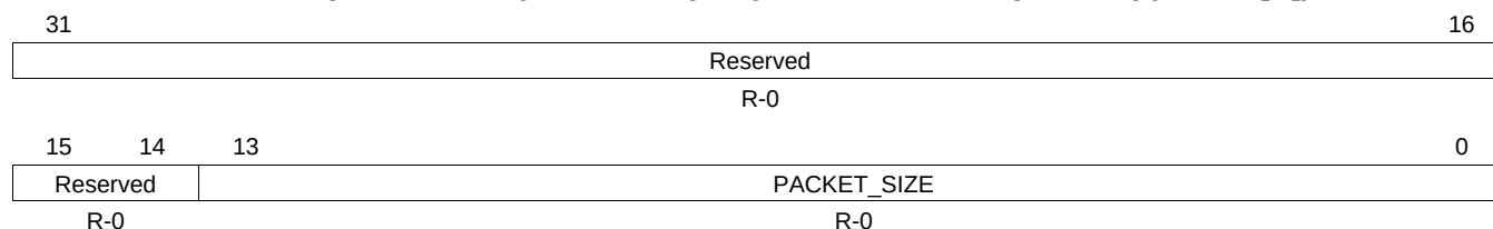
Figure 29-117. Queue Manager Queue N Status Register C (QSTATC[N])
