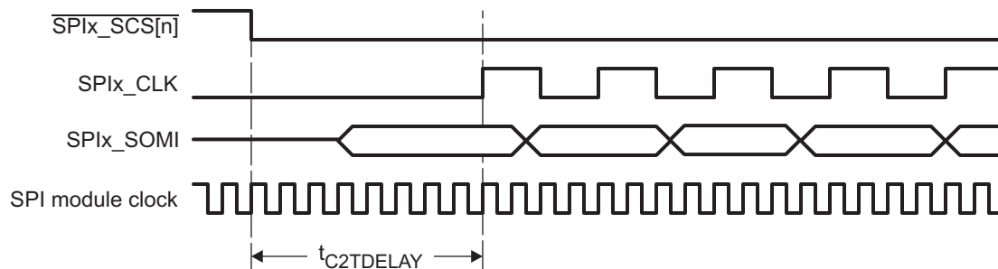
Figure 25-34. Example: t_{\text{C2EDELAY}} = 8 SPI Module Clock Cycles
