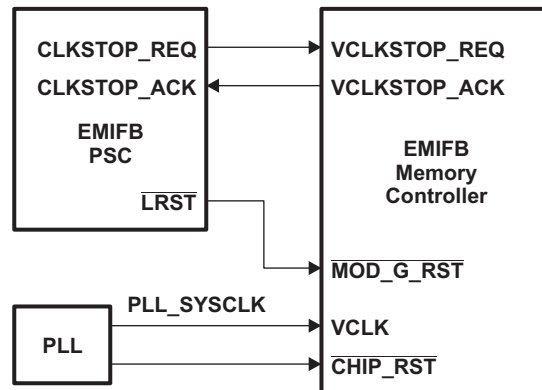
Figure 18-10. EMIFB Memory Controller Power and Sleep Controller Diagram
