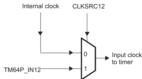
Figure 26-2. Timer Clock Source Block Diagram
