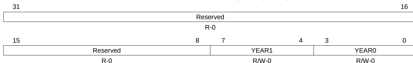
Figure 24-9. Year Register (YEAR)
