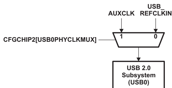
Figure 29-2. USB Clocking Diagram
