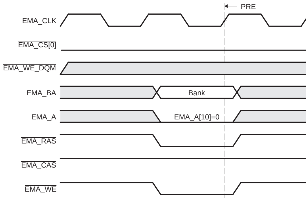
Figure 17-2. Timing Waveform of SDRAM PRE Command
