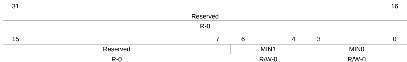
Figure 24-5. Minute Register (MINUTE)
