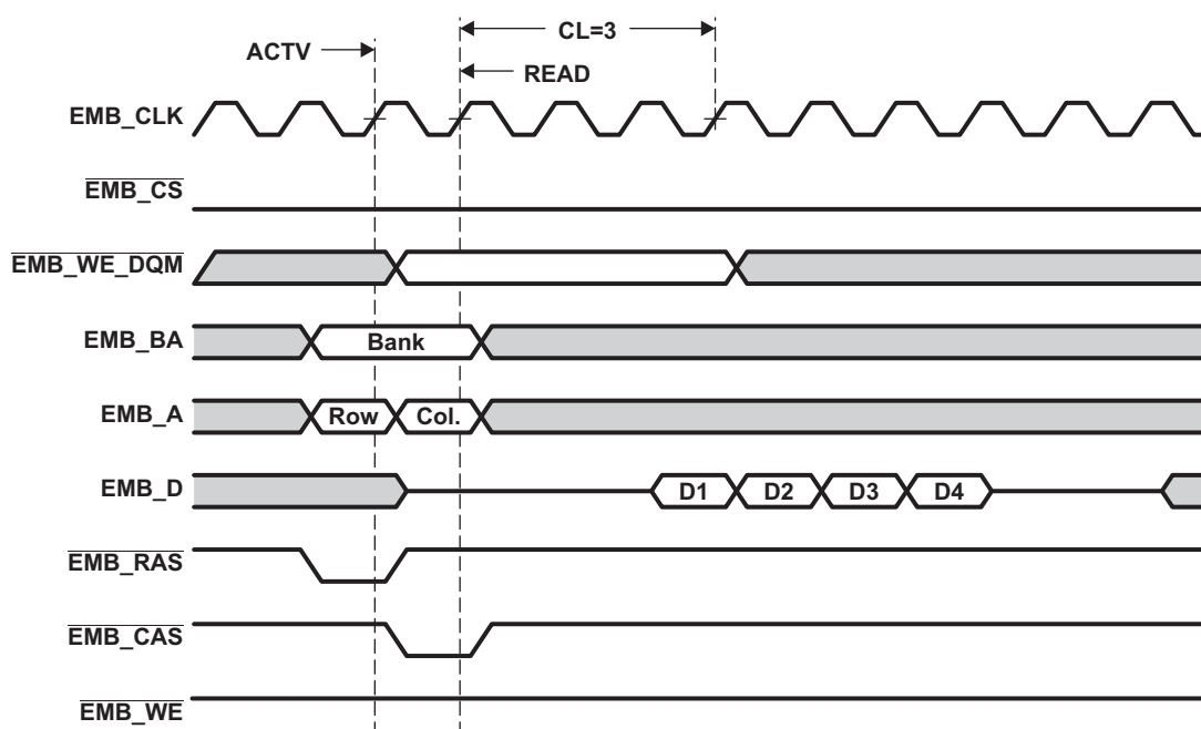
Figure 18-6. Timing Waveform for Basic SDRAM Read Operation
