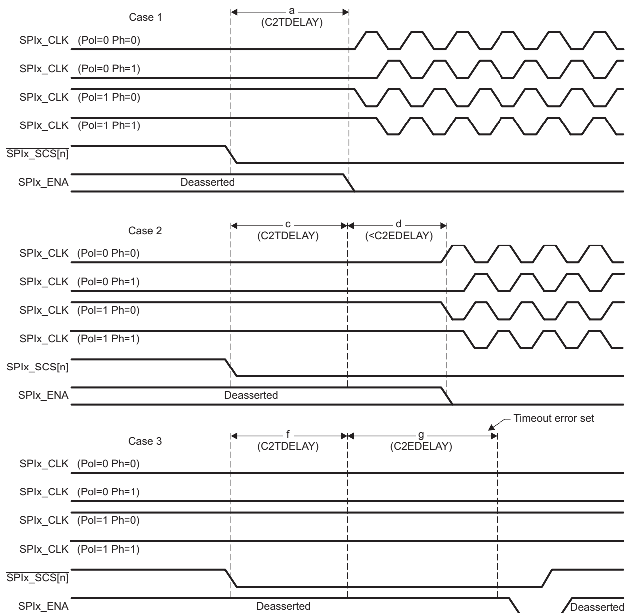
Figure 25-17. SPI 5-Pin Mode Demonstrating C2TDELAY and C2EDELAY
