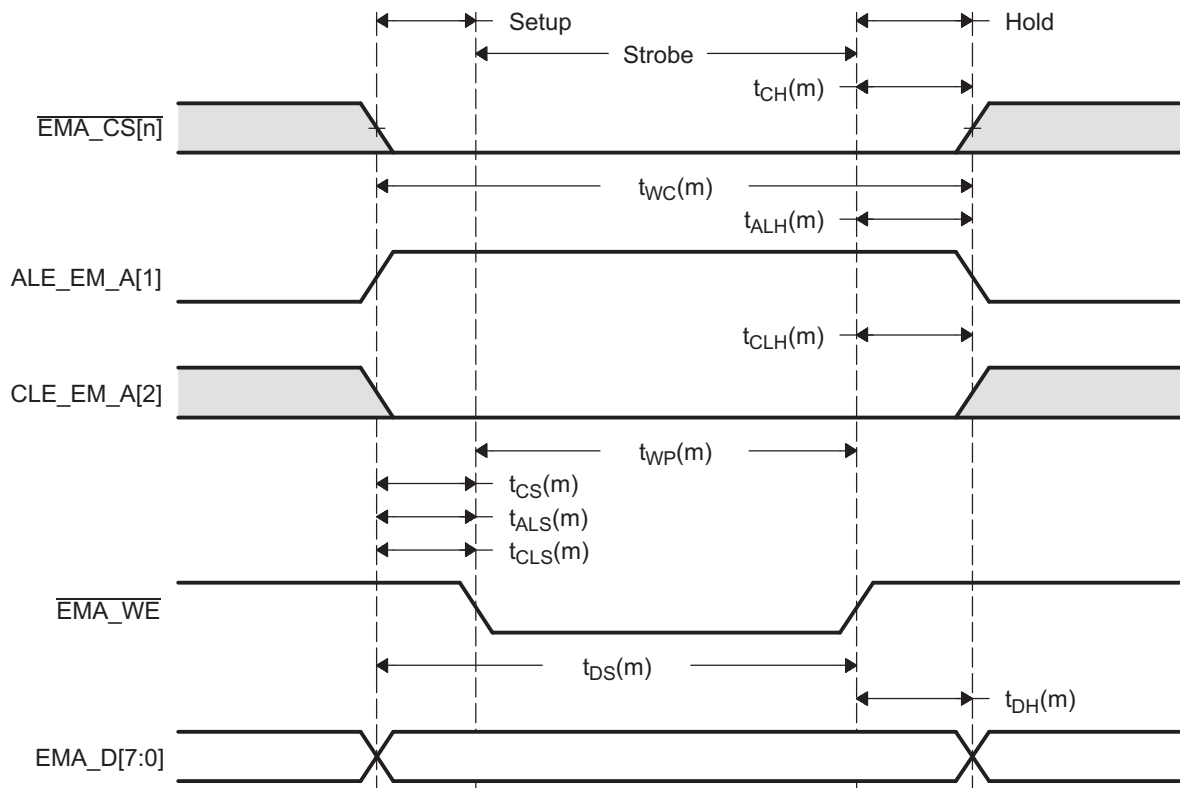
Figure 17-29. Timing Waveform of a NAND Flash Address Write
