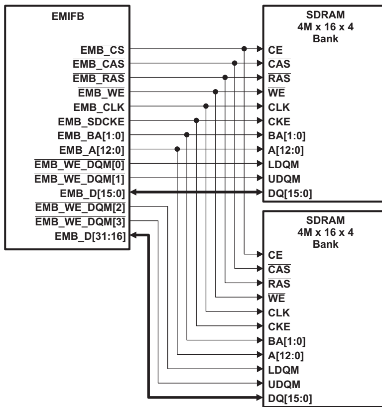
Figure 18-5. EMIFB to Dual 4M × 16 × 4 bank SDRAM Interface
