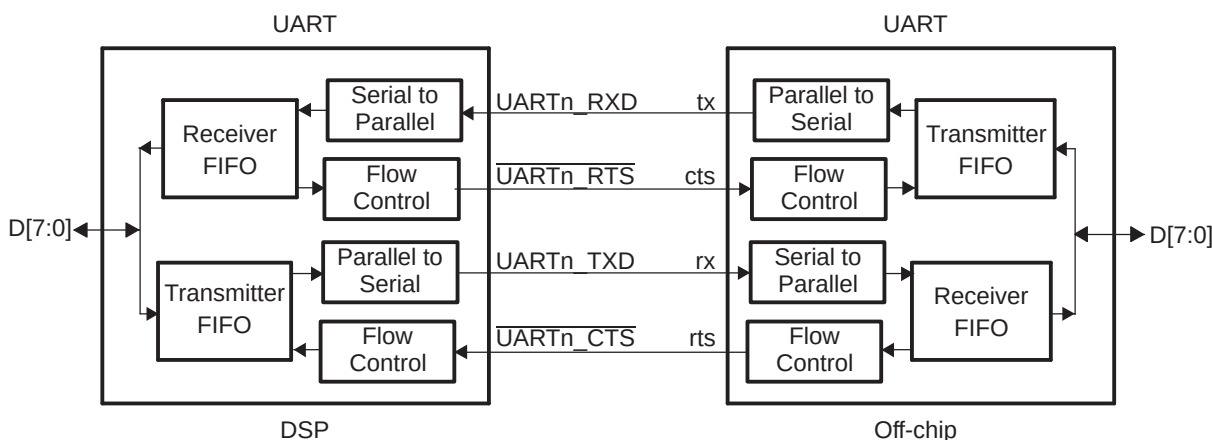
Figure 27-5. UART Interface Using Autoflow Diagram
