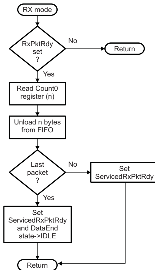
Figure 29-9. RX Mode Flow Chart
