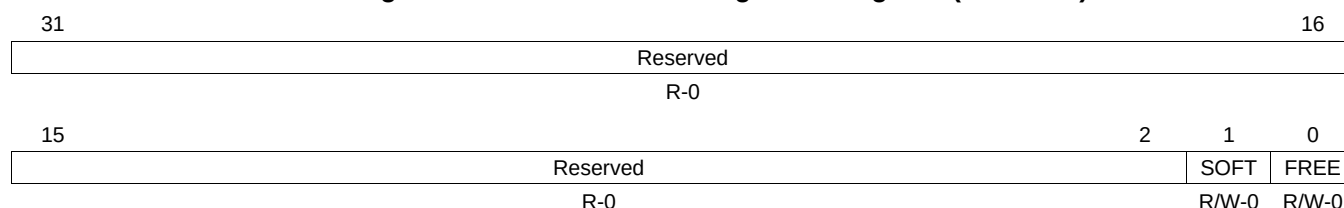
Figure 26-14. Emulation Management Register (EMUMGT)
