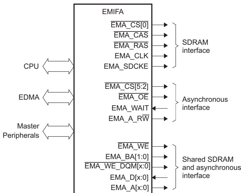
Figure 17-1. EMIFA Functional Block Diagram
