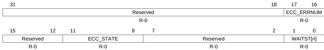
Figure 17-43. NAND Flash Status Register (NANDFSR)
