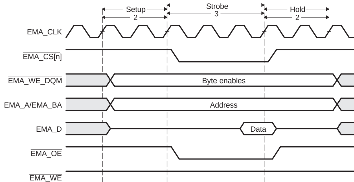
Figure 17-12. Timing Waveform of an Asynchronous Read Cycle in Select Strobe Mode
