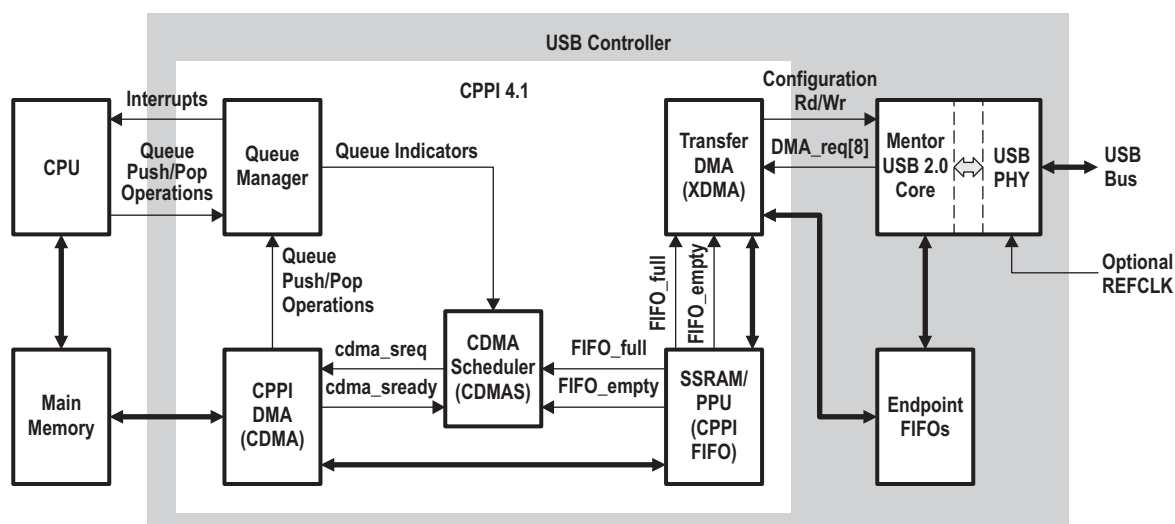
Figure 29-15. USB Controller Block Diagram
