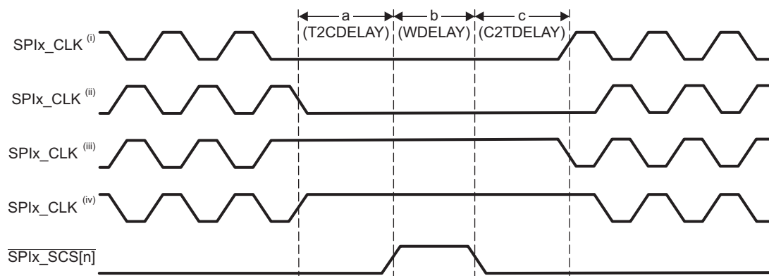
Figure 25-14. SPI 4-Pin with \overline{\text{SPIx\_SCS}}[n] Mode with T2CDELAY, WDELAY, and C2TDELAY
