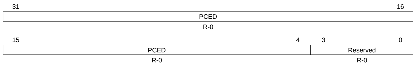
Figure 28-9. HC Current Periodic Register (HCPERIODCURRENTED)
