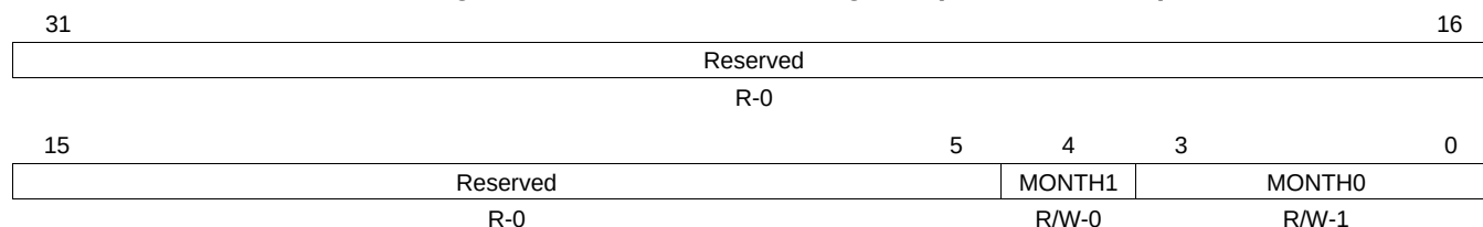
Figure 24-15. Alarm Month Register (ALARMMONTH)
