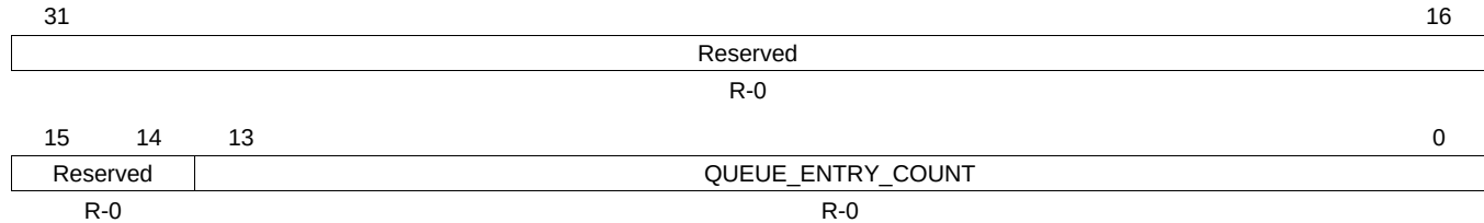
Figure 29-115. Queue Manager Queue N Status Register A (QSTATATA[ N ])
