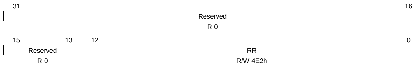
Figure 17-34. SDRAM Refresh Control Register (SDRCR)
