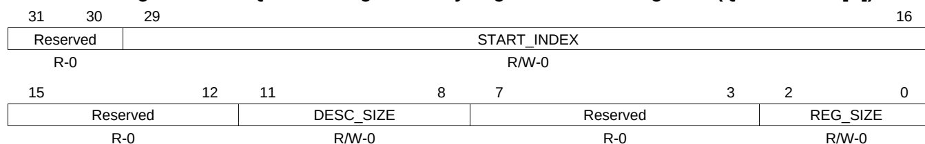
Figure 29-113. Queue Manager Memory Region R Control Registers (QMEMRCTRL[ R ])
