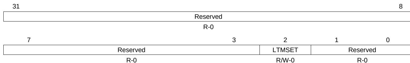
Figure 18-27. Interrupt Mask Set Register (IMSR)
