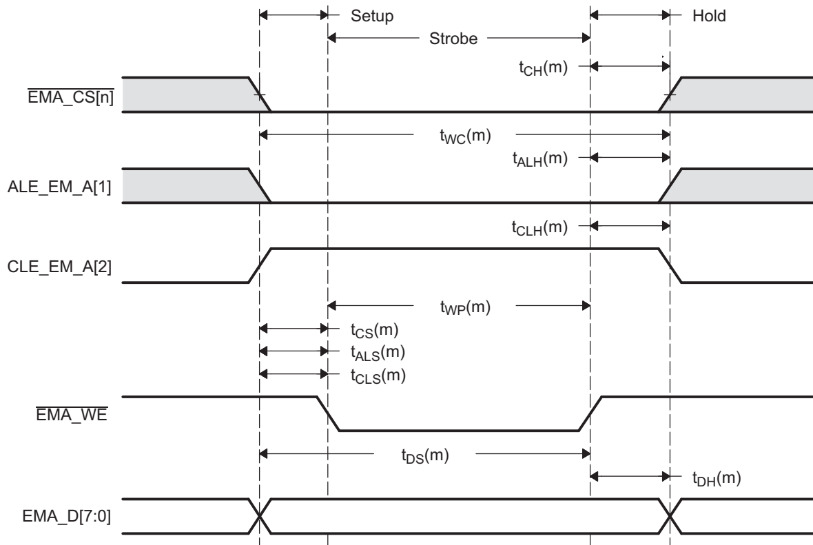
Figure 17-28. Timing Waveform of a NAND Flash Command Write
