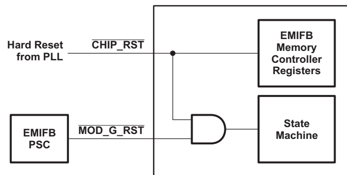
Figure 18-9. EMIFB Memory Controller Reset Block Diagram
