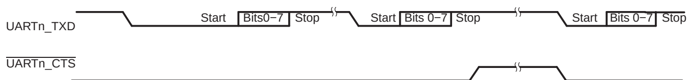
Figure 27-7. Autoflow Functional Timing Waveforms for UARTn_CTS
