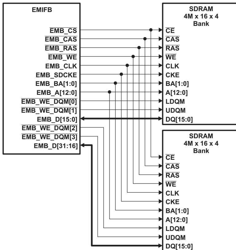
Figure 18-11. Connecting EMIFB Memory Controller for 32-bit Connection
