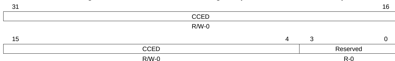
Figure 28-11. HC Current Control Register (HCCONTROLCURRENTED)
