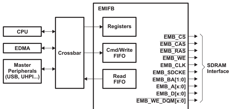
Figure 18-1. EMIFB Functional Block Diagram
