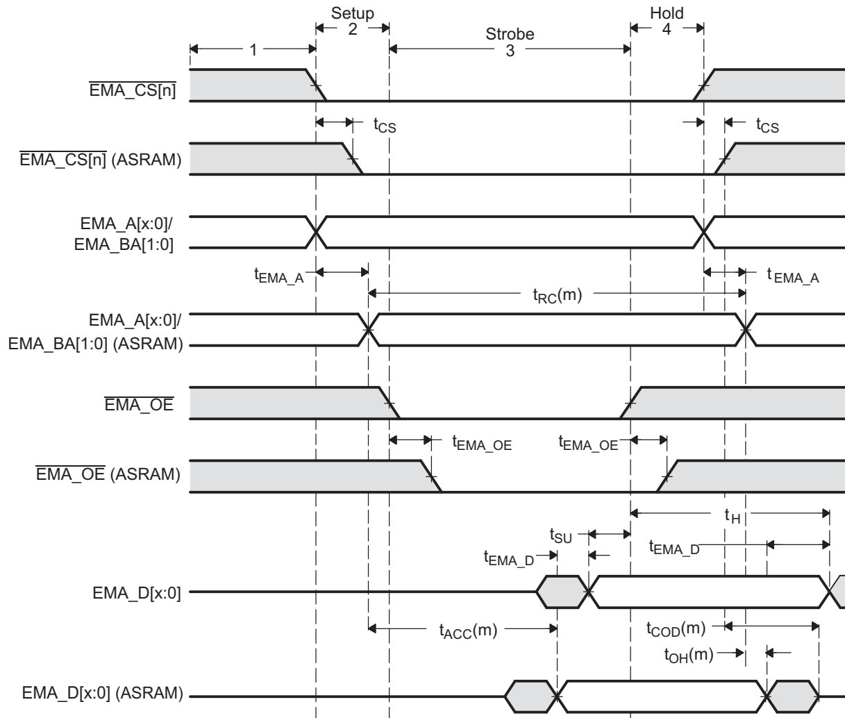
Figure 17-25. Timing Waveform of an ASRAM Read with PCB Delays
