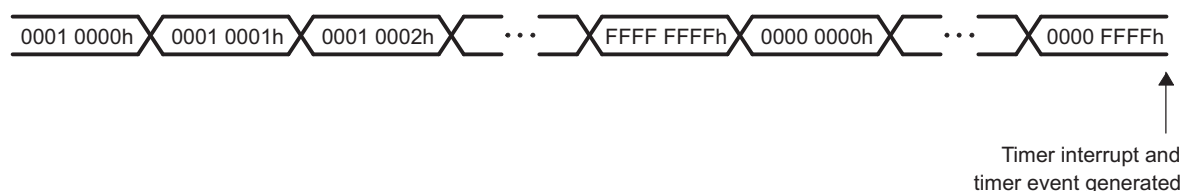
Figure 26-8. 32-Bit Timer Counter Overflow Example
