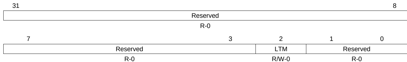
Figure 18-26. Interrupt Mask Register (IMR)
