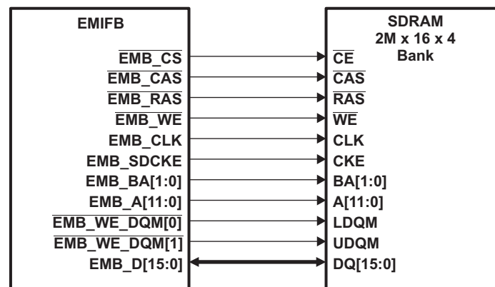
Figure 18-3. EMIFB to 2M × 16 × 4 bank SDRAM Interface
