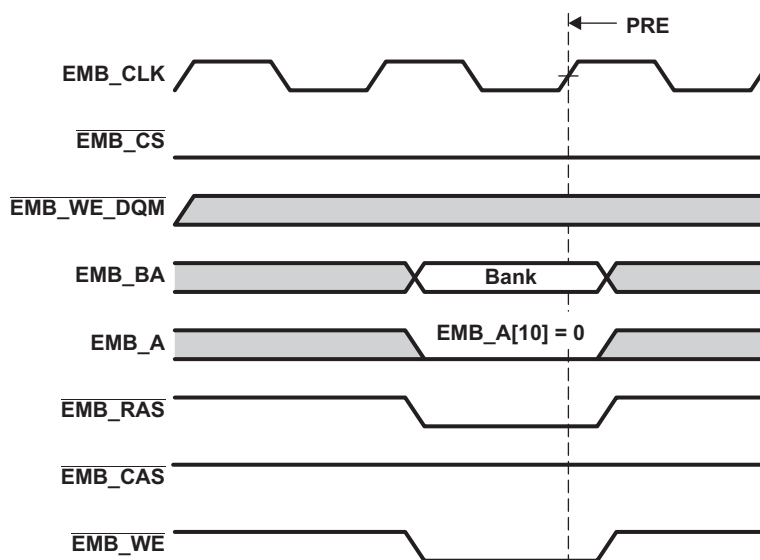
Figure 18-2. Timing Waveform of SDRAM PRE Command
