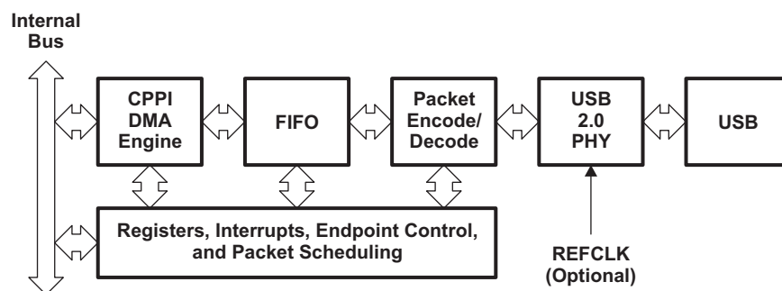
Figure 29-1. Functional Block Diagram
