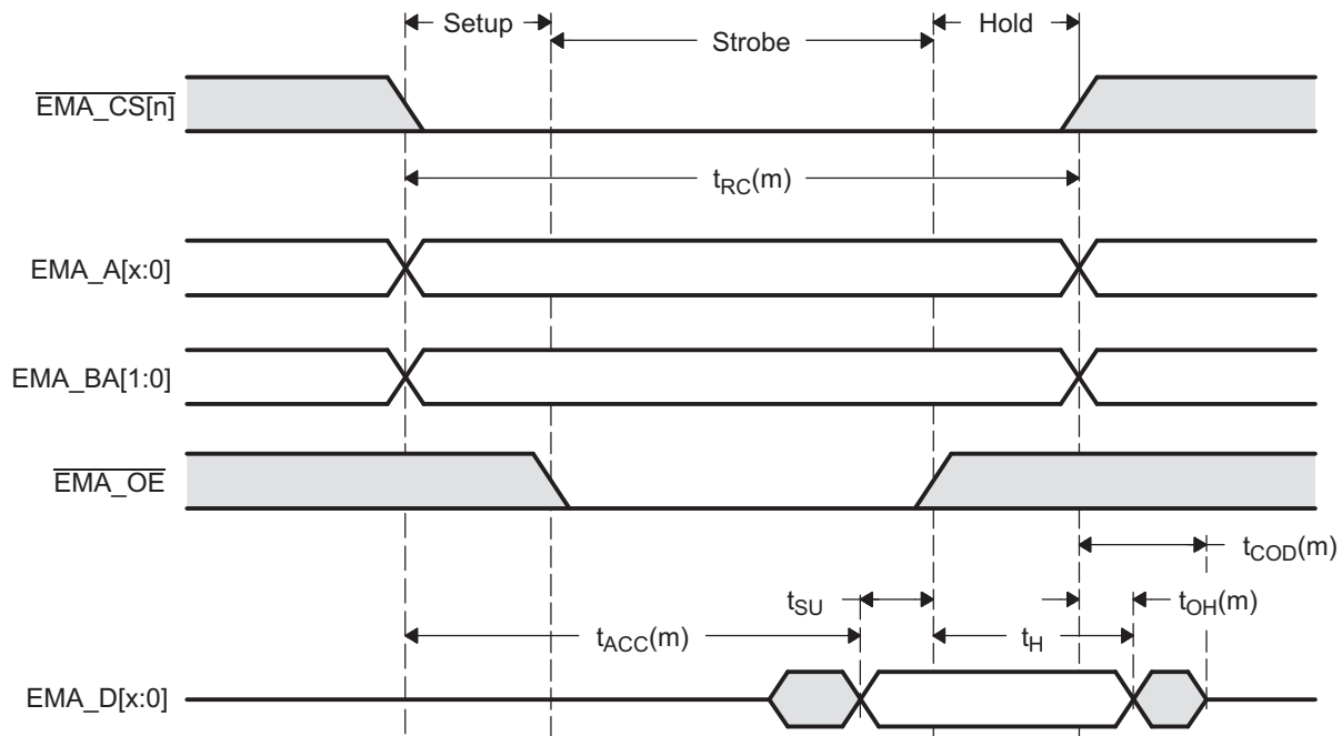
Figure 17-23. Timing Waveform of an ASRAM Read
