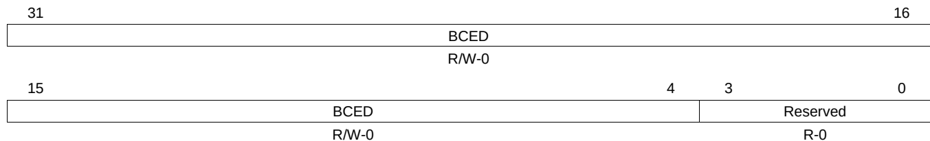
Figure 28-13. HC Current Bulk Register (HCBULKCURRENTED)
