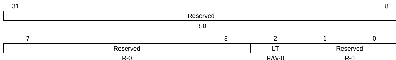
Figure 18-25. Interrupt Raw Register (IRR)
