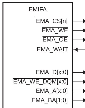
Figure 17-7. EMIFA Asynchronous Interface
