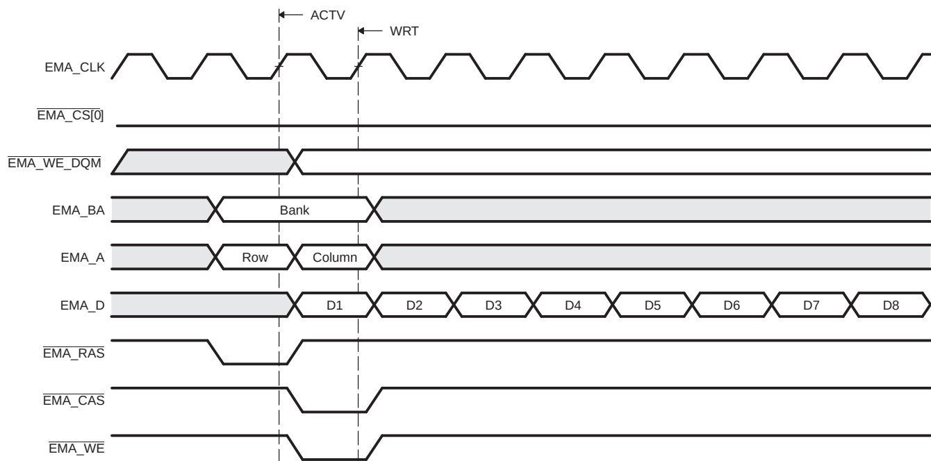
Figure 17-6. Timing Waveform for Basic SDRAM Write Operation
