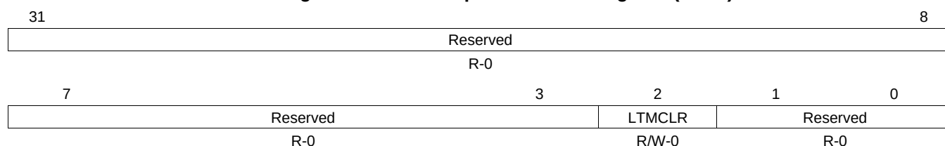
Figure 18-28. Interrupt Mask Clear Register (IMCR)
