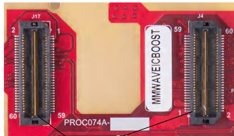
60Pin HD Connector
