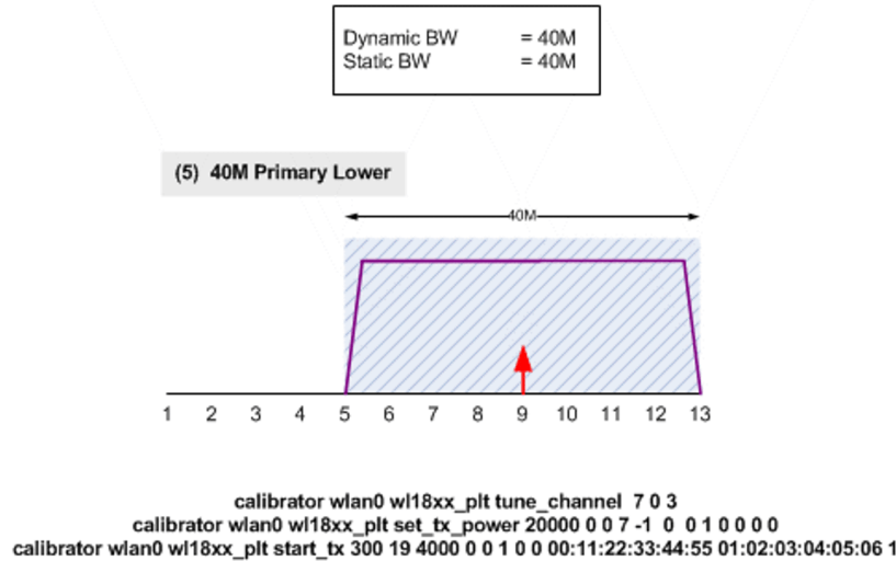
Figure 3-6. Band 2.4 GHz, 40 MHz Primary Lower
