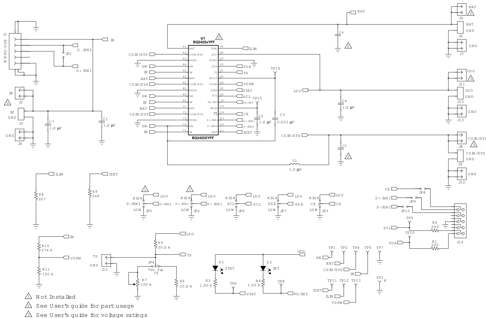
Figure 1. bq2425xEVM-150 Schematic
