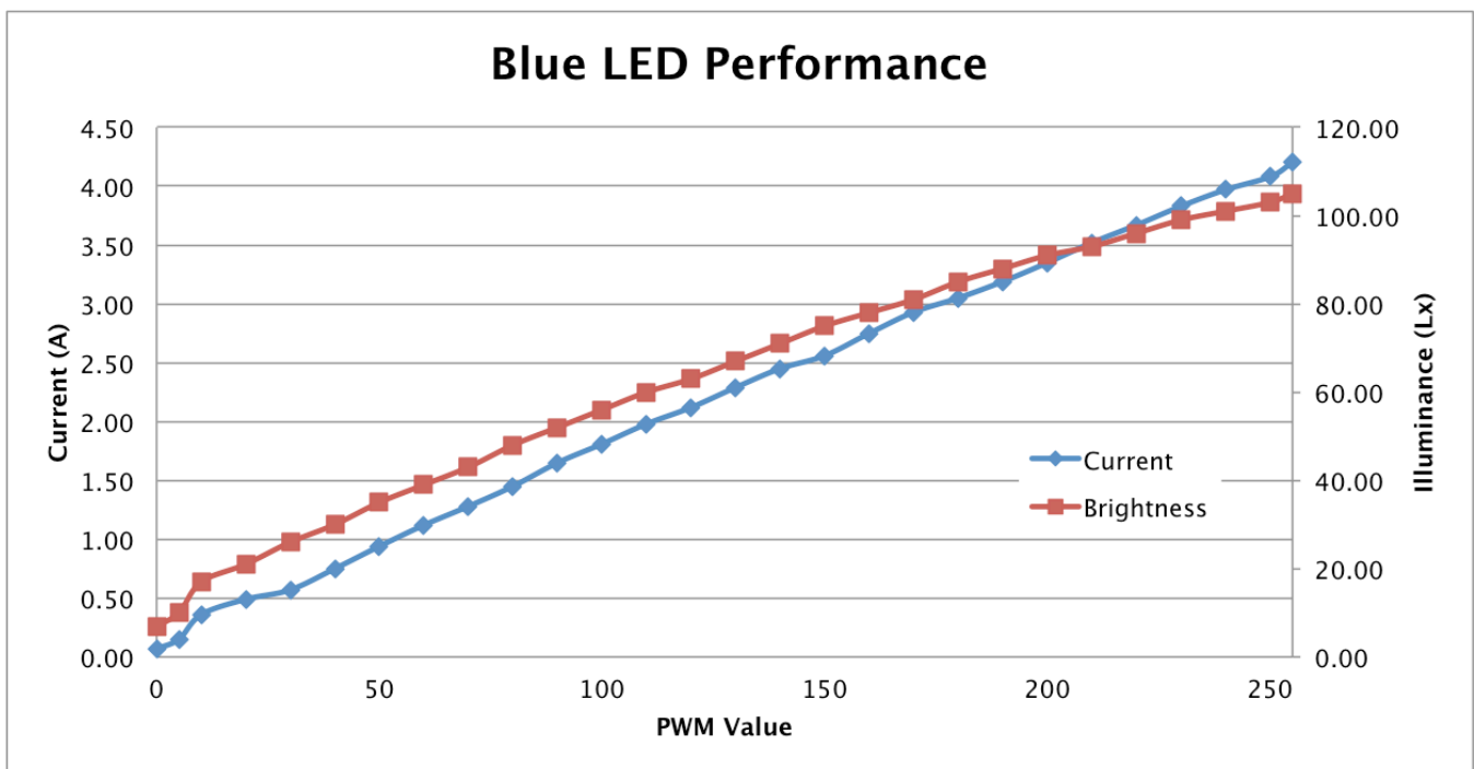
Figure 1-3. Typical Blue LED Current and Illuminance based on PWM values
