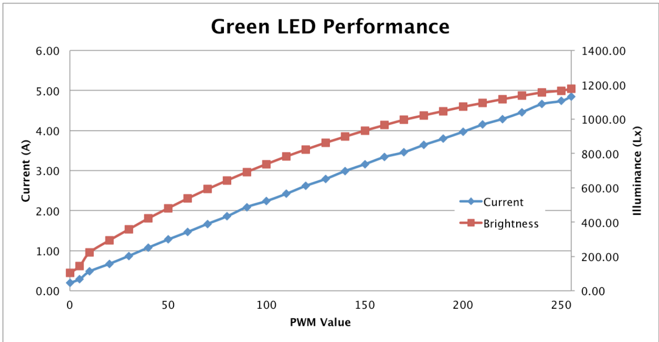
Figure 1-2. Typical Green LED Current and Illuminance based on PWM values
