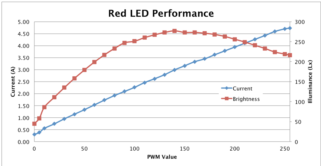
Figure 1-1. Typical Red LED Current and Illuminance based on PWM values
