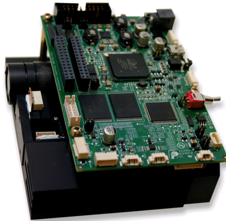
DLP LightCrafter4500 Evaluation Module
