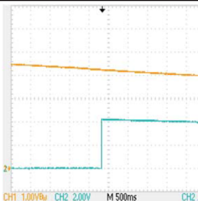
Figure 30. Initial Power Up, COUT
