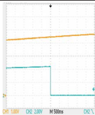
Figure 29. Initial Power Up, DOUT
