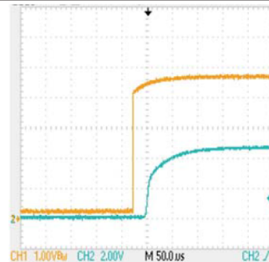
Figure 28. UVP Set Condition
