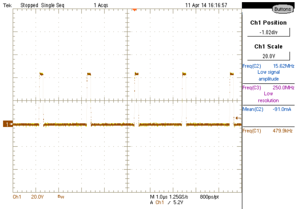
Figure 6, Vin=45V
