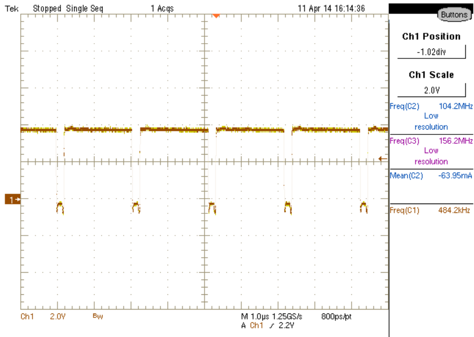
Figure 4 Vin=4.5V
