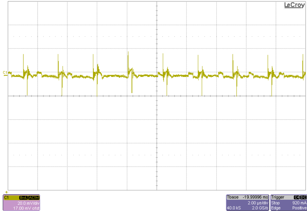
Figure 10. VIN = 12V, VCCINT Output Ripple @ IOU = 3A
