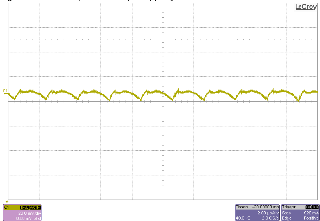
Figure 11. VIN = 12V, VCCAUX Output Ripple @ IOU = 3A
