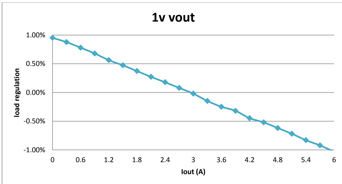
Figure 8. VIN = 12V, VCCINT Load Regulation
