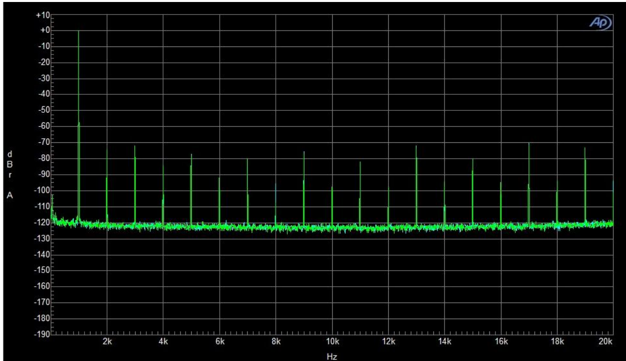
TAS5760 Subwoofer Out FFT 1KHz Fundamental at 1 Watt into 8 ohms
