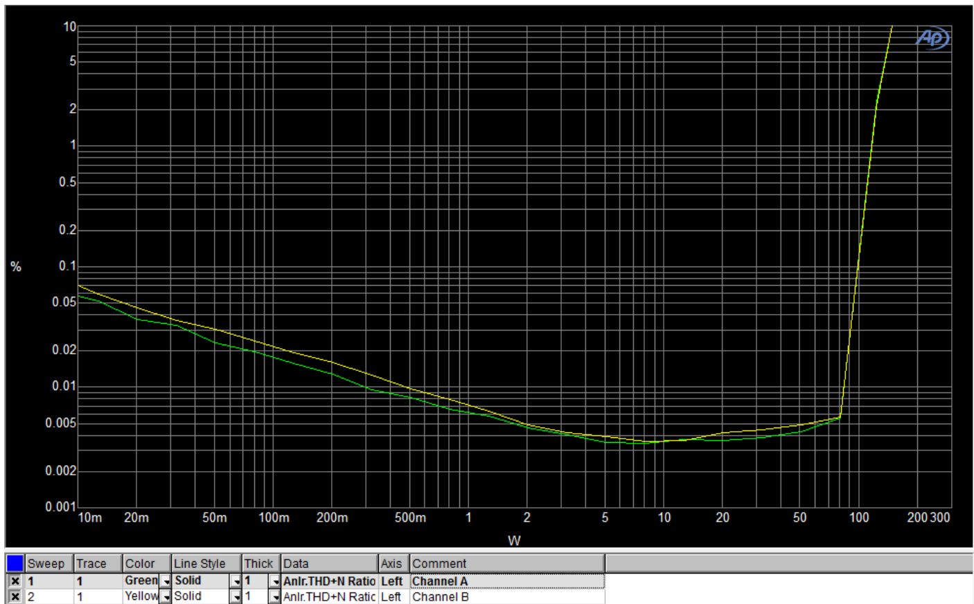
THD + N Vs Output Power 4ohms
