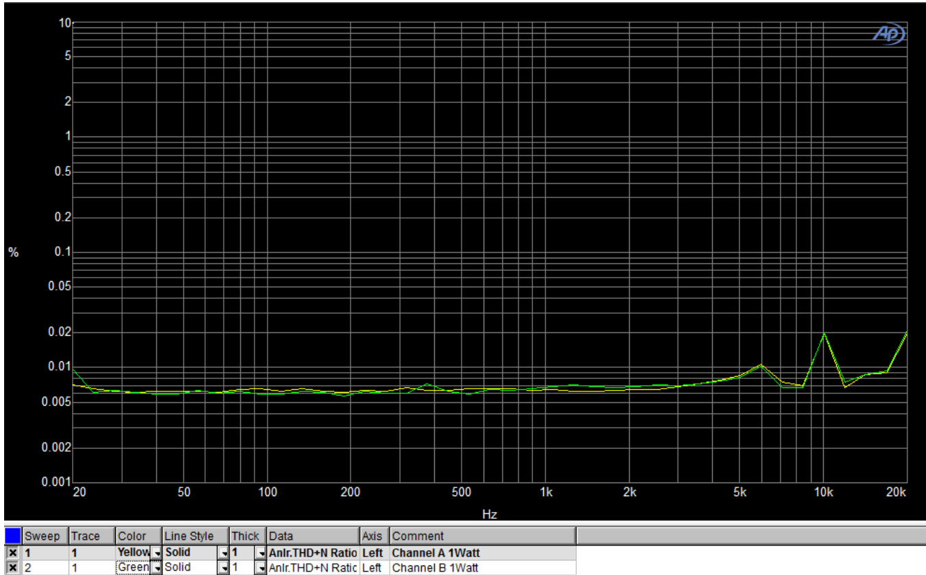
THD + N Vs Frequency @ 1Watt 4ohms
