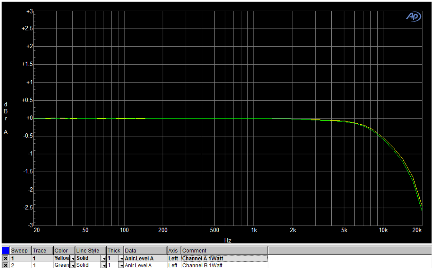
Frequency Response 1W 4ohms (Measurement setup uses 20KHz cutoff)
