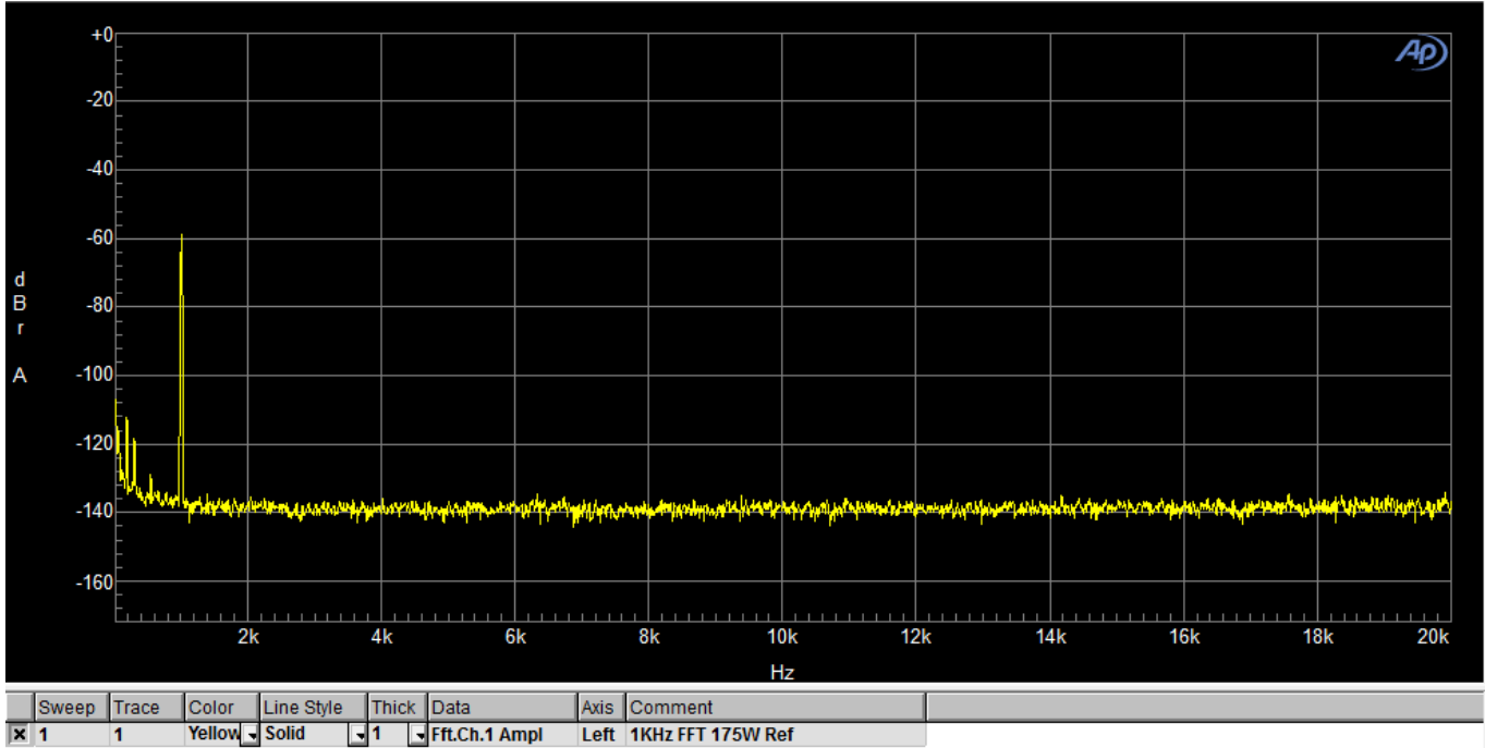
FFT -60dB Reference to 175W (10% THD + N) 4ohms
