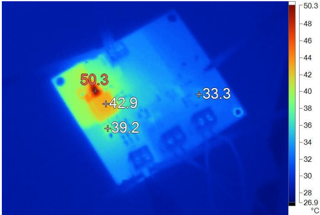
Figure 13: PCB top
