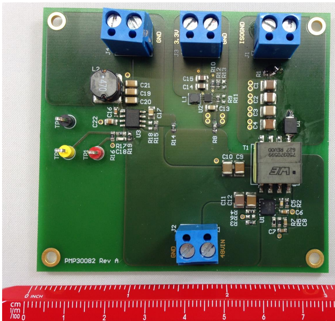
Figure 1: PCB Top
