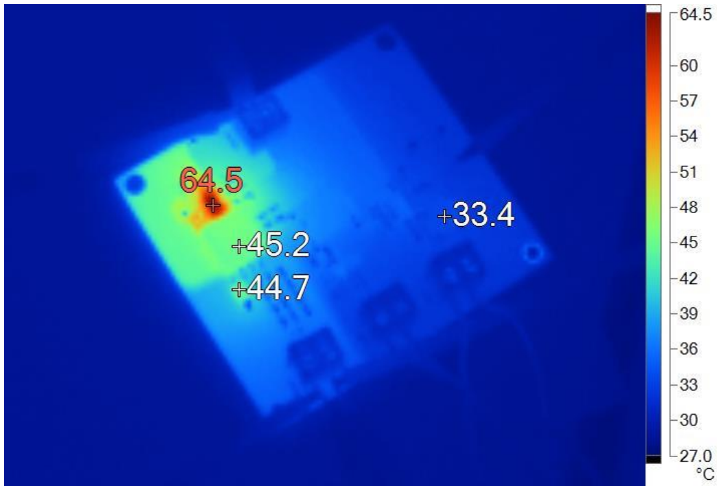
Figure 14: PCB top
