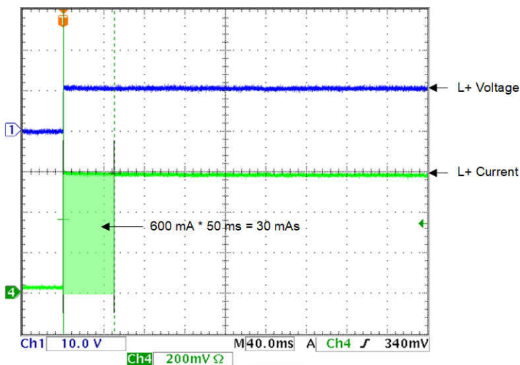
Figure 3-1. TCM_PHYL_INTF_ISIRM with 20 V
