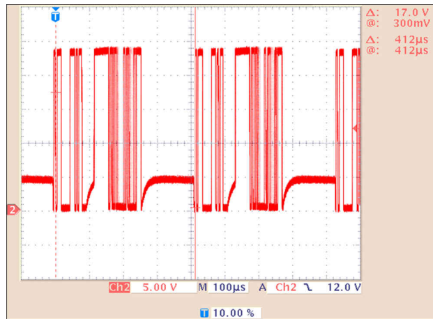
Figure 3-8. CQ Line Communication
