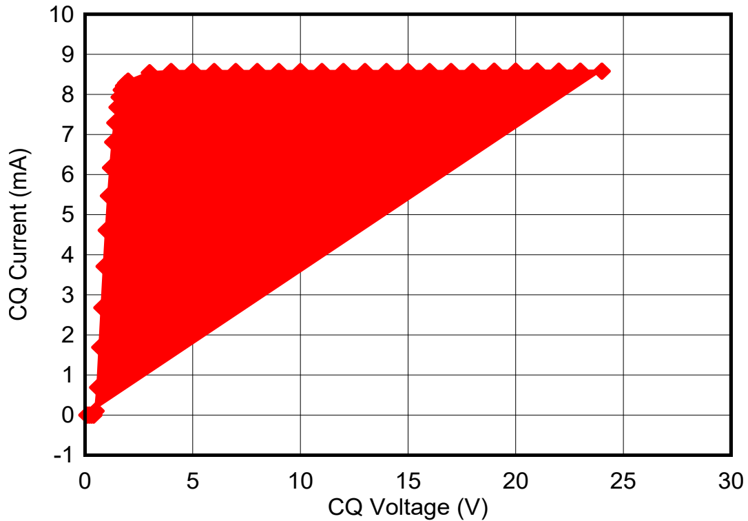
Figure 3-7. Current Sink of TIOL112
