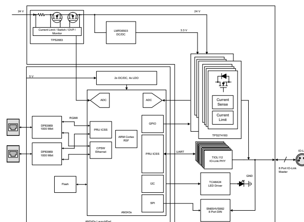
Figure 2-1. TIDA-010234 Block Diagram
