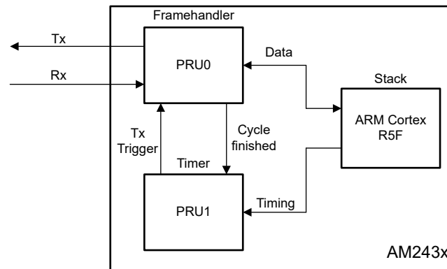
Figure 2-2. Sitara PRU – ARM Relation
