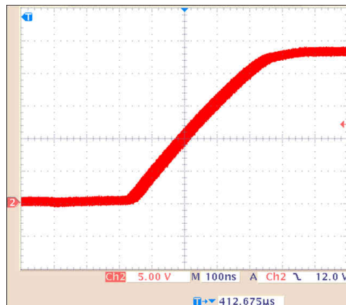
Figure 3-10. Master Cycle Jitter
