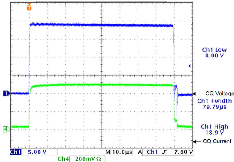
Figure 3-3. TCM_PHYL_INTF_IQWUH with 20 V
