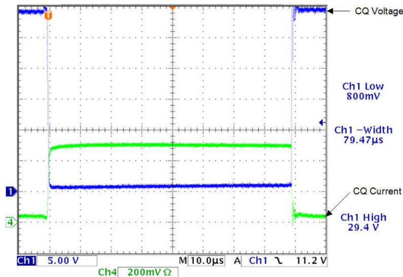
Figure 3-6. TCM_PHYL_INTF_IQWUL with 30 V
