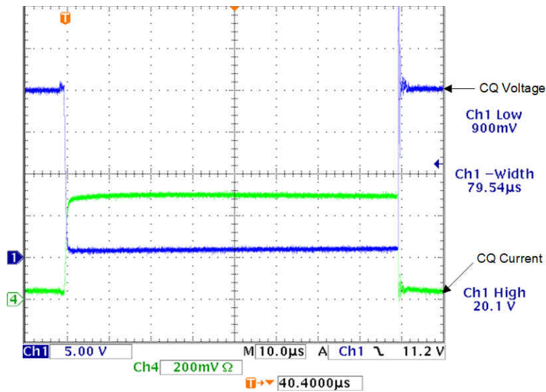
Figure 3-5. TCM_PHYL_INTF_IQWUL with 20 V
