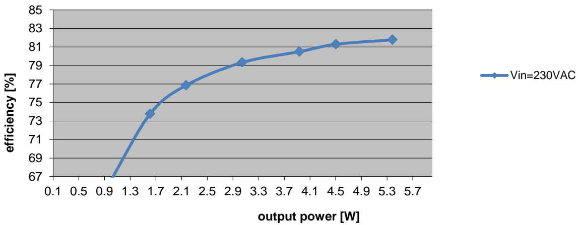
PMP30198 efficiency
