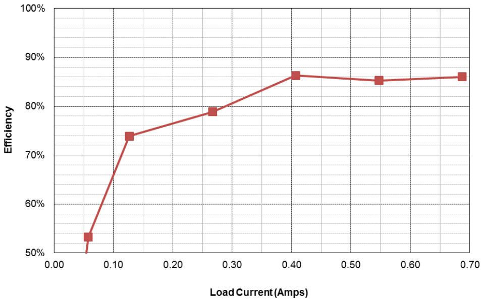
PMP21002 Rev A Efficiency, Mentech TOEP07-0167SG Transformer
