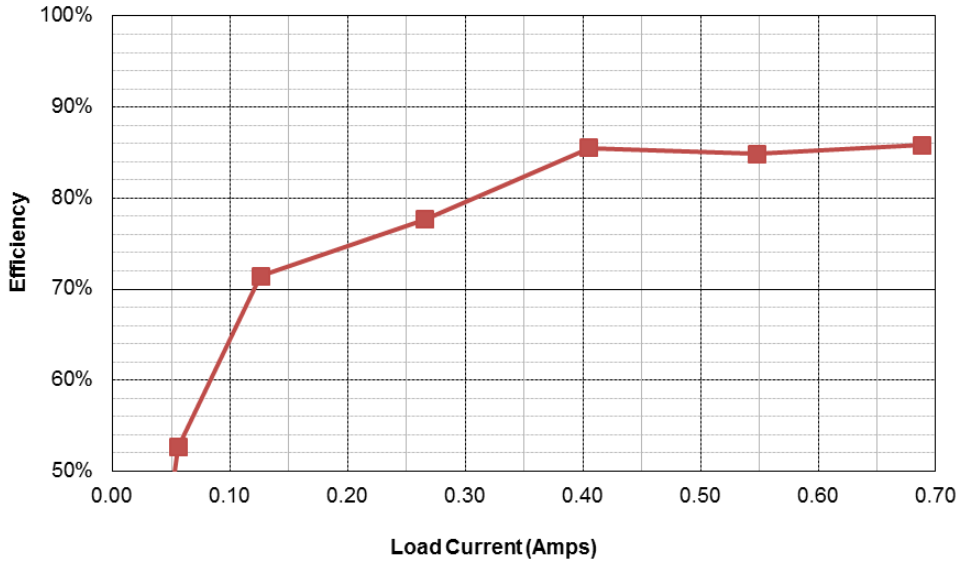
PMP21002 Rev A Efficiency, UMEC UT38806S Transformer
