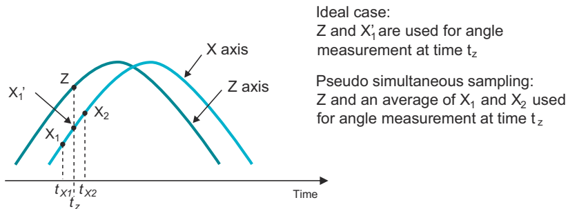
Figure 1-2. XZX Pattern Example of Pseudo-Simultaneous Sampling
