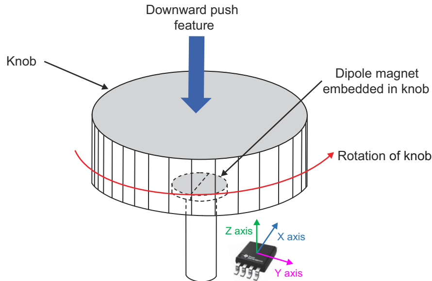
Figure 3-2. Example Out-of-Plane Angle Measurement Using a Linear 3D Hall-Effect Position Sensor in a Knob or Dial Application
