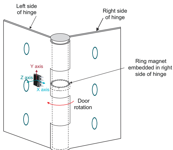
Figure 2-1. Example of Angle Detection in a Traditional Door-Hinge Application
