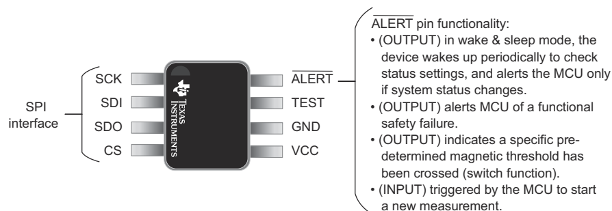
Figure 4-2. TMAG5170 Digital Interface
