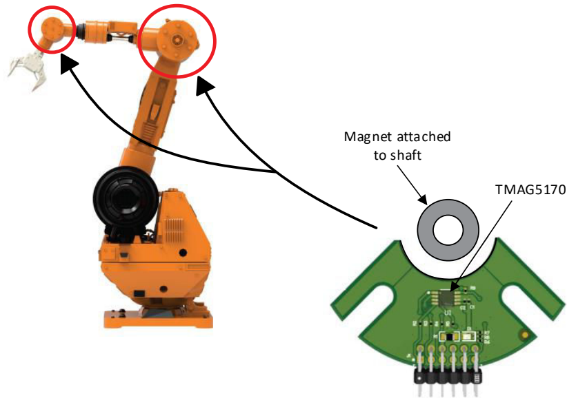
Figure 4-1. Example of a Robotic Arm Using the TMAG5170
