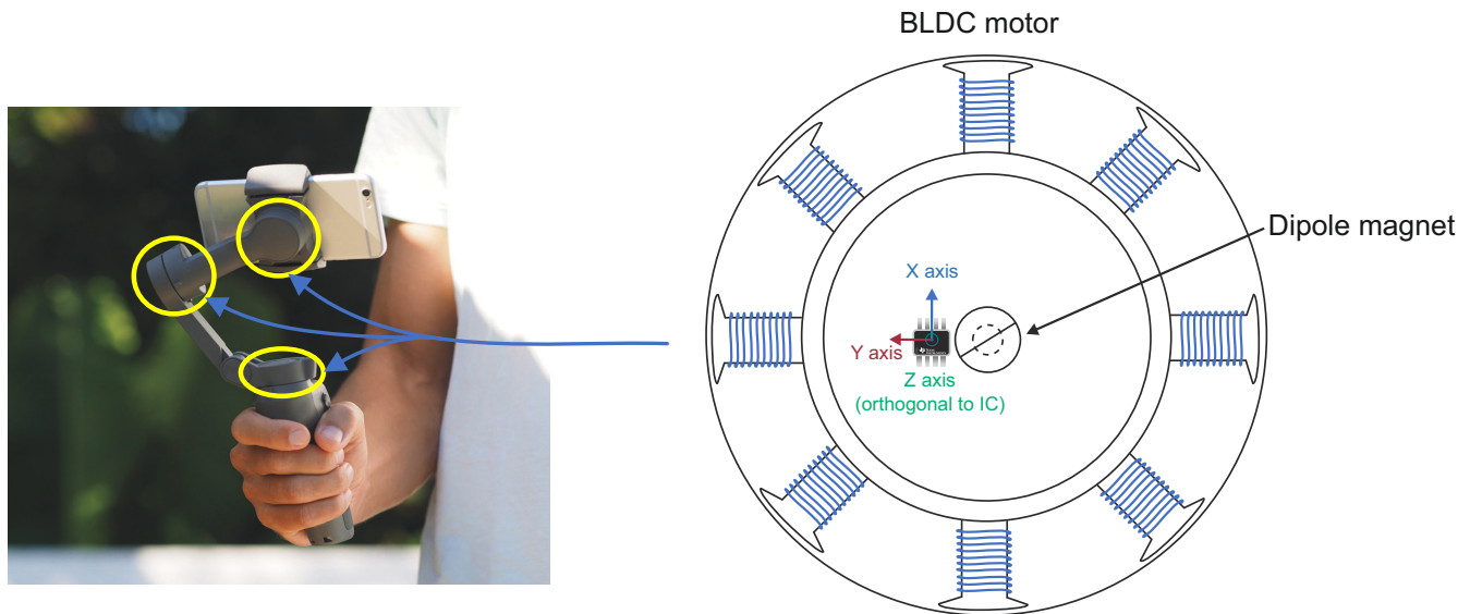
Figure 3-1. Off-Axis Angle Measurement Using 3D Linear in a Handheld Gimbal Motor
