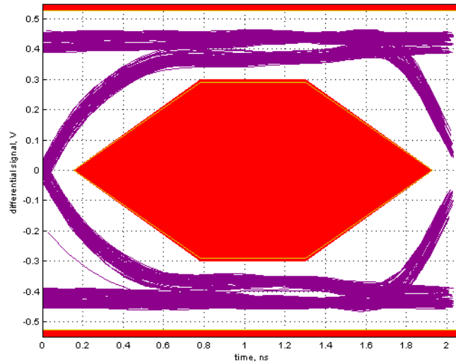
Figure 9. USB 2.0 Eye Diagram through TS3USBCA4 with Compliance Mask in Red
