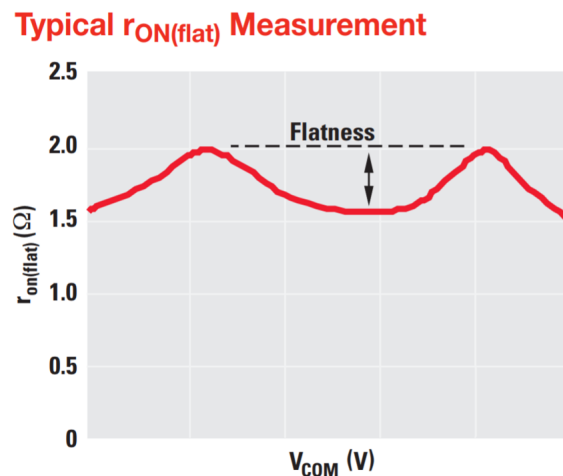
Figure 2. Device R_{on} vs. Signal Voltage
