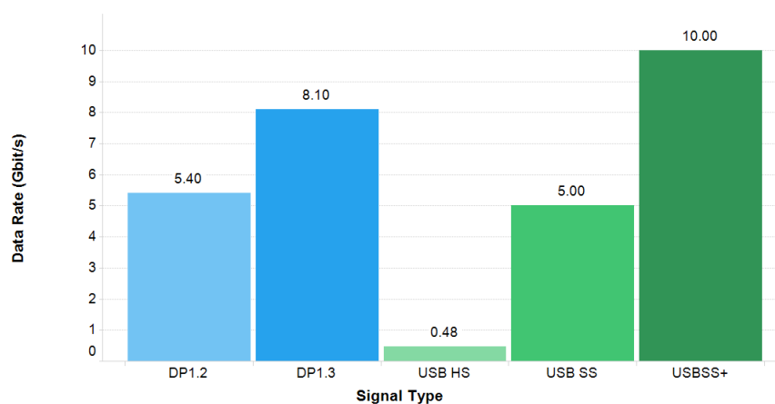
Figure 1. USB-C Signals and Their Associated Data Rates
