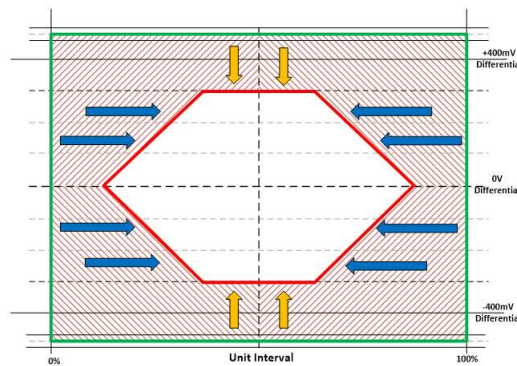
Figure 8. Ideal Eye Diagram with Example Parameters
