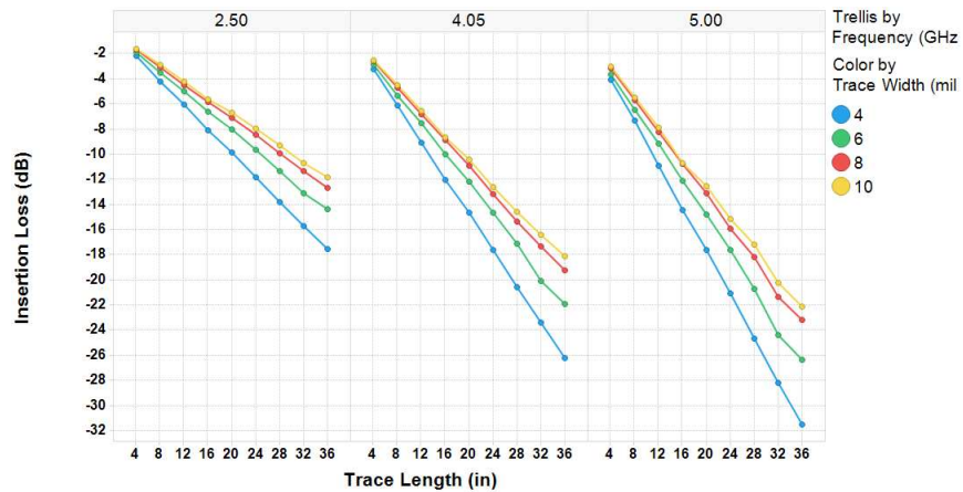
Figure 7. PCB Trace Insertion Loss vs. Signal Frequency
