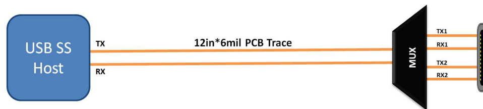
Figure 11. Illustration of a Larger USB System Such as a Laptop or Desktop PC
