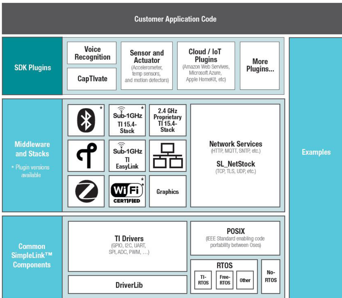
Figure 3. SimpleLink SDK diagram.
