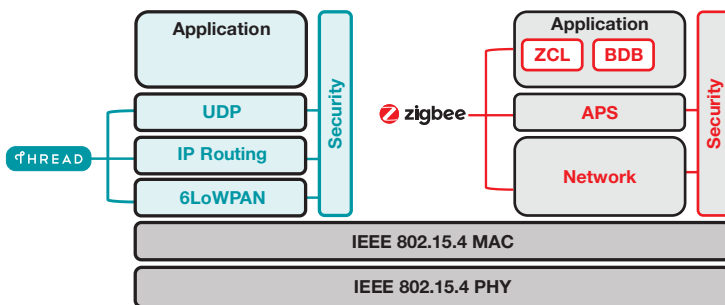
Figure 1. Zigbee and Thread protocol layering.
