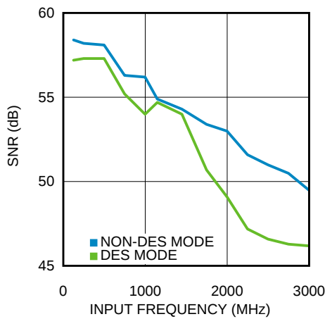
Figure 4-21. SNR vs. Input Frequency (ADC12D1800RF)
