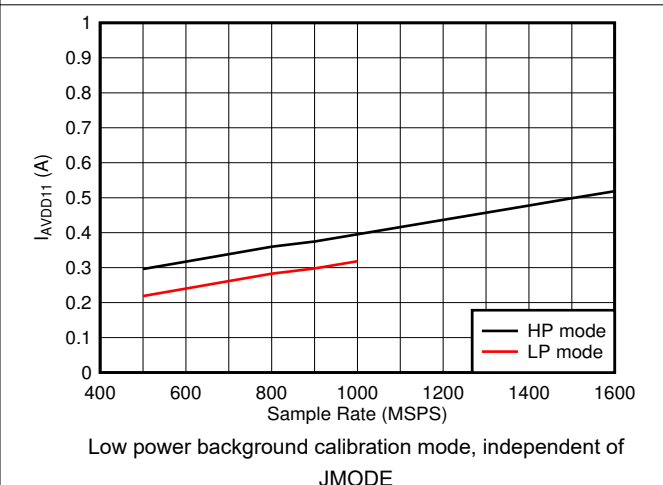
Figure 6-104. Single Channel, I_{VA11} vs F_S
