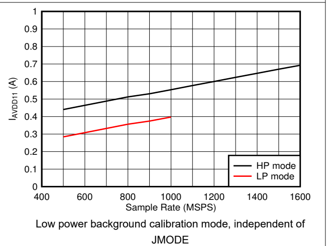
Figure 6-84. Quad Channel, I_{VA11} vs F_S
