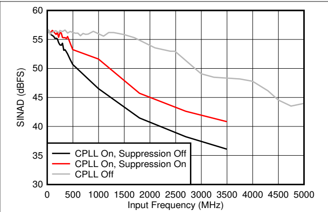
Figure 6-42. SINAD vs F_{IN} and C-PLL modes
