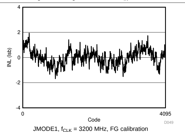
Figure 31. INL vs Code
