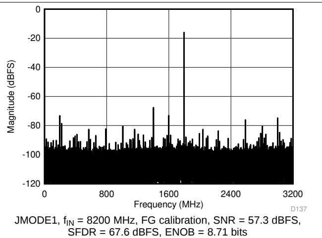
Figure 29. Single-Tone FFT at A_{\text{IN}} = -16\text{ dBFS}
