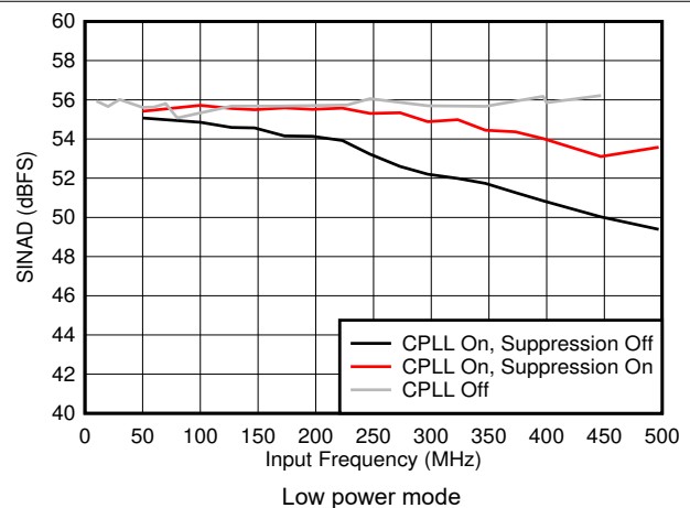
Figure 5-46. SINAD vs F_{IN} and C-PLL modes
