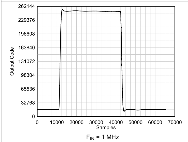
Figure 6-62. Pulse Response
