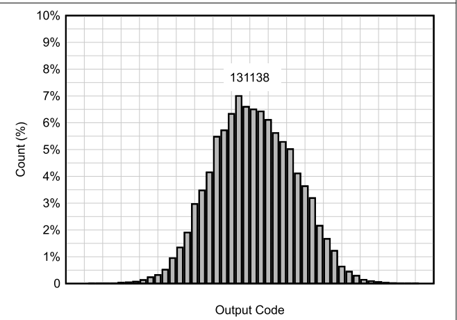
Figure 6-61. DC Histogram
