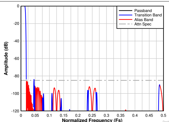
Figure 8-28. Decimation by 32 complex frequency response
