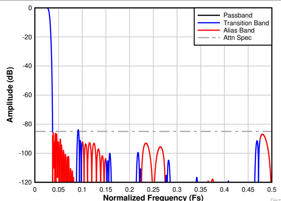
Figure 8-26. Decimation by 16 complex frequency response
