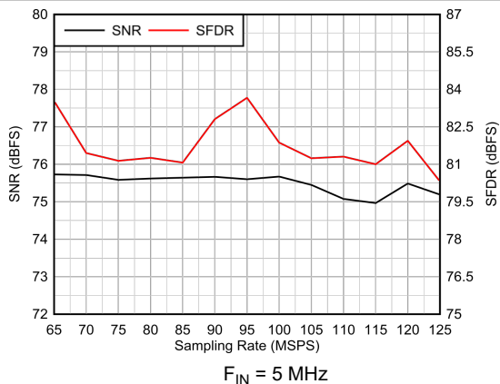
Figure 6-15. AC Performance vs Sampling Rate
