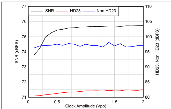
Figure 8-11. AC vs Clock Amplitude F_S = 500\text{MSPS} , F_{IN} = 100\text{MHz} , A_{IN} = -1\text{dBFS}
