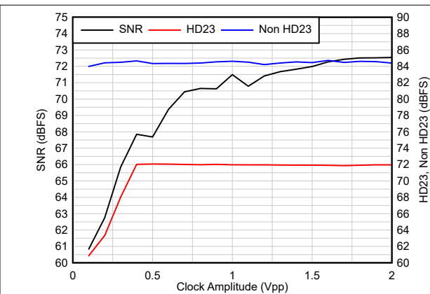
Figure 8-12. AC vs Clock Amplitude F_S = 500\text{MSPS} , F_{IN} = 400\text{MHz} , A_{IN} = -1\text{dBFS}
