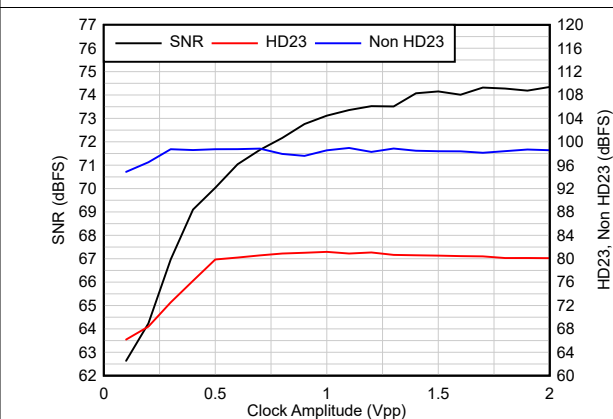
Figure 8-14. AC vs Clock Amplitude F_S = 250\text{MSPS} , F_{IN} = 240\text{MHz} , A_{IN} = -1\text{dBFS}
