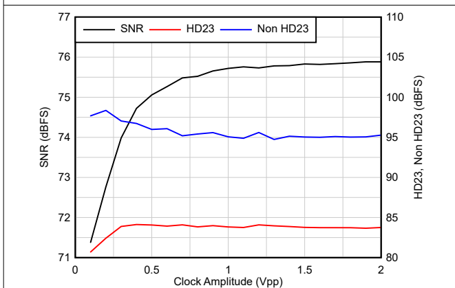
Figure 8-13. AC vs Clock Amplitude F_S = 250\text{MSPS} , F_{IN} = 100\text{MHz} , A_{IN} = -1\text{dBFS}
