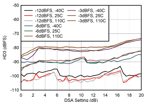
Figure 5-49. HD3 vs DSA Setting at 400 MHz
