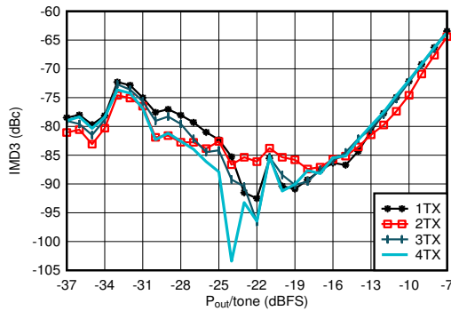
Figure 5-337. TX IMD3 vs Digital Level at 0.85 GHz
