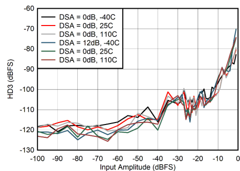
Figure 5-48. HD3 vs Input Amplitude at 400 MHz
