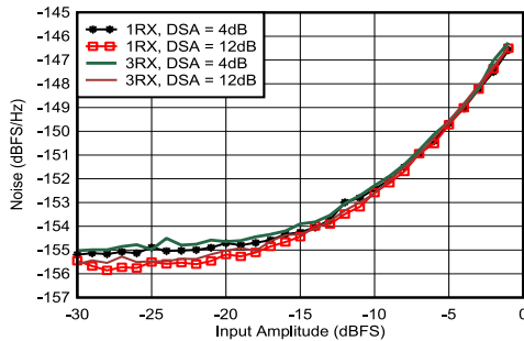
Figure 4-330. RX Noise Spectral Density vs Input Amplitude and Channel at 1.75 GHz
