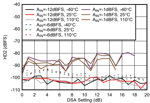
Figure 4-436. RX HD2 vs DSA Setting at 8.1GHz
