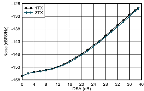
Figure 4-168. TX Output Noise vs Channel and Attenuation at 2.6 GHz
