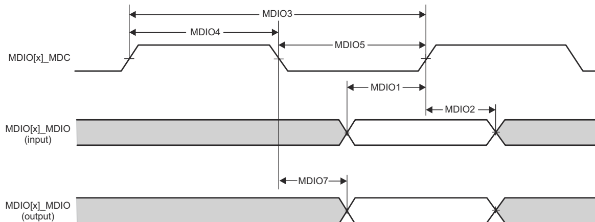
Figure 6-10. CPSW MDIO Timing Requirements and Switching Characteristics
