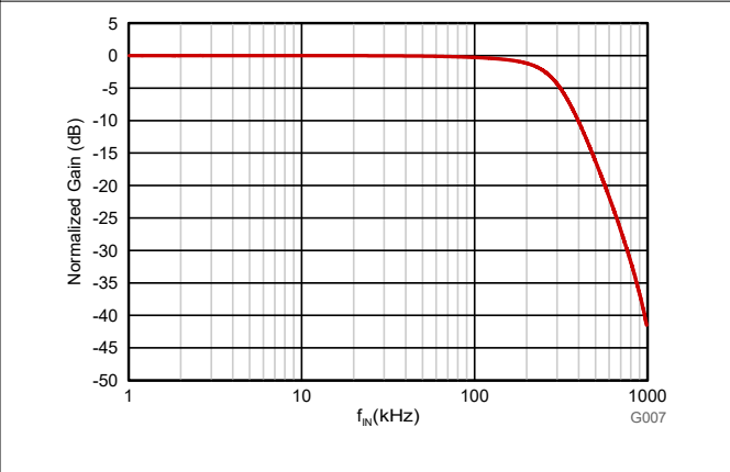
Figure 6-21. Normalized Gain vs Input Frequency
