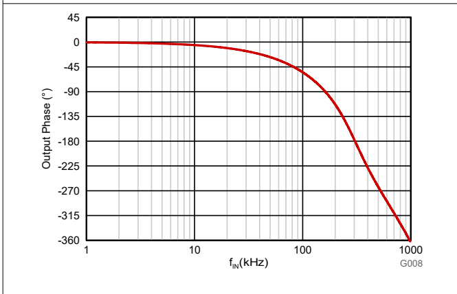
Figure 6-22. Output Phase vs Input Frequency
