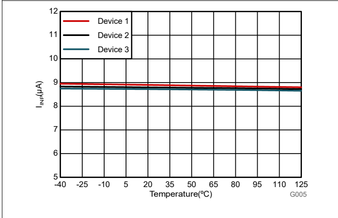
Figure 6-20. Input Current vs Temperature
