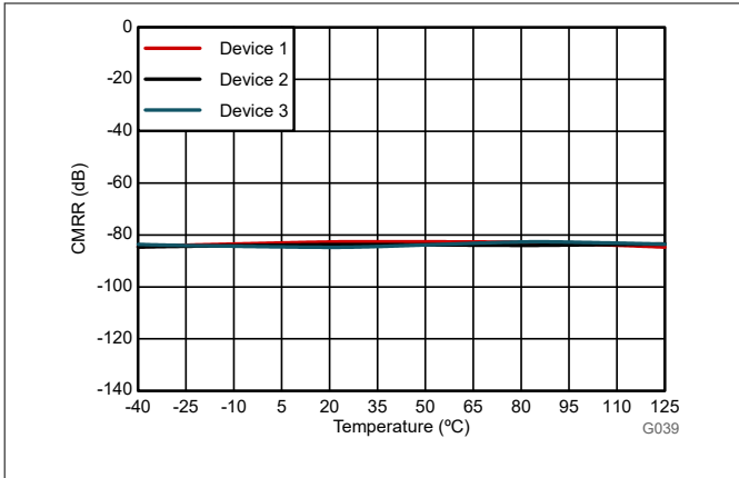
Figure 6-18. Common-Mode Rejection Ratio vs Temperature
