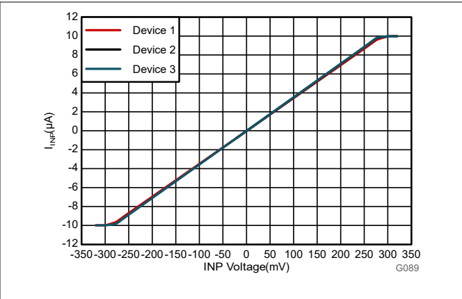
Figure 6-19. Input Current vs Input Voltage
