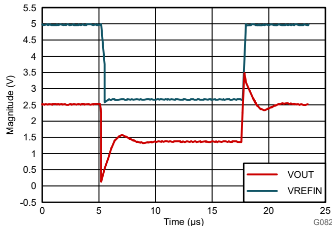
Figure 8-5. Reference Input Step Response of the AMC0x00R
