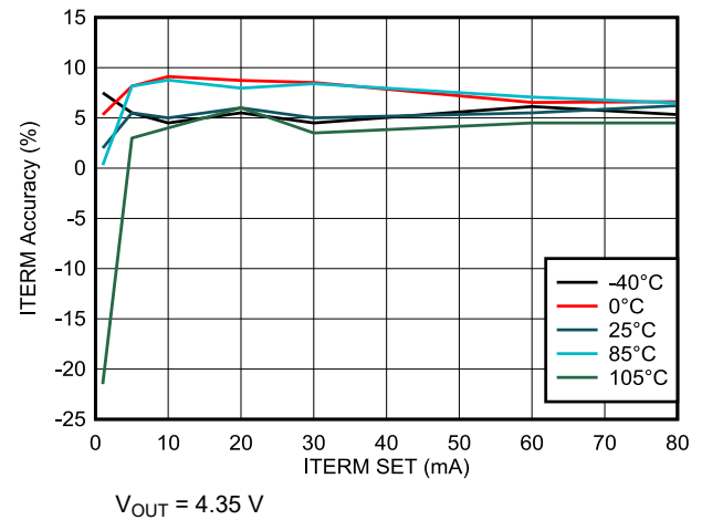
Figure 6-10. Termination Current Accuracy vs Termination Current Setting
