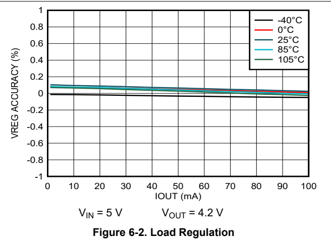
Figure 6-2. Load Regulation
