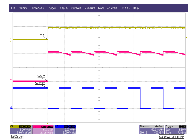
R_{ISET} = 500 \Omega OUT = open-circuit Figure 8-3. Power Up Without Battery
