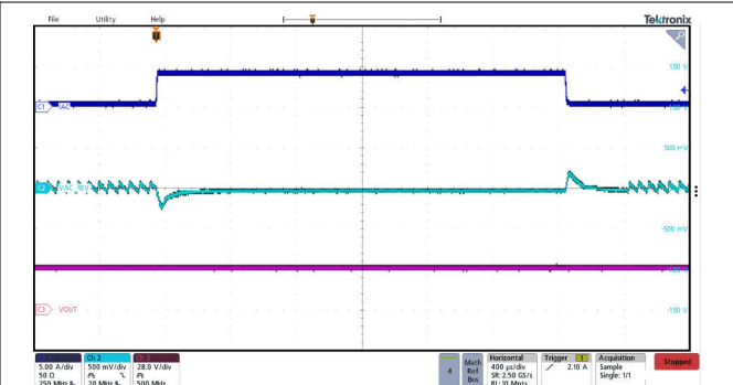
Figure 9-16. Reverse Mode Buck Transient Reponse
