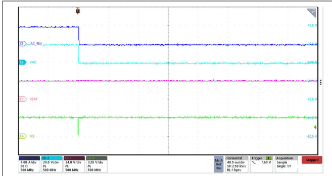
Figure 9-15. Reverse Mode Power Down with 4-A Load
