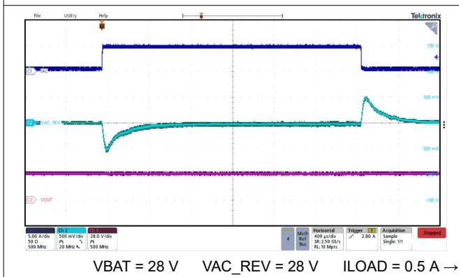
Figure 9-17. Reverse Mode Buck-Boost Transient Reponse
