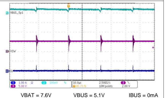
Figure 85. Buck Mode (OTG) PFM Switching
