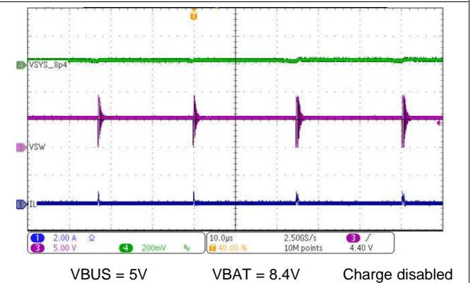
Figure 87. Boost Mode PFM Switching
