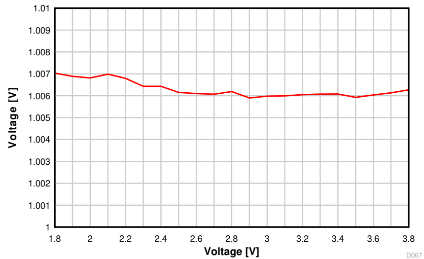
Figure 8-63. ADC Accuracy vs. Supply Voltage (V DD S)
