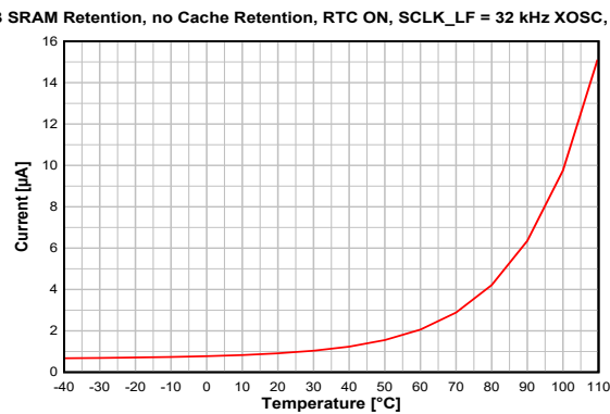
Figure 8-5. Standby Mode (MCU) Current vs. Temperature (VDD5 = 3.6 V)
