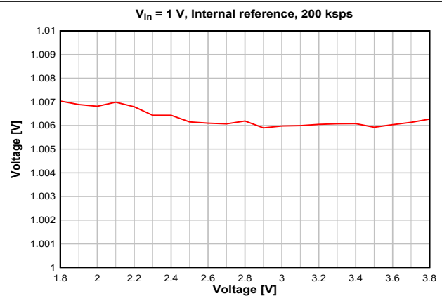
Figure 8-40. ADC Accuracy vs. Supply Voltage (VDD)
